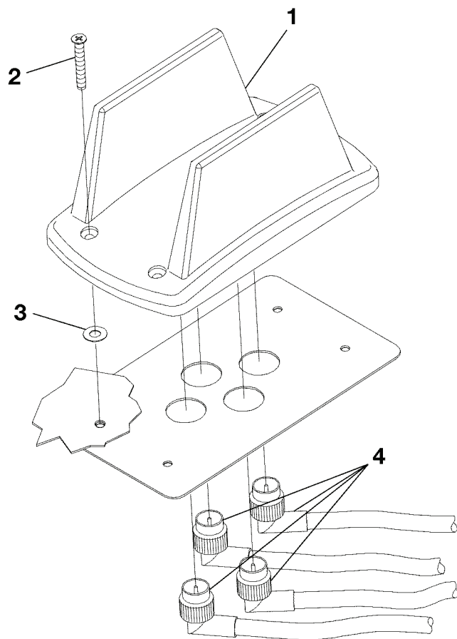
DETAIL A
