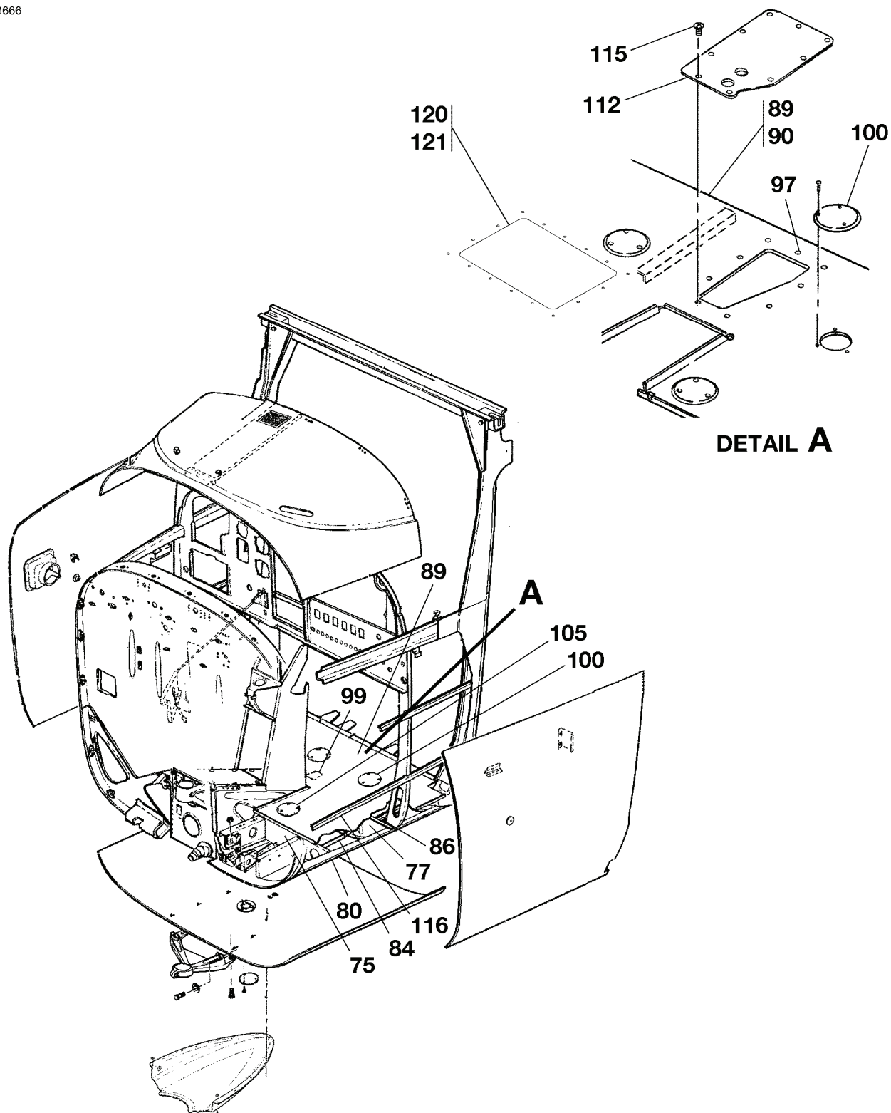
FORWARD FUSELAGE ASSEMBLY FIGURE 01 (SHEET 2)
