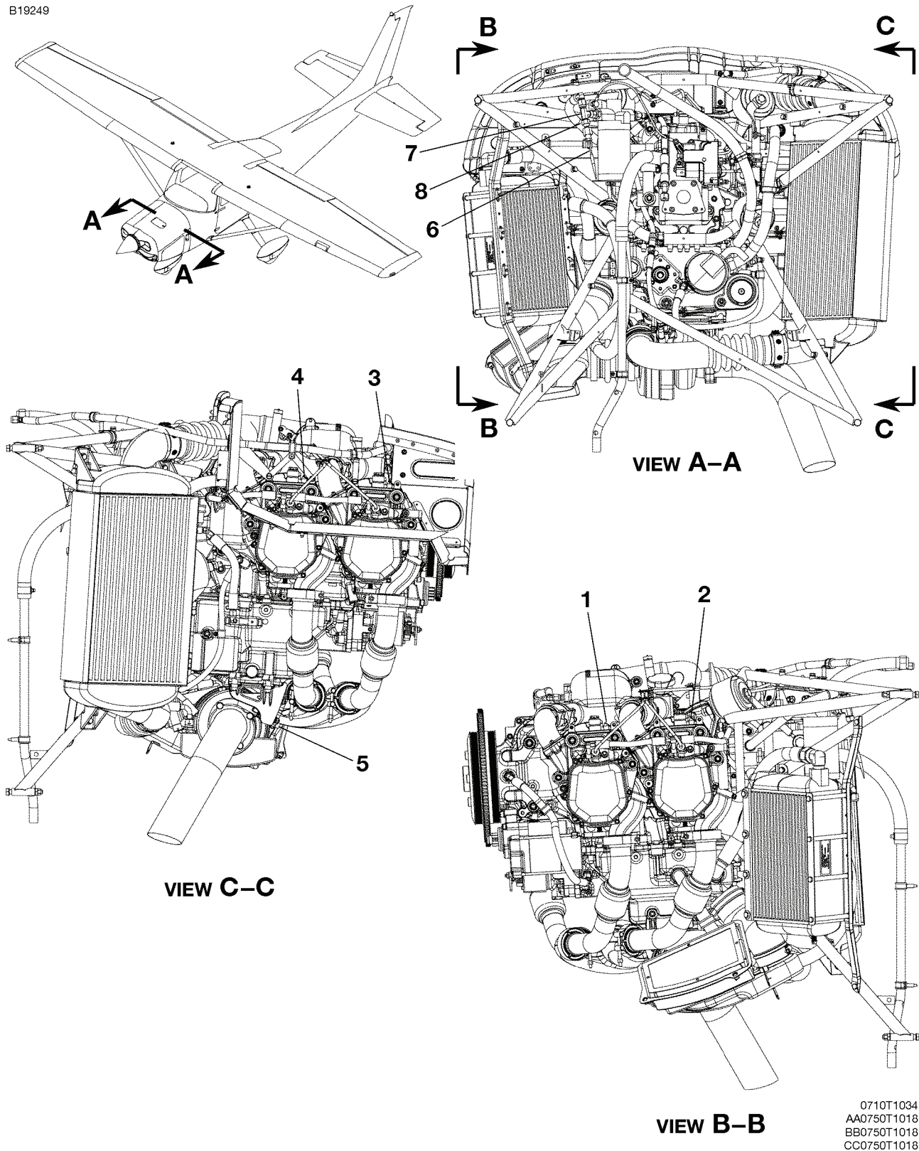
EXHAUST INDICATING SYSTEM - J182T FIGURE 02 (SHEET 1)
