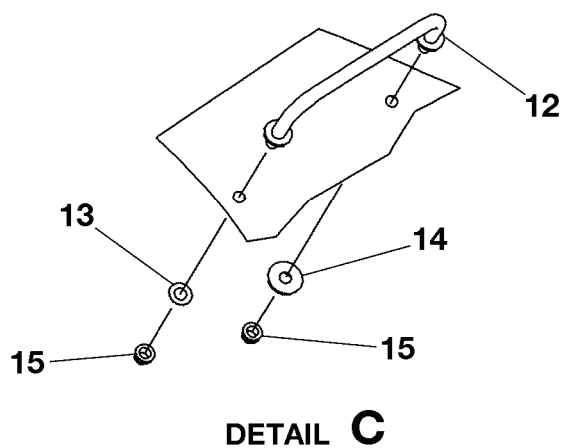
STEP AND HANDLE INSTALLATION-REFUELING FIGURE 01 (SHEET 1)
