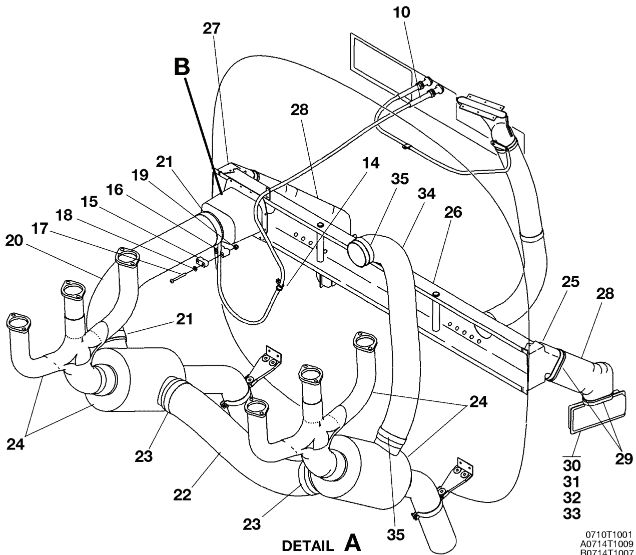
CABIN HEATING AND DEFROSTING INSTALLATION FIGURE 01 (SHEET 1)
