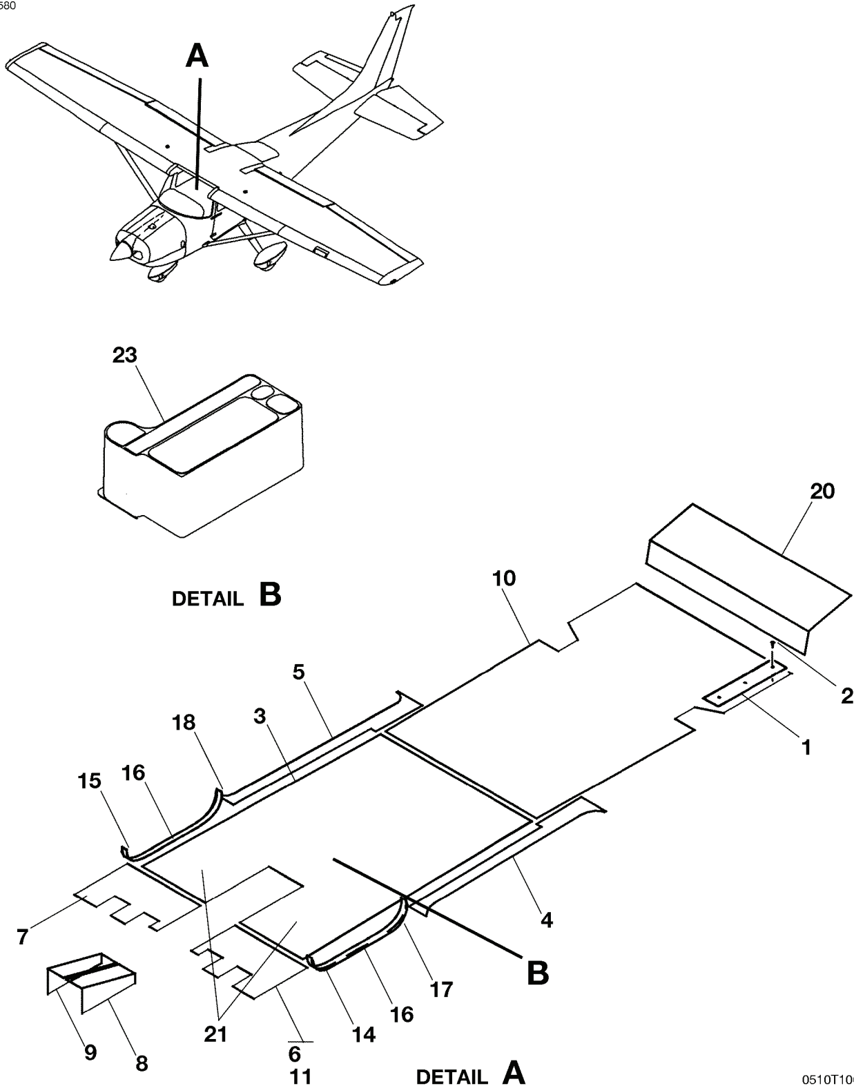
CARPET INSTALLATION - CABIN FIGURE 01 (SHEET 1)
