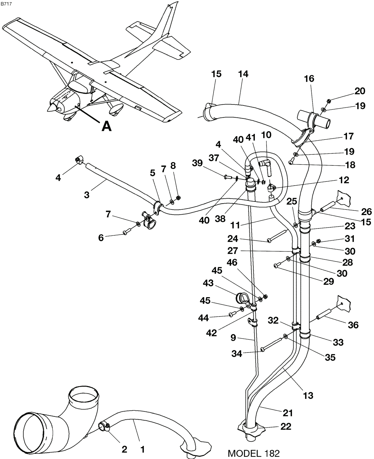
ENGINE DRAIN LINES INSTALLATION - 182 FIGURE 01 (SHEET 1)
