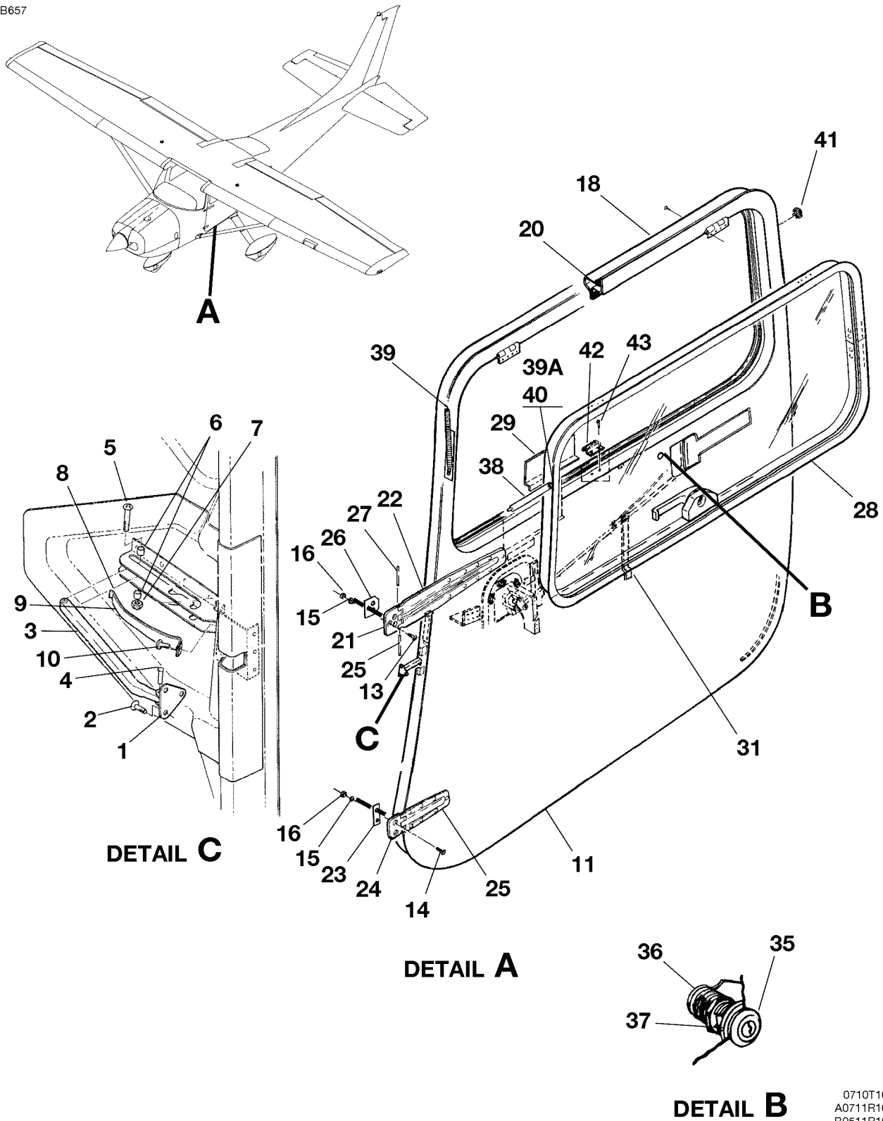
CABIN DOOR INSTALLATION - LH FIGURE 01 (SHEET 1)
