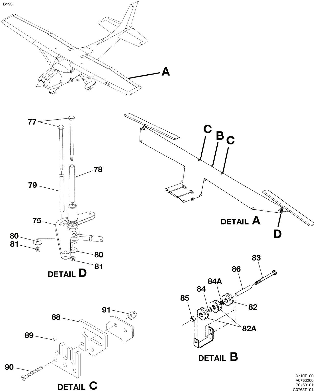
AILERON CONTROL SYSTEM INSTALLATION FIGURE 03 (SHEET 2)
