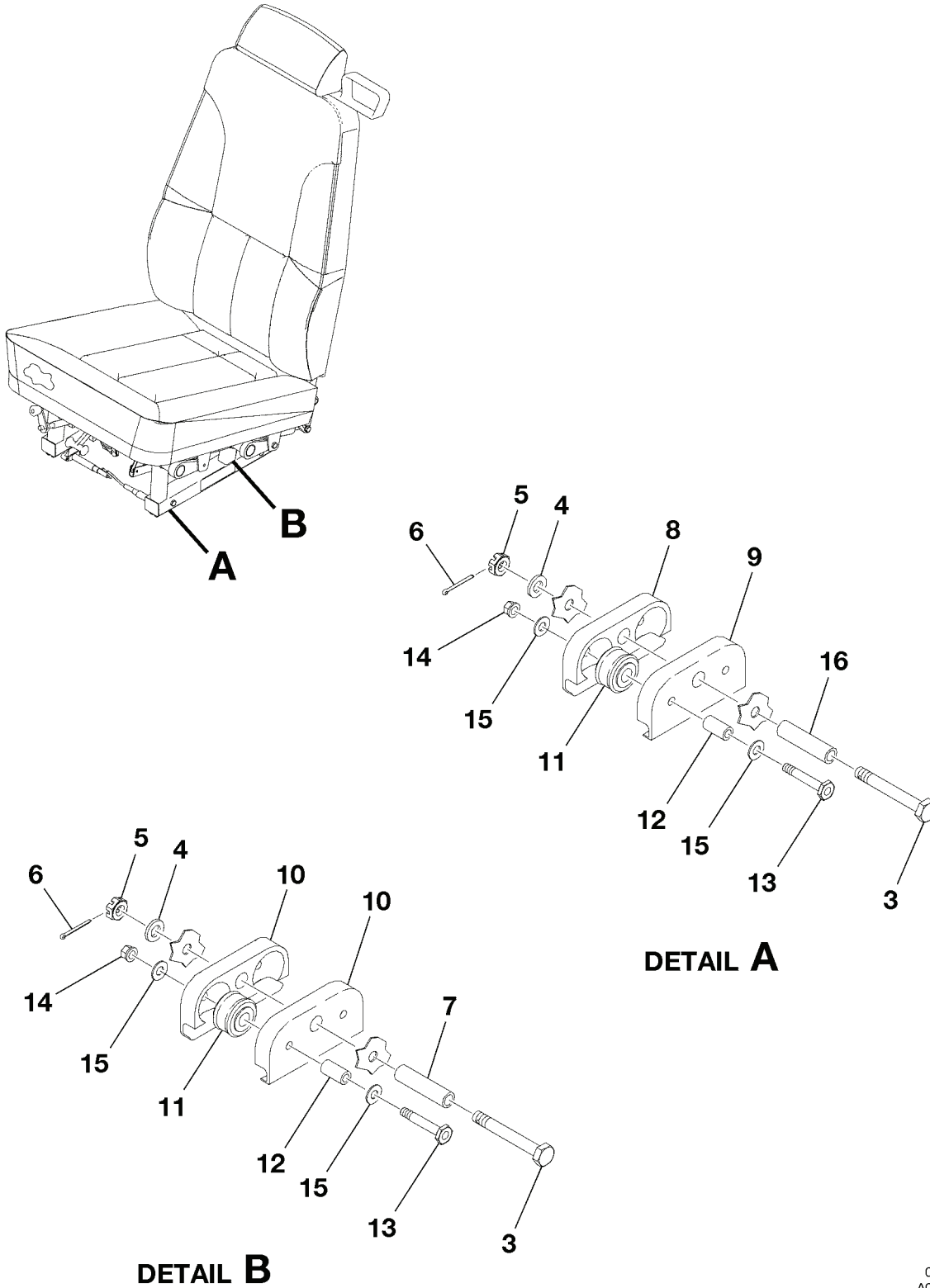
SEAT FOOT ASSY-PILOT AND COPILOT FIGURE 03 (SHEET 1)
