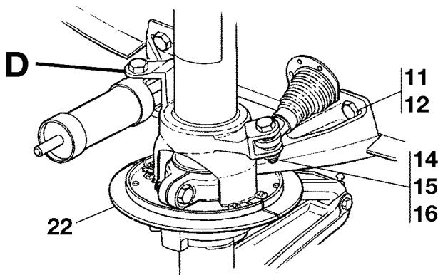
DETAIL C
