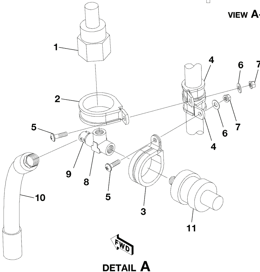
OIL INDICATING SYSTEM - J182T FIGURE 02 (SHEET 1)
