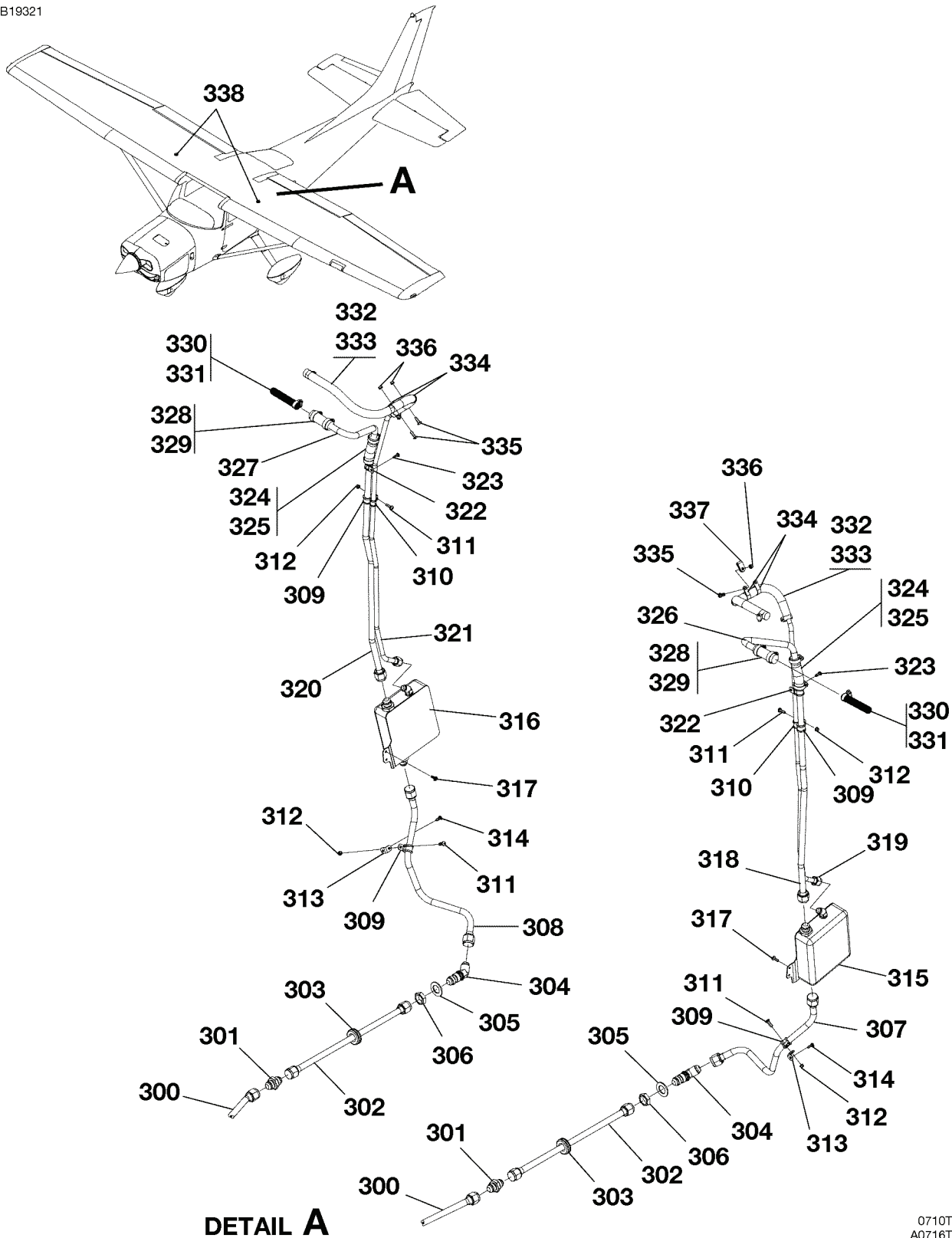
FUEL SYSTEM - J182T FIGURE 03 (SHEET 5)
