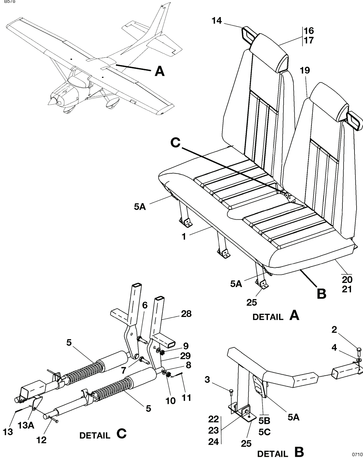
AFT BENCH SEAT INSTALLATION - RECLINING BACK FIGURE 01 (SHEET 1)
