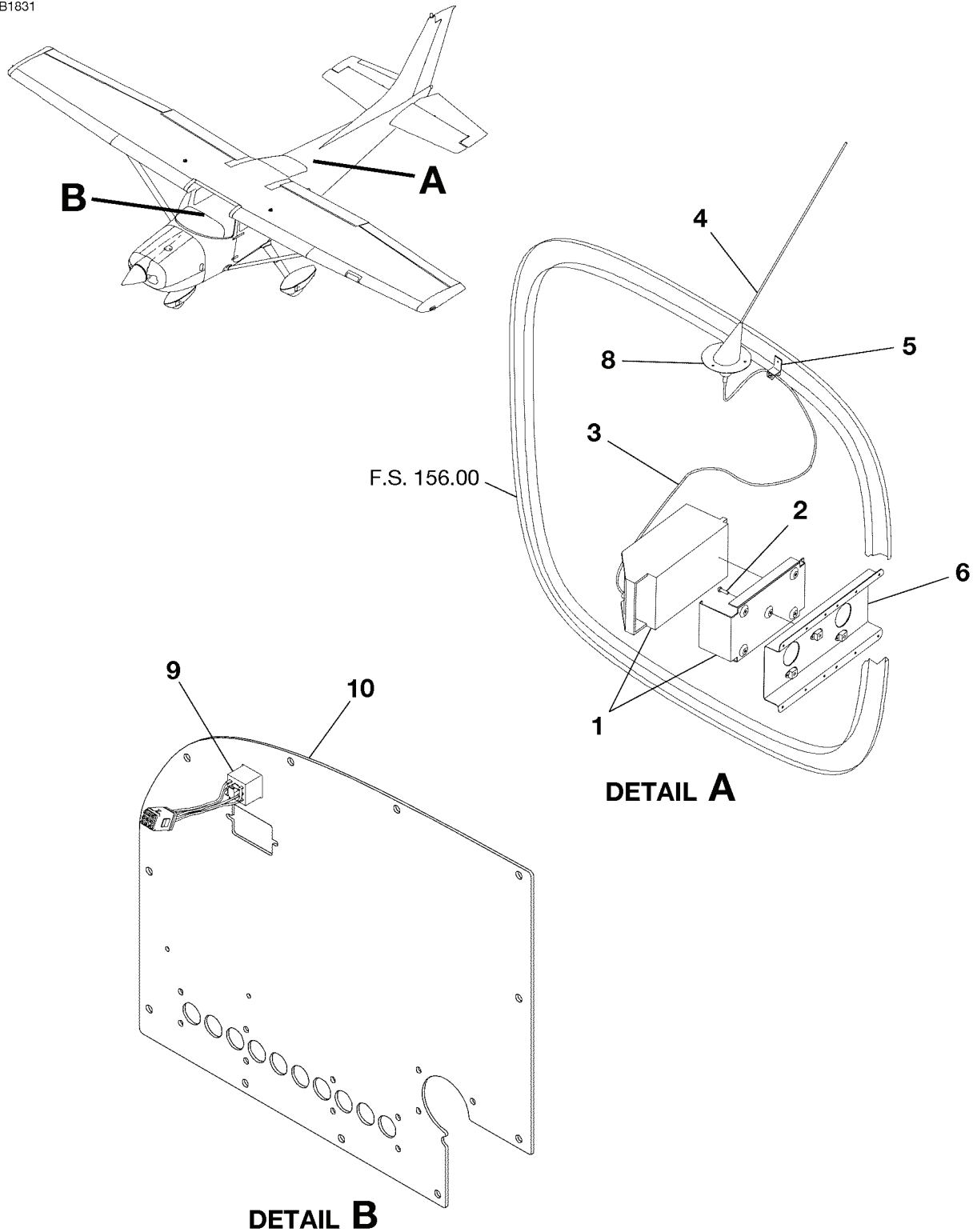
EMERGENCY LOCATOR TRANSMITTER AND ANTENNA INSTALLATION FIGURE 02 (SHEET 1)
