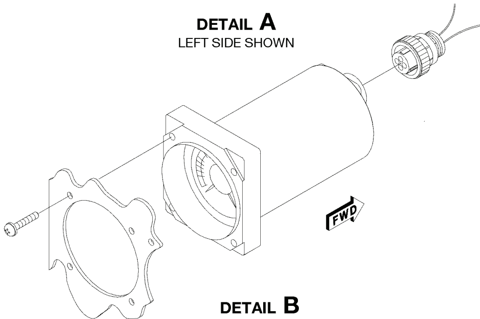
FUEL INDICATING SYSTEM FIGURE 02 (SHEET 1)
