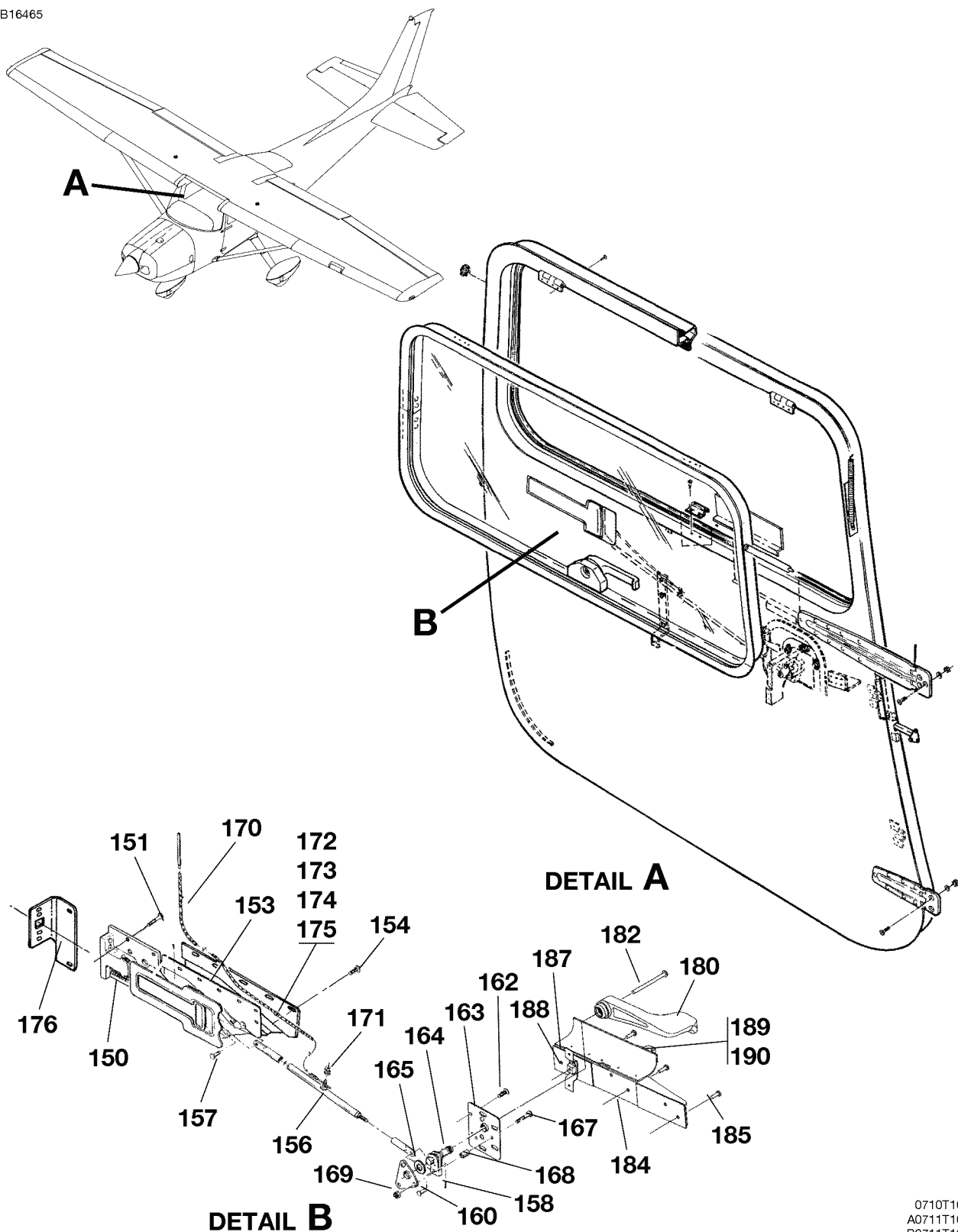
CABIN DOOR INSTALLATION - RH FIGURE 02 (SHEET 3)
