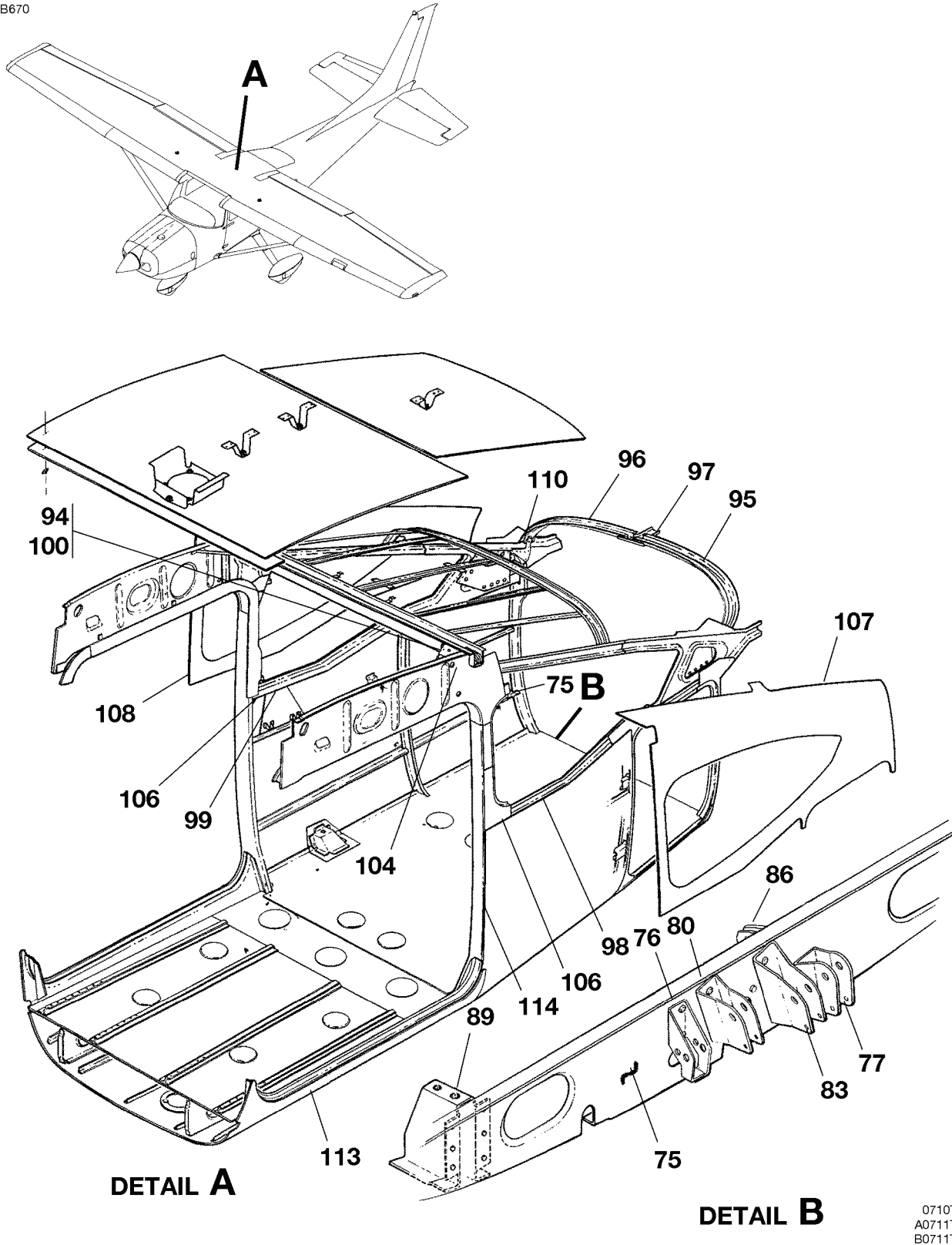
CENTER SECTION CABIN ASSEMBLY FIGURE 03 (SHEET 2)
