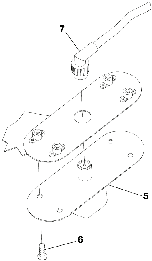
DETAIL B
