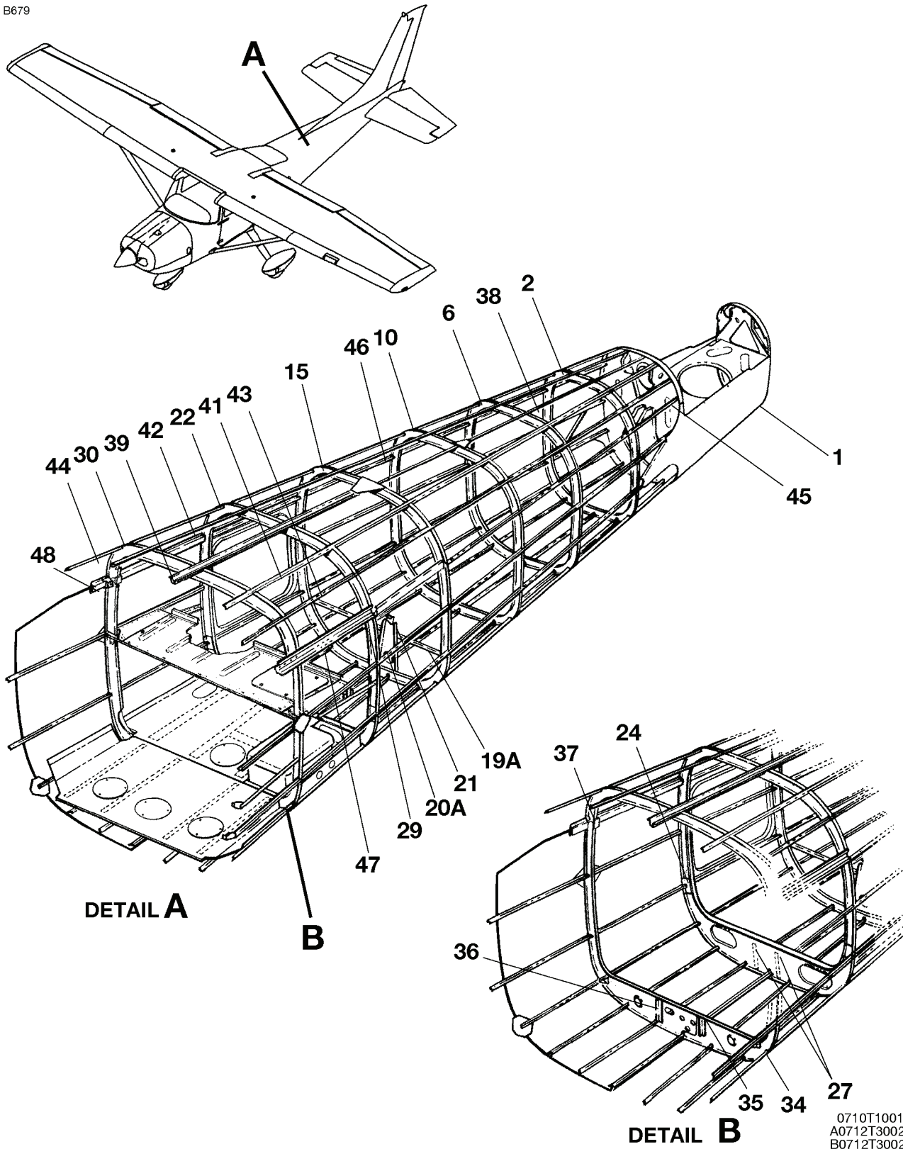
TAILCONE ASSEMBLY FIGURE 01 (SHEET 1)
