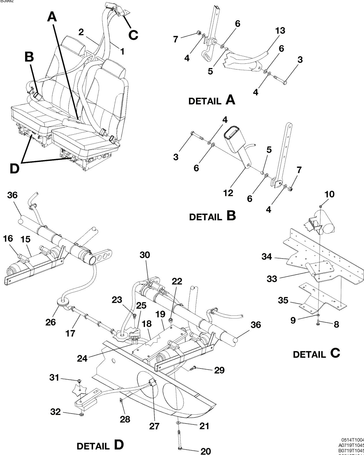
AMSAFE INFLATABLE RESTRAINT SYSTEM - PILOT AND COPILOT FIGURE 01A (SHEET 1)
