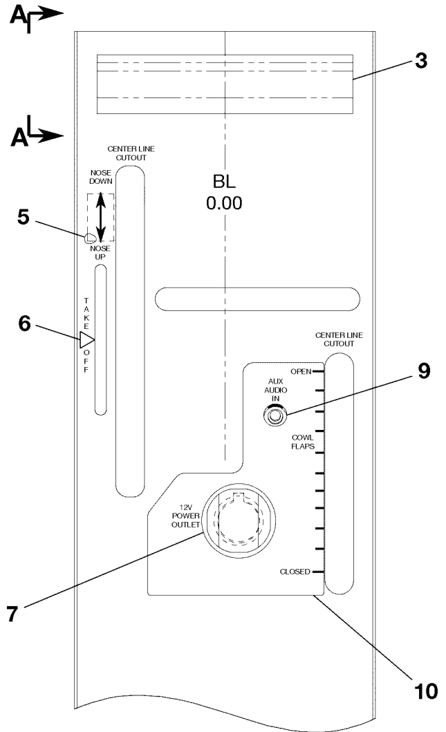
DETAIL A
