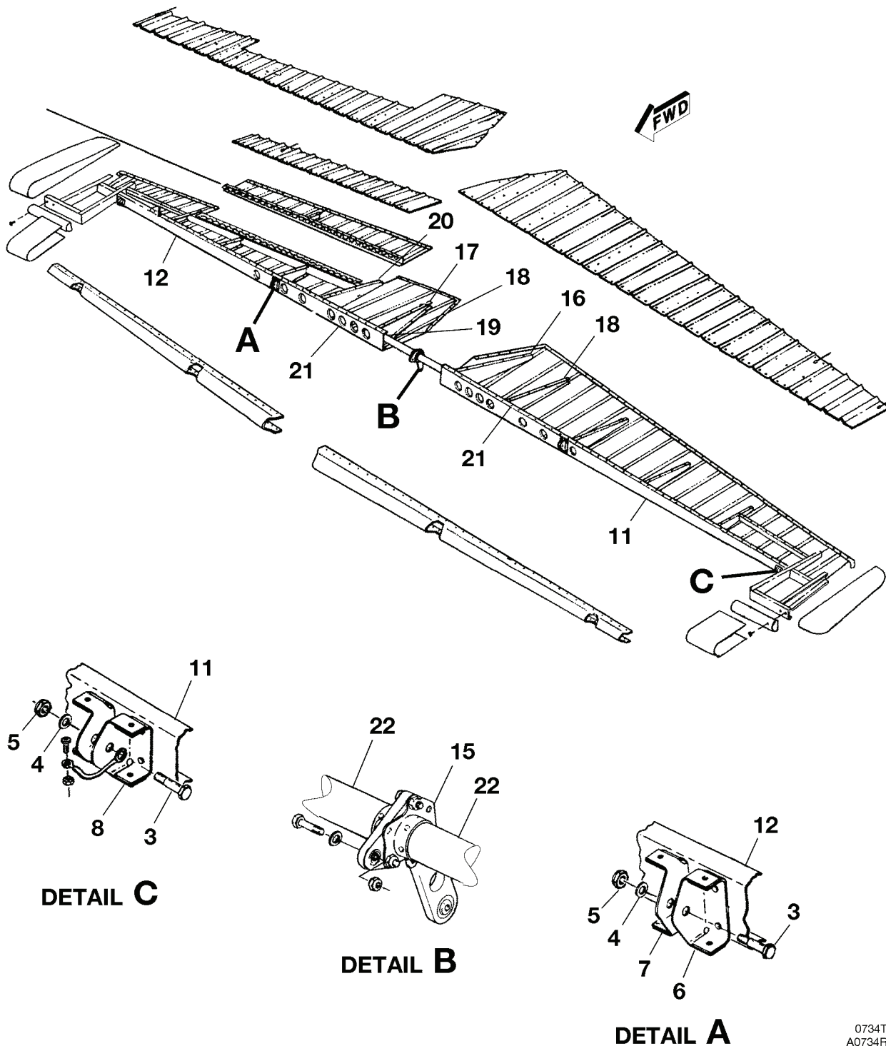
ELEVATOR INSTALLATION FIGURE 01 (SHEET 1)
