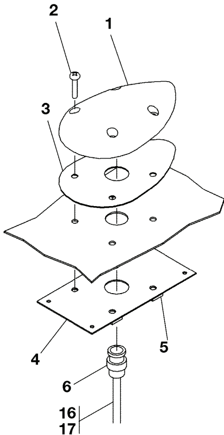
DETAIL C
