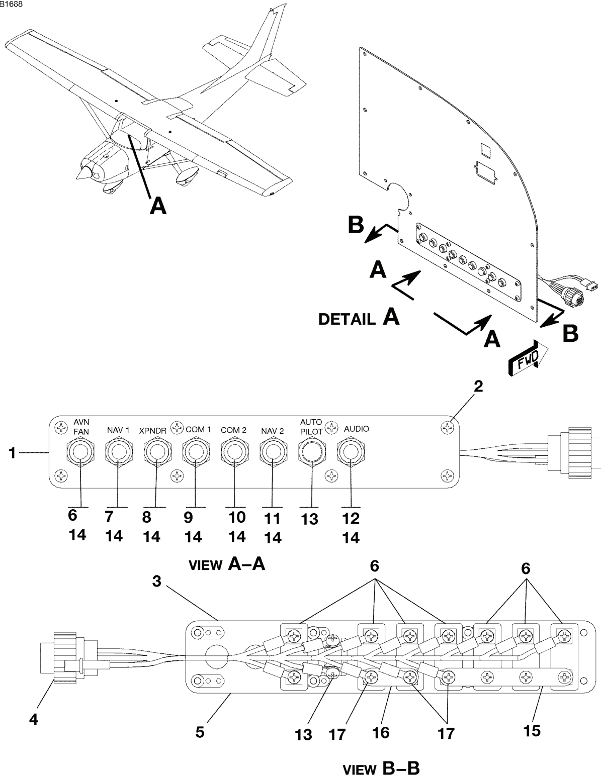
CIRCUIT BREAKER PANEL ASSEMBLY - GARMIN FIGURE 04 (SHEET 1)
