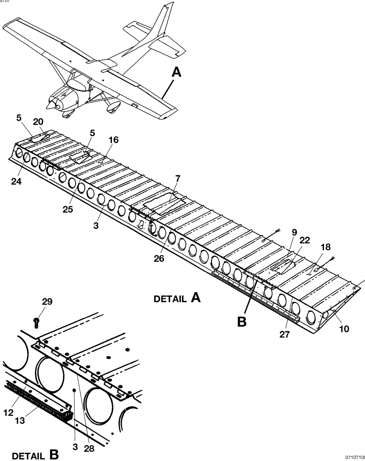
AILERON ASSEMBLY FIGURE 01 (SHEET 1)
