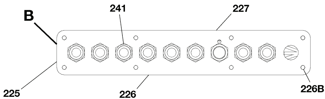
DETAIL A NAV II WITH ADF AIRPLANES 18280945 AND ON AND AIRPLANES T18208001 AND ON
