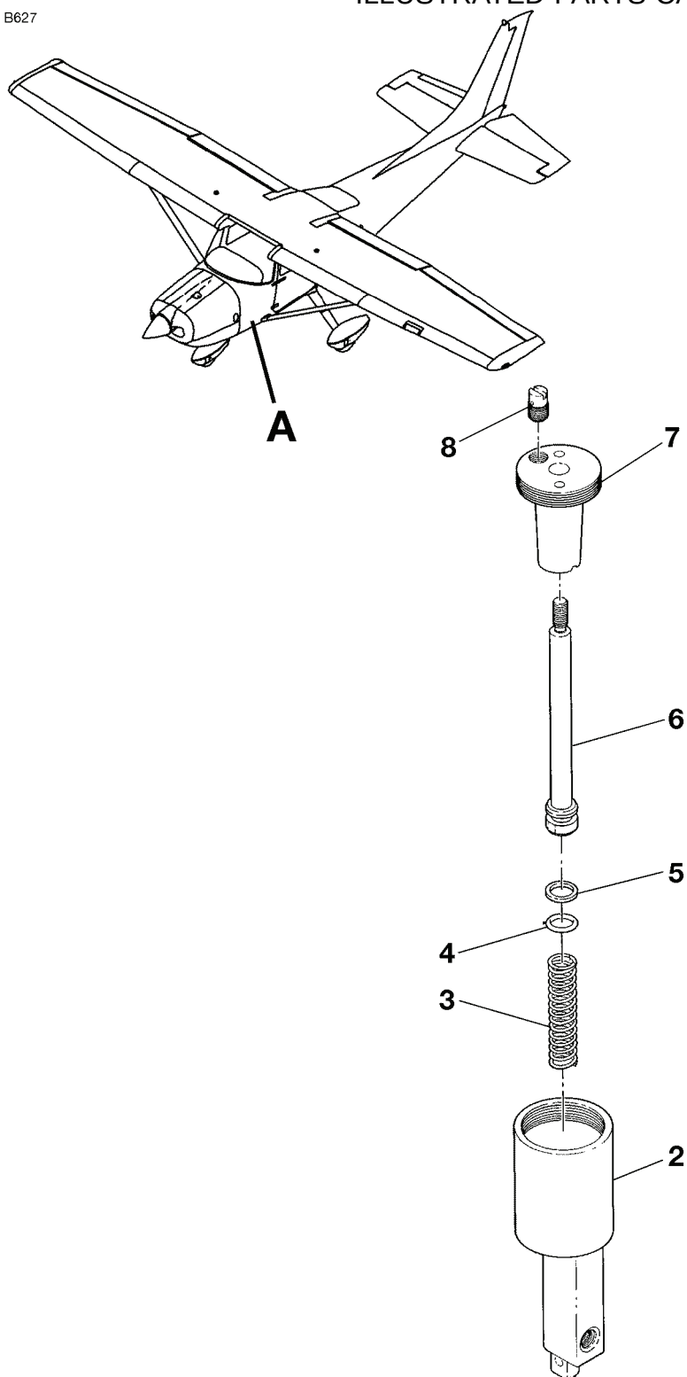
MASTER BRAKE CYLINDER ASSEMBLY FIGURE 01 (SHEET 1)
