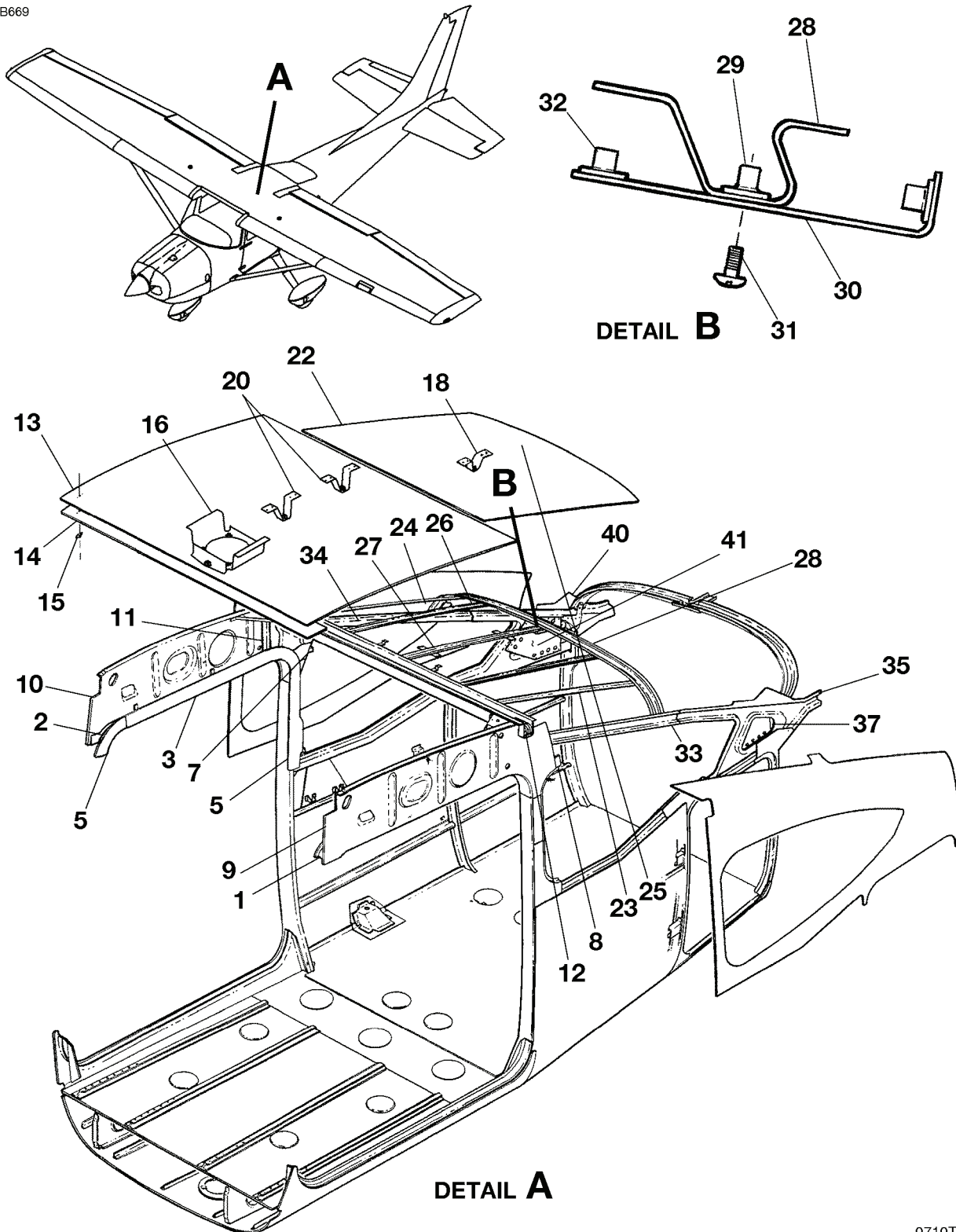
CENTER SECTION CABIN ASSEMBLY FIGURE 03 (SHEET 1)
