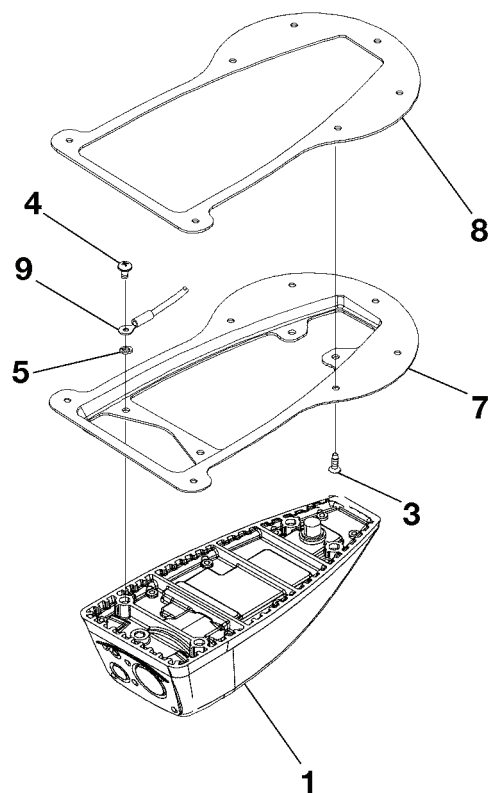
DETAIL B
