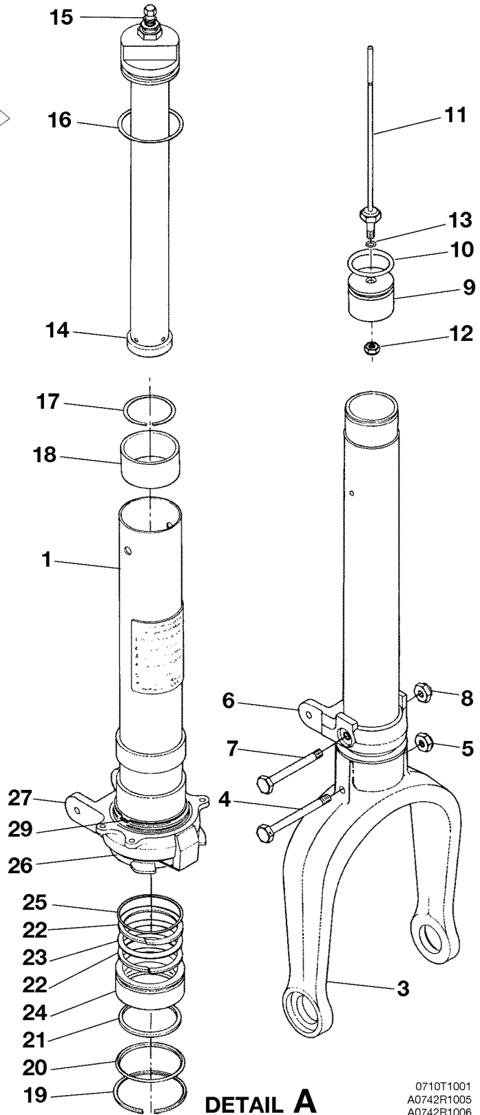
NOSE GEAR SHOCK STRUT ASSEMBLY FIGURE 01 (SHEET 1)
