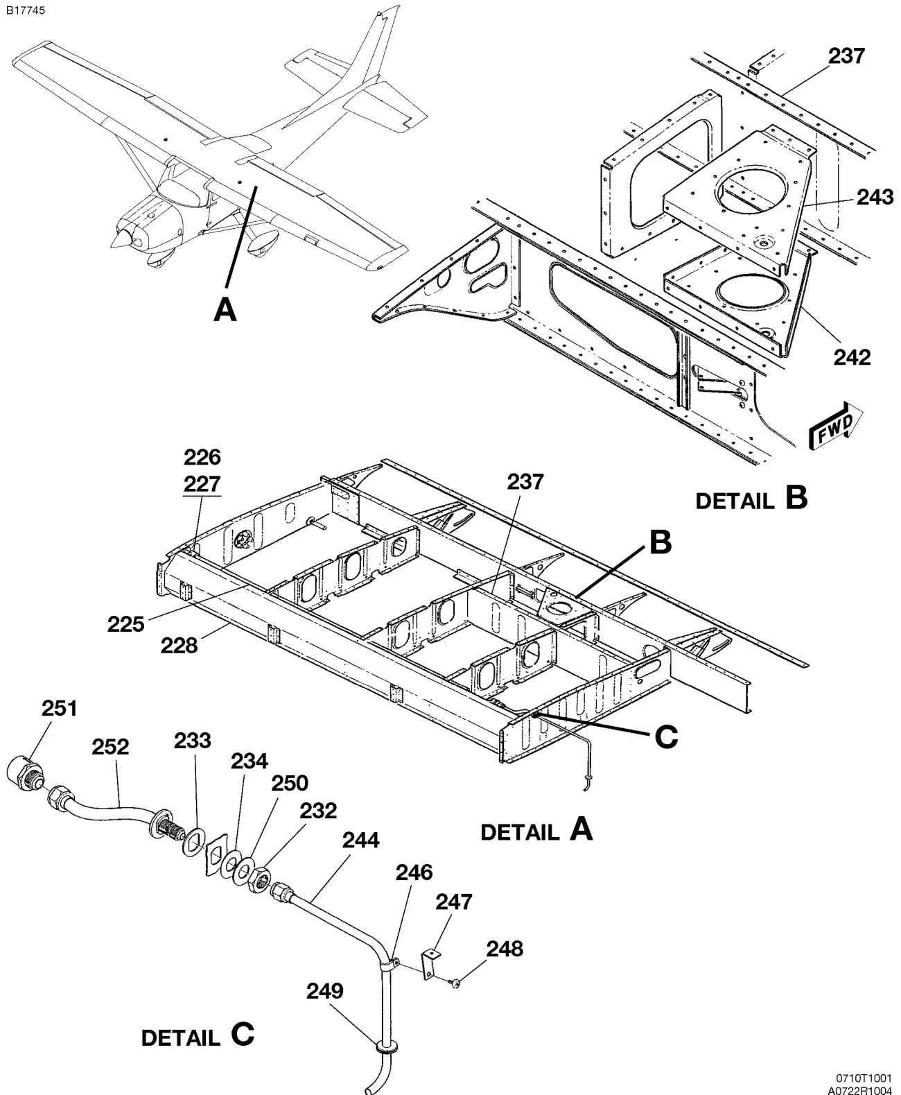
FUEL BAY STRUCTURE ASSEMBLY FIGURE 02 (SHEET 4)
