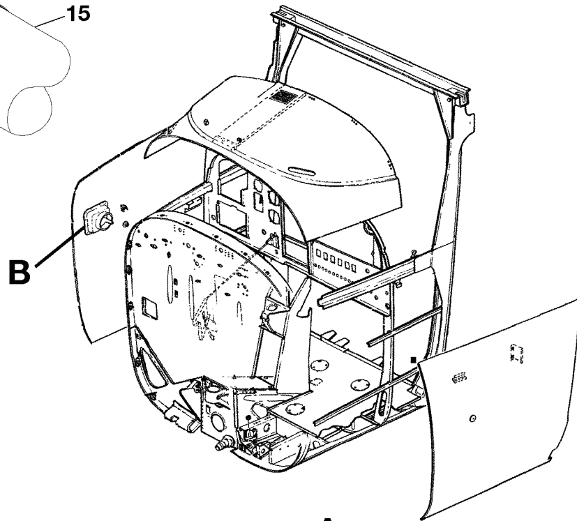
DETAIL A
