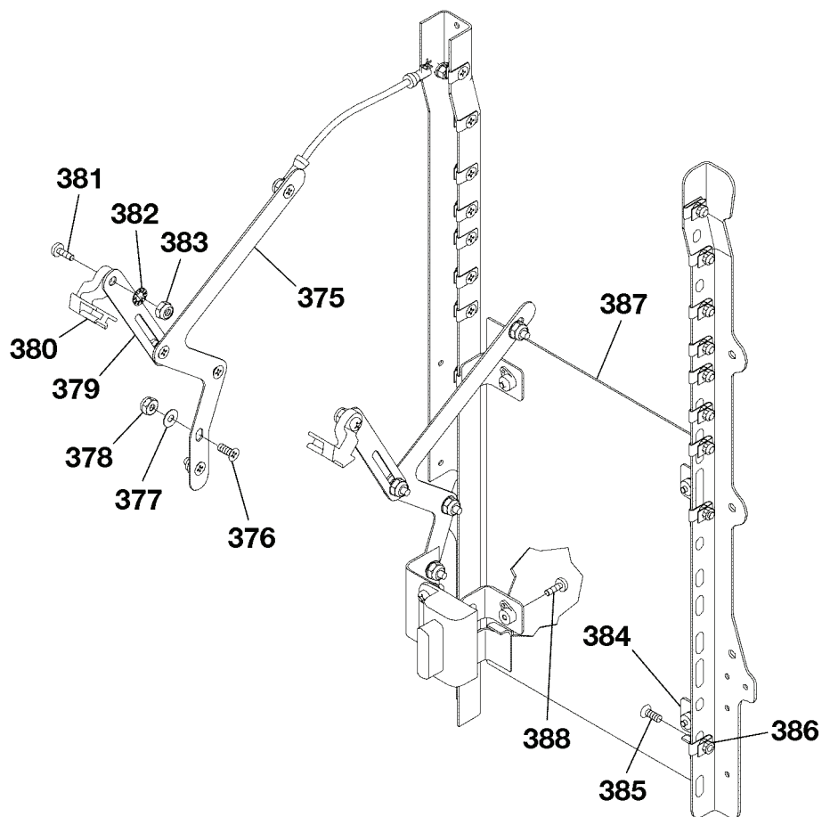
DETAIL A
