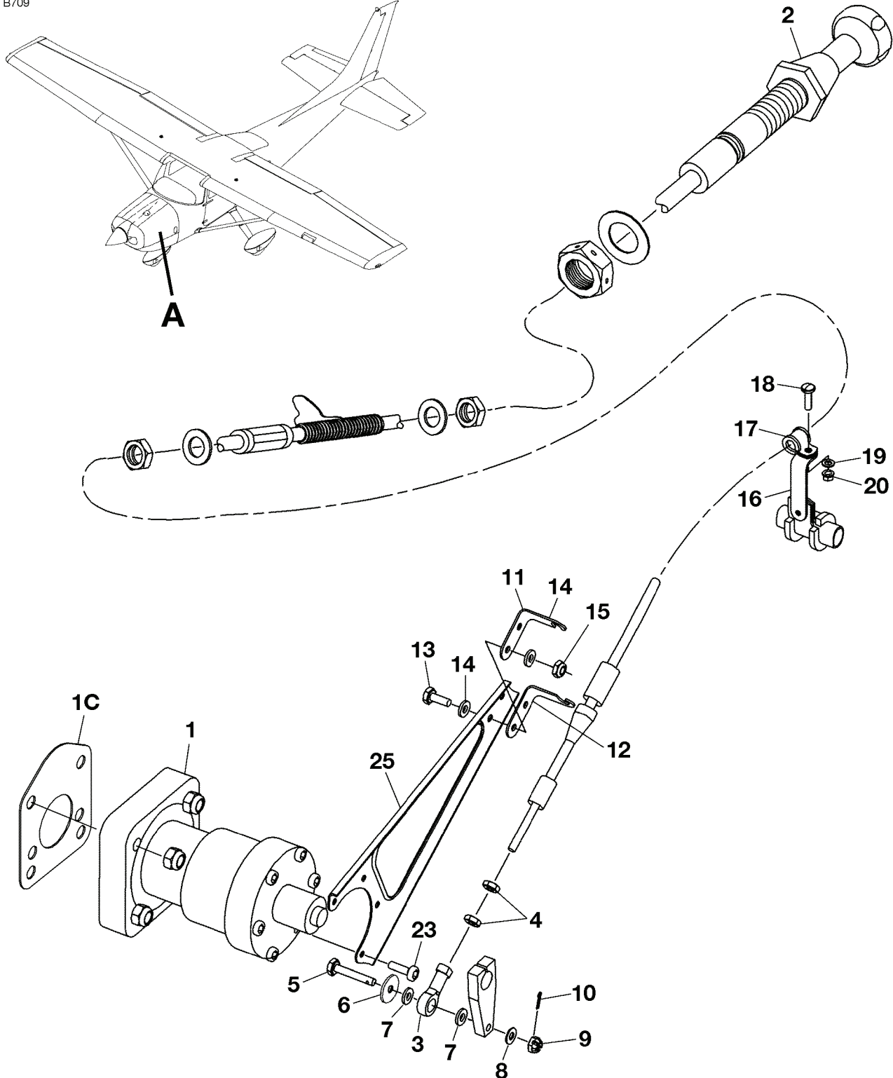
GOVERNOR INSTALLATION - PROPELLER FIGURE 01 (SHEET 1)
