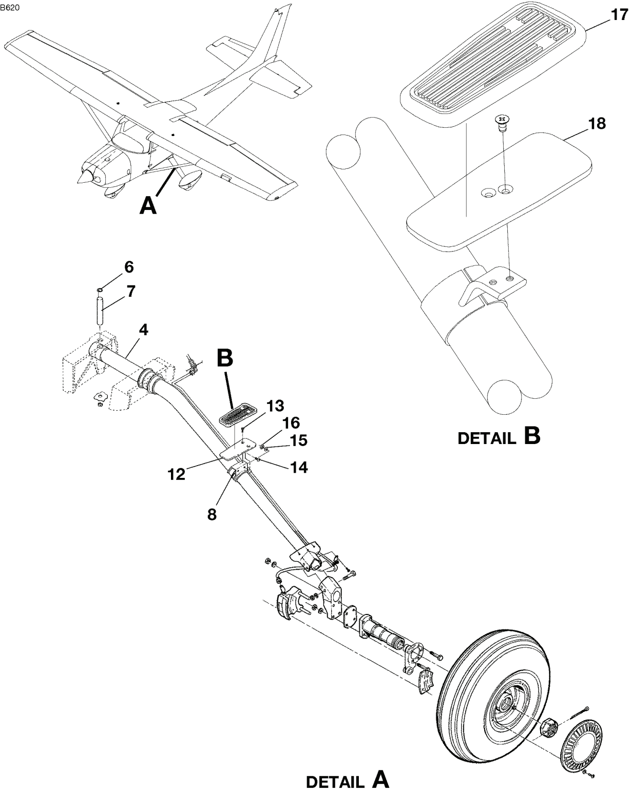
MAIN LANDING GEAR INSTALLATION FIGURE 01 (SHEET 1)
