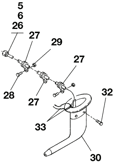
DETAIL C
