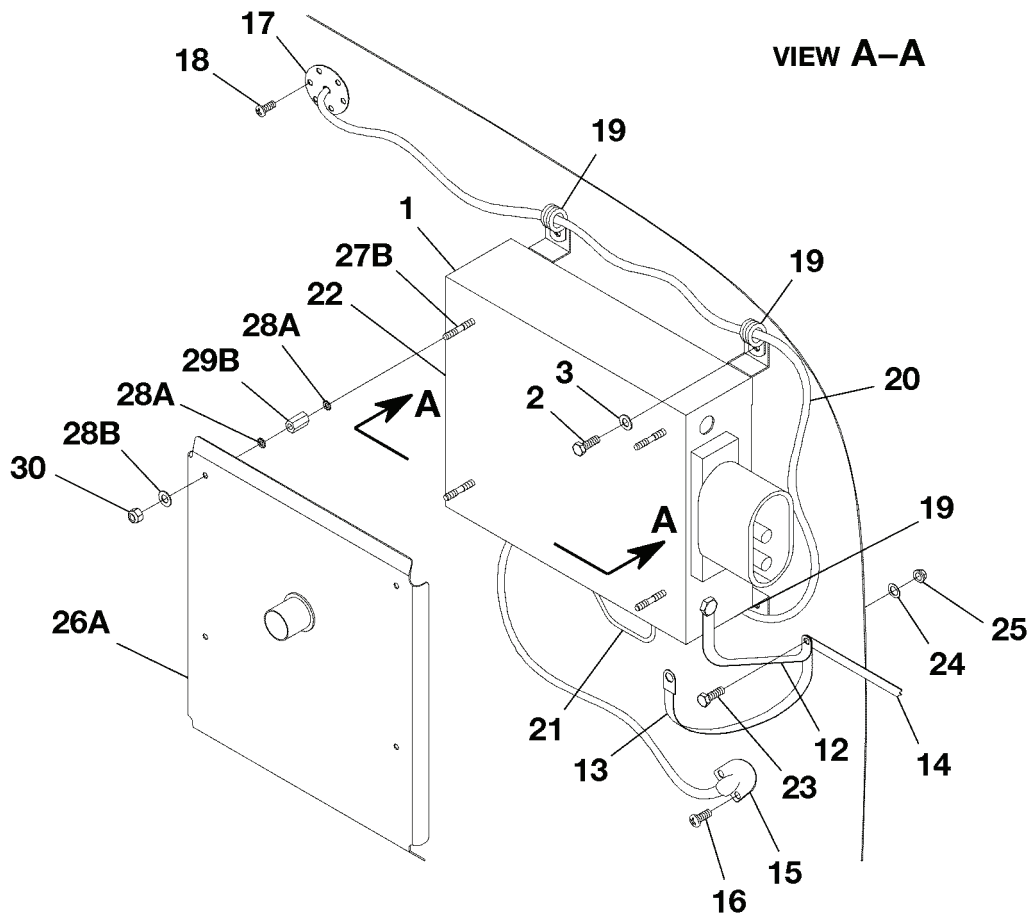
POWER JUNCTION BOX INSTALLATION FIGURE 01 (SHEET 1)
