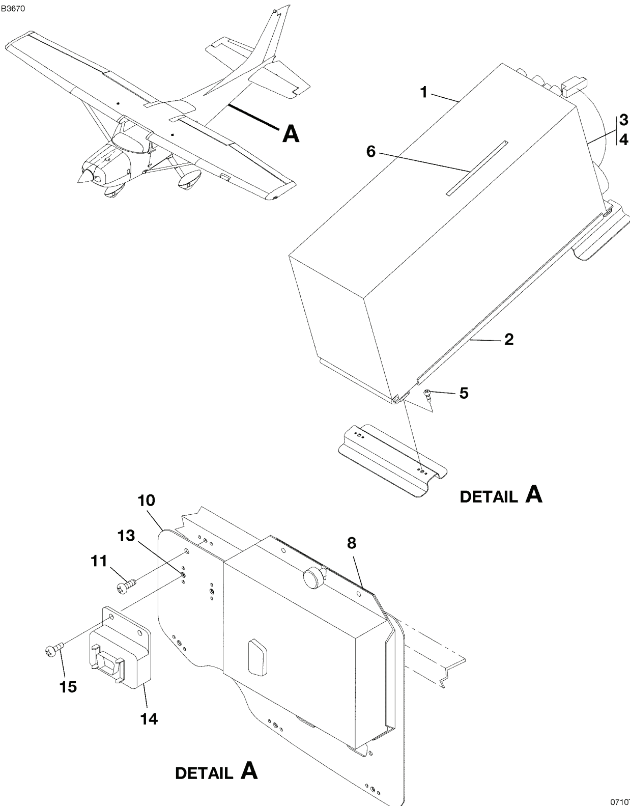
KMH-880 RECEIVER INSTALLATION FIGURE 01 (SHEET 1)
