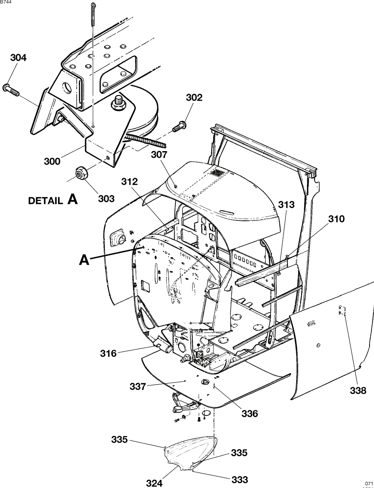
FORWARD FUSELAGE ASSEMBLY FIGURE 01 (SHEET 5)
