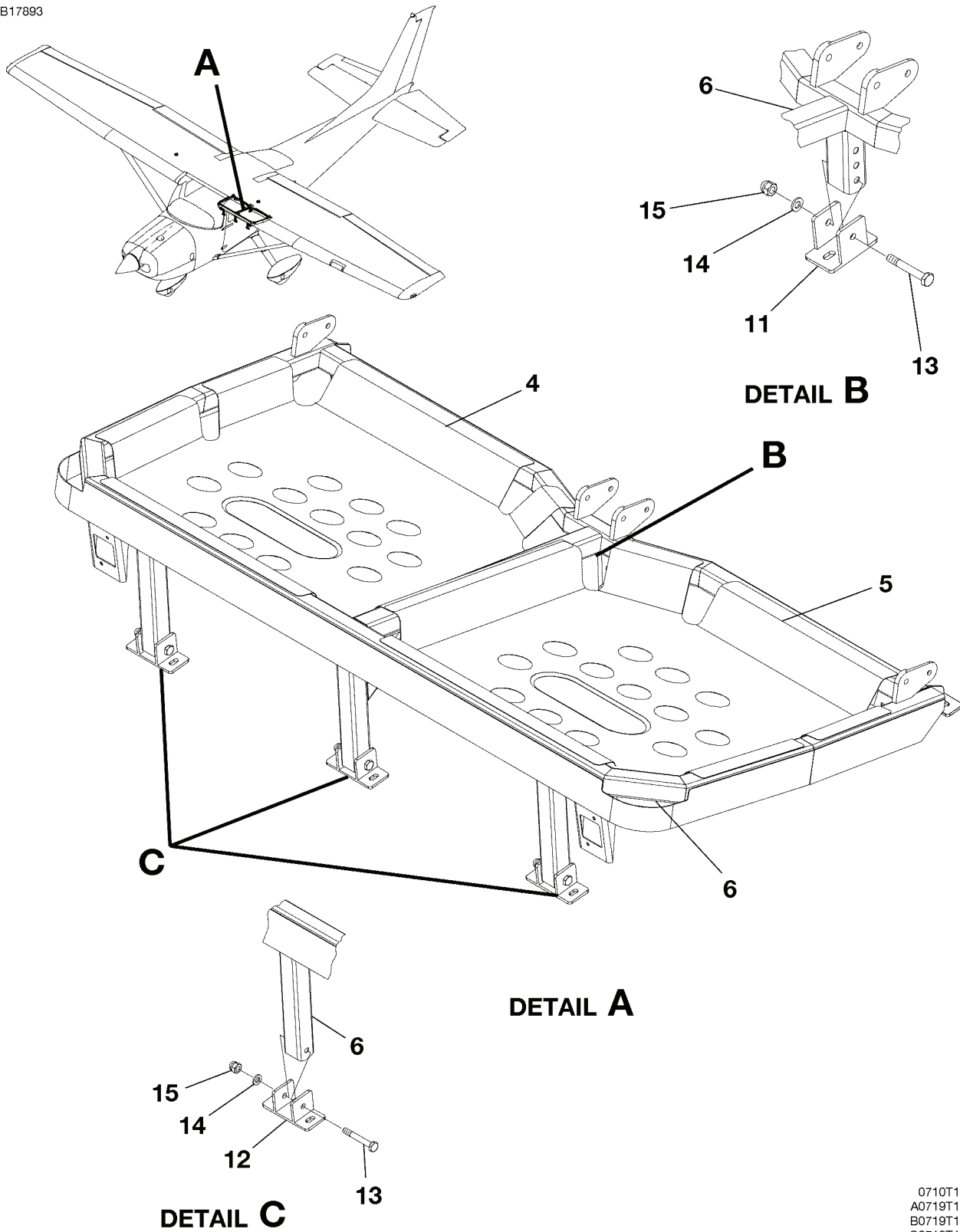
SEAT FRAME ASSY FIGURE 05 (SHEET 1)
