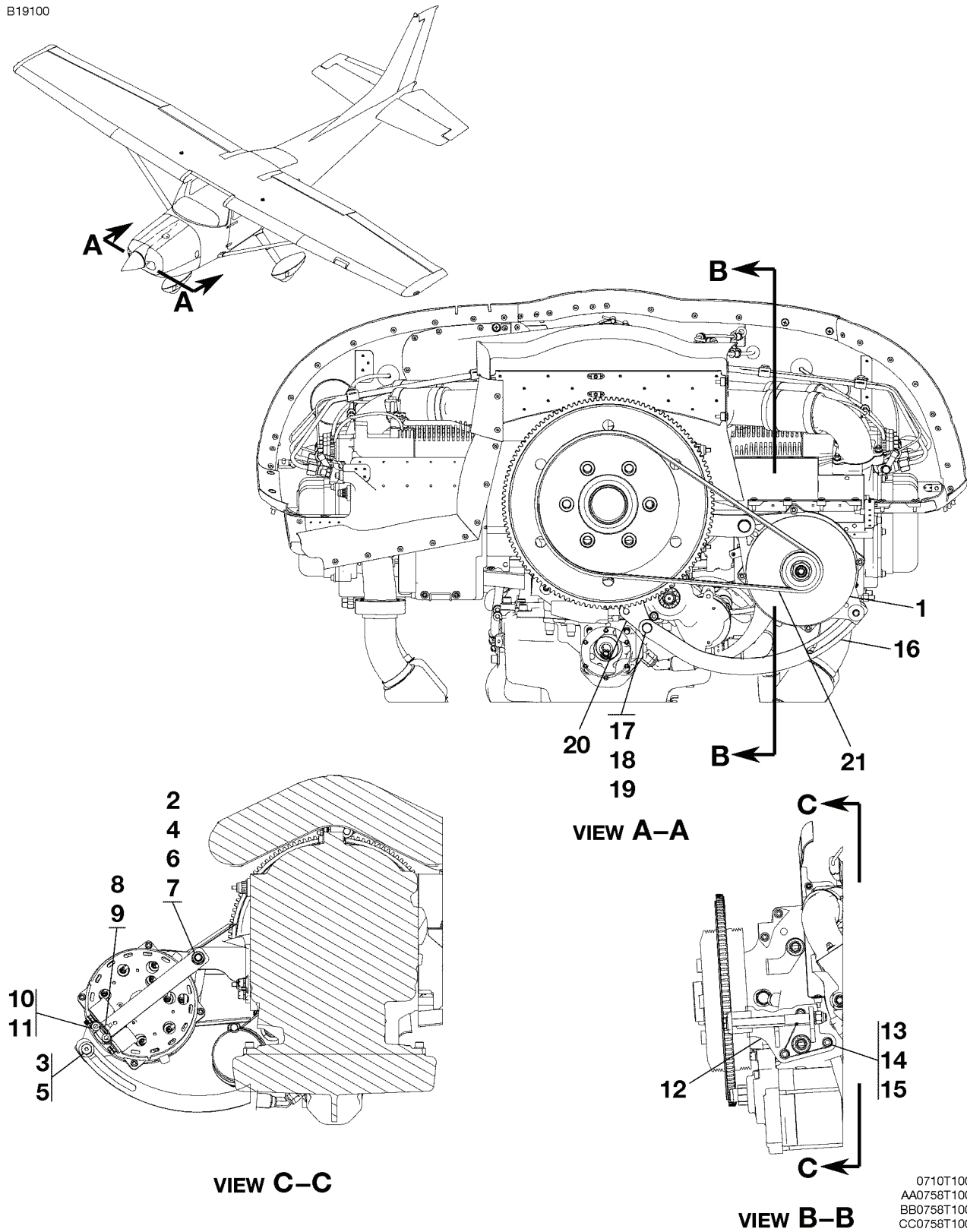
ALTERNATOR INSTALLATION - J182T FIGURE 01A (SHEET 1)
