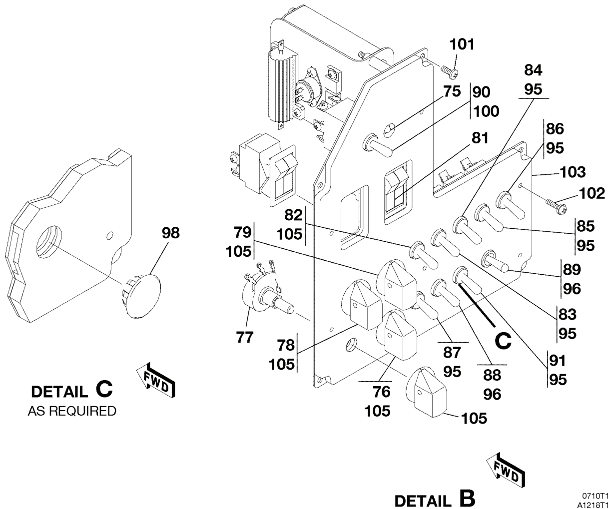
SWITCH PANEL INSTALLATION - NAV III FIGURE 03 (SHEET 2)
