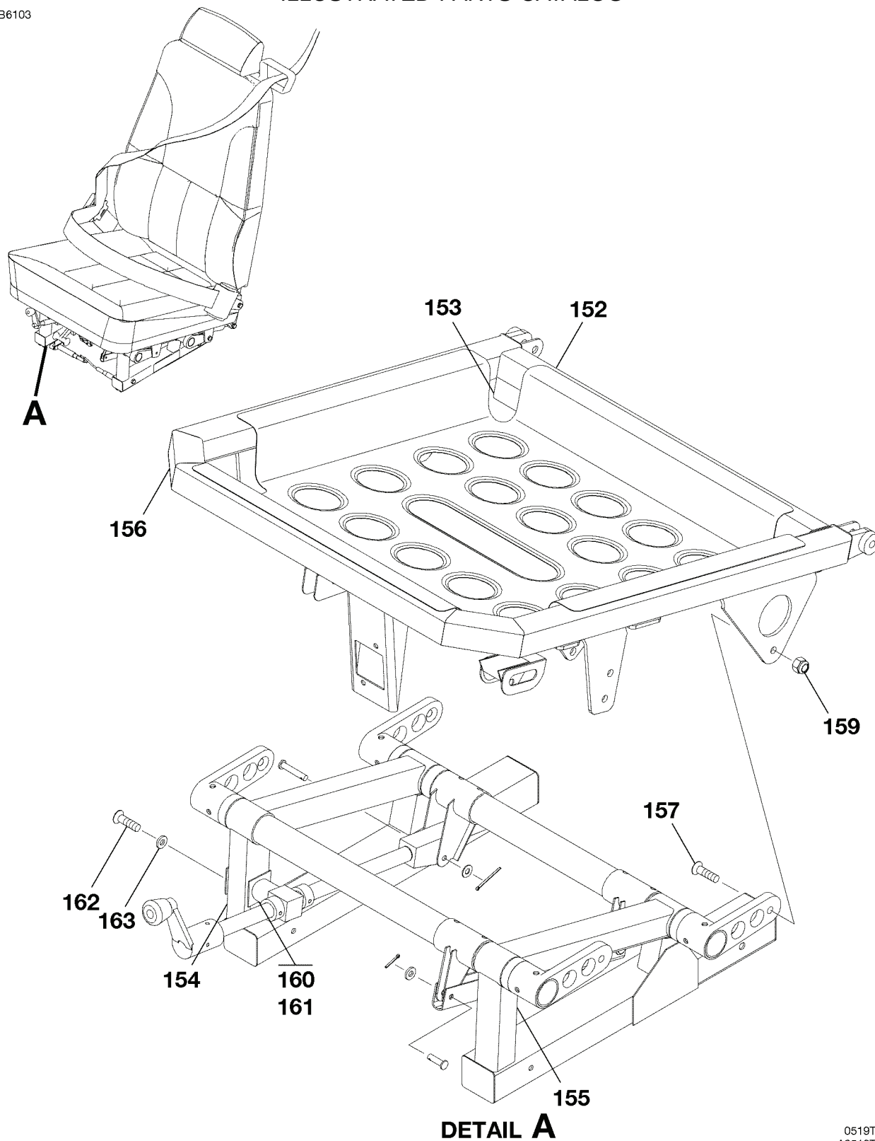
SEAT ASSEMBLY-PILOT AND COPILOT FIGURE 02A (SHEET 3)
