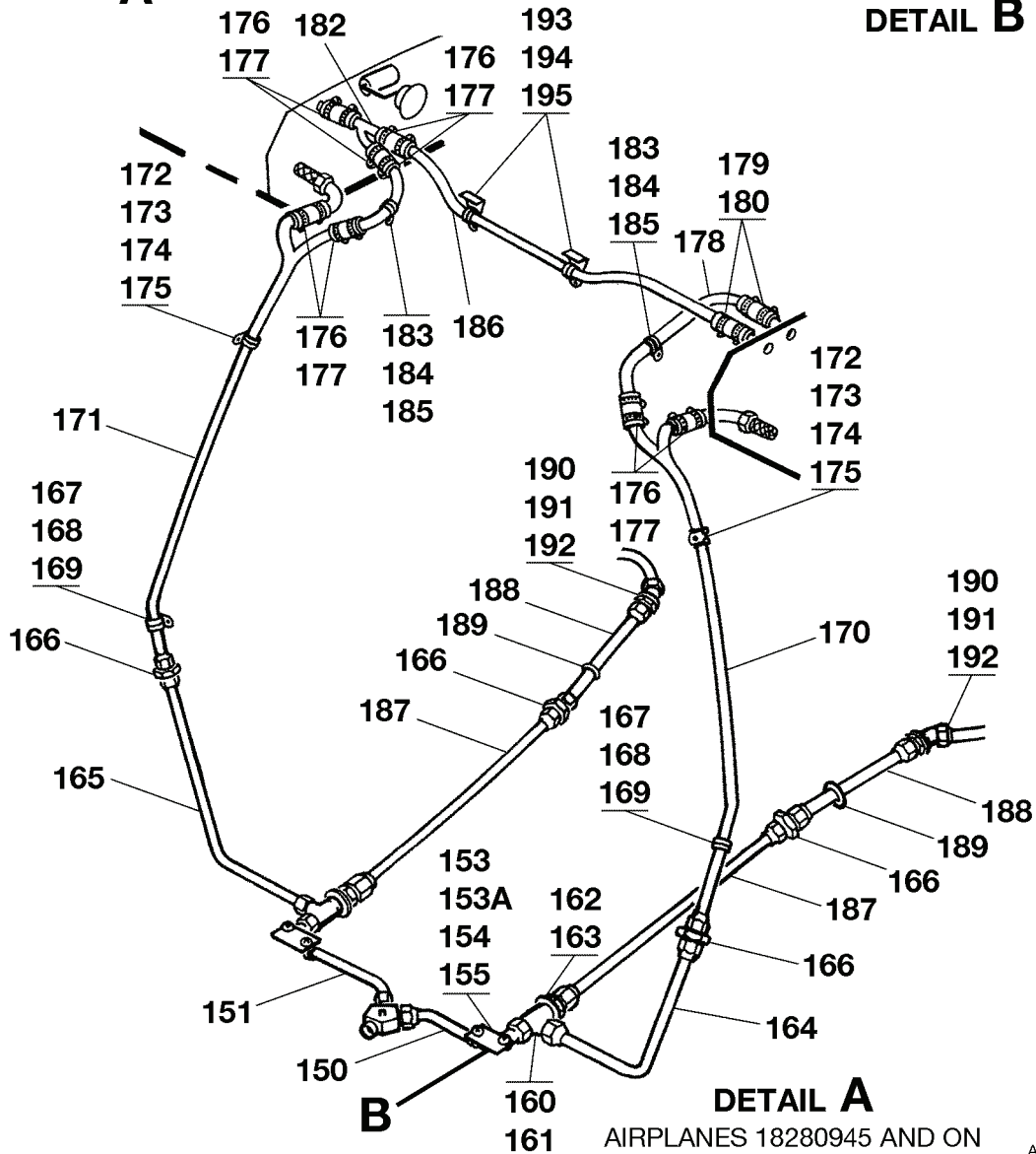
FUEL SYSTEM - 182/T182 FIGURE 02 (SHEET 3)
