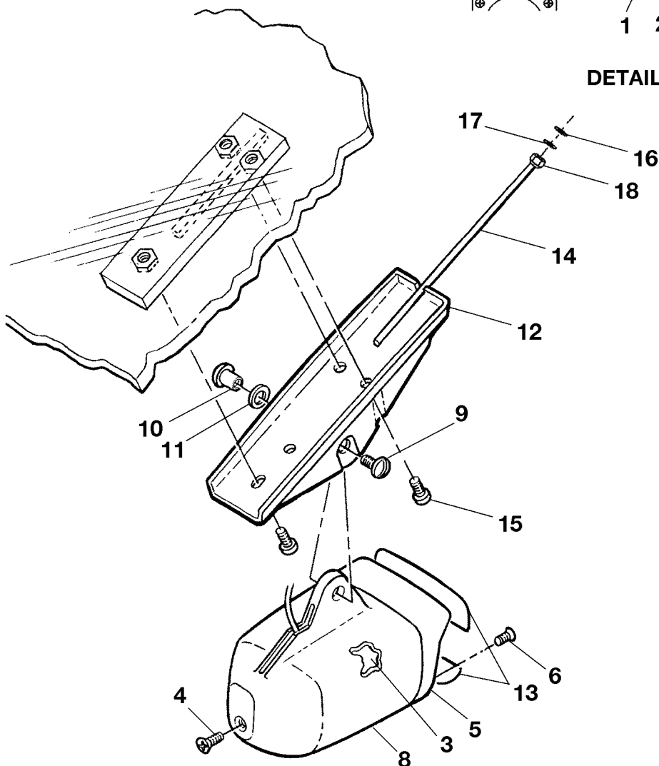
DETAIL B
