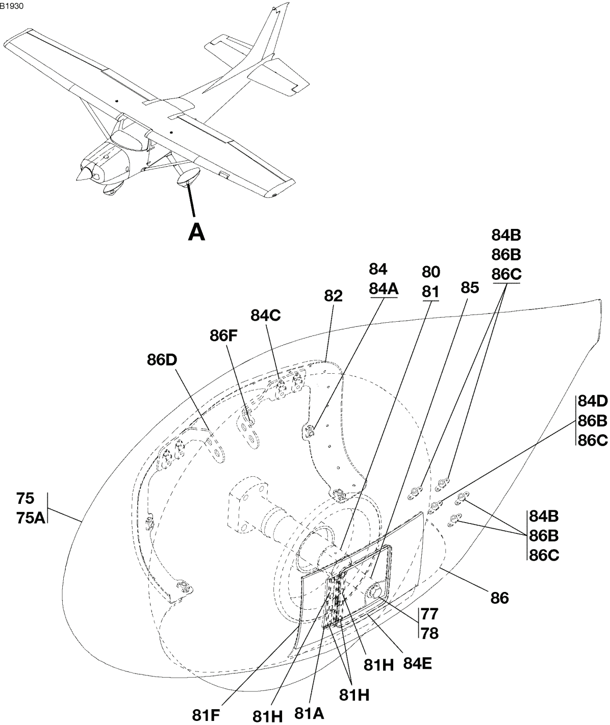
DETAIL A
