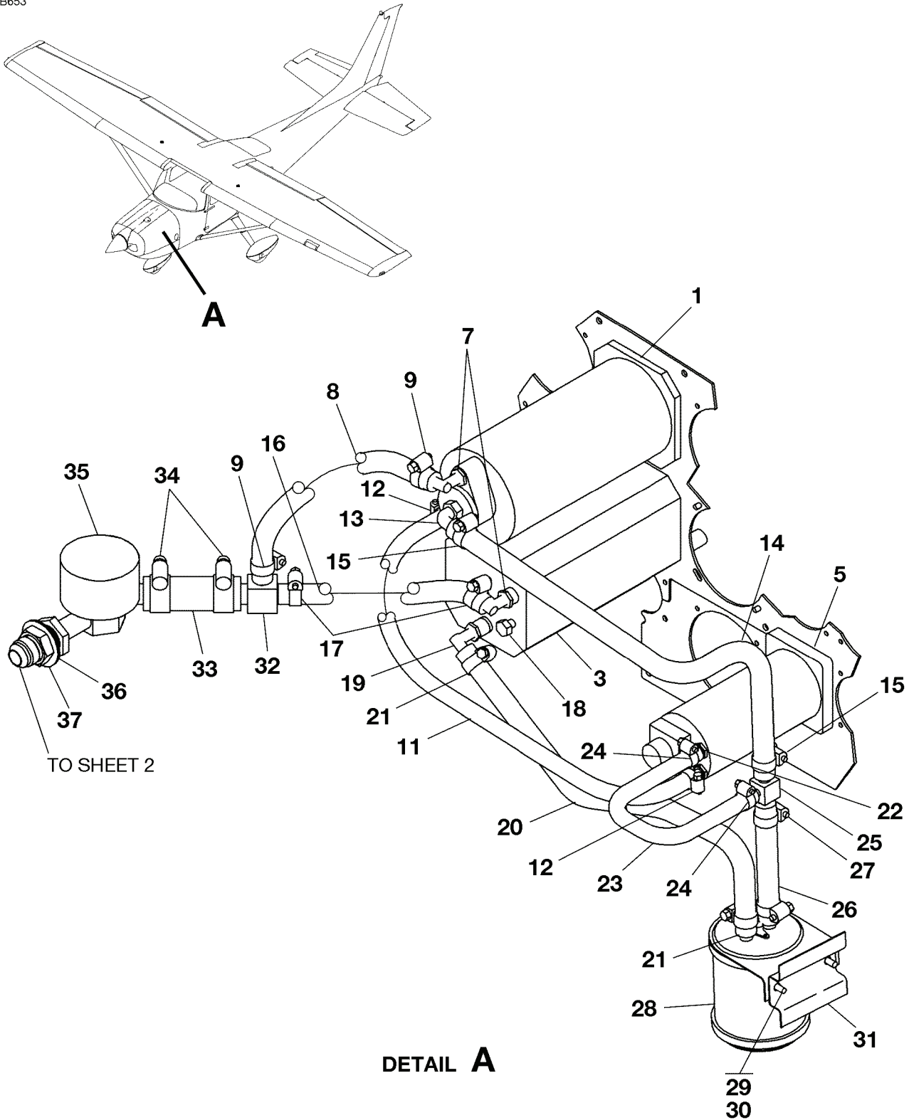
VACUUM SYSTEM FIGURE 01 (SHEET 1)
