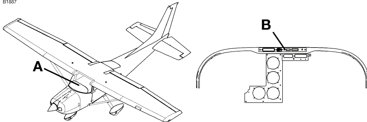
DETAIL A
