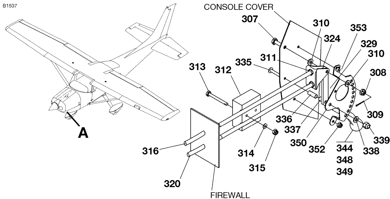
DETAIL B
