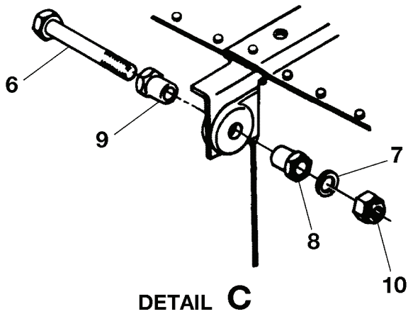
WING INSTALLATION FIGURE 01 (SHEET 1)
