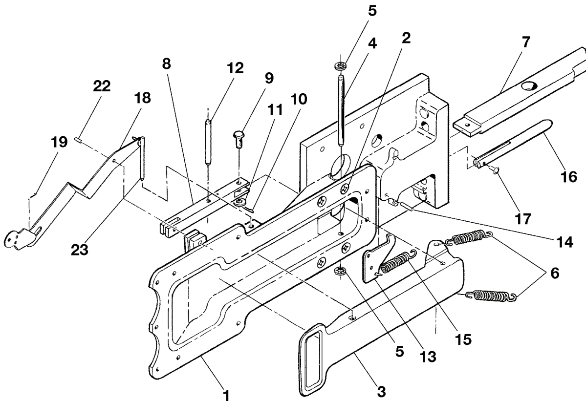
DETAIL A
