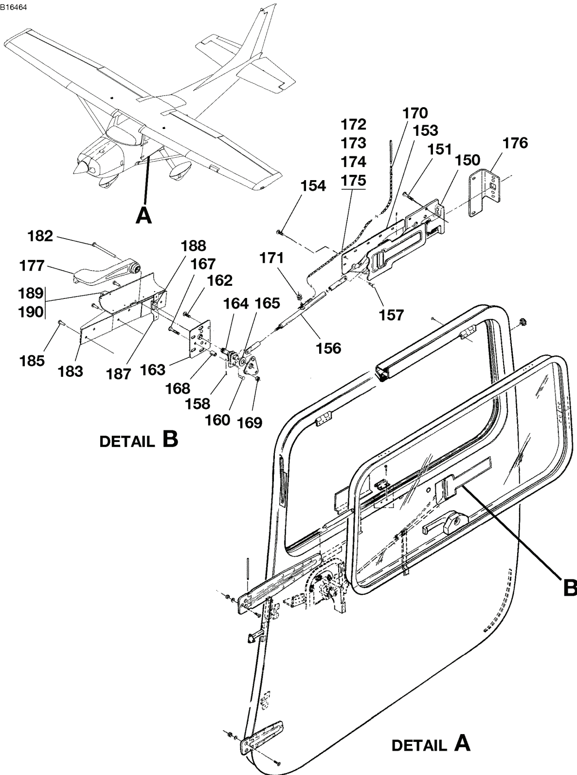
CABIN DOOR INSTALLATION - LH FIGURE 01 (SHEET 3)
