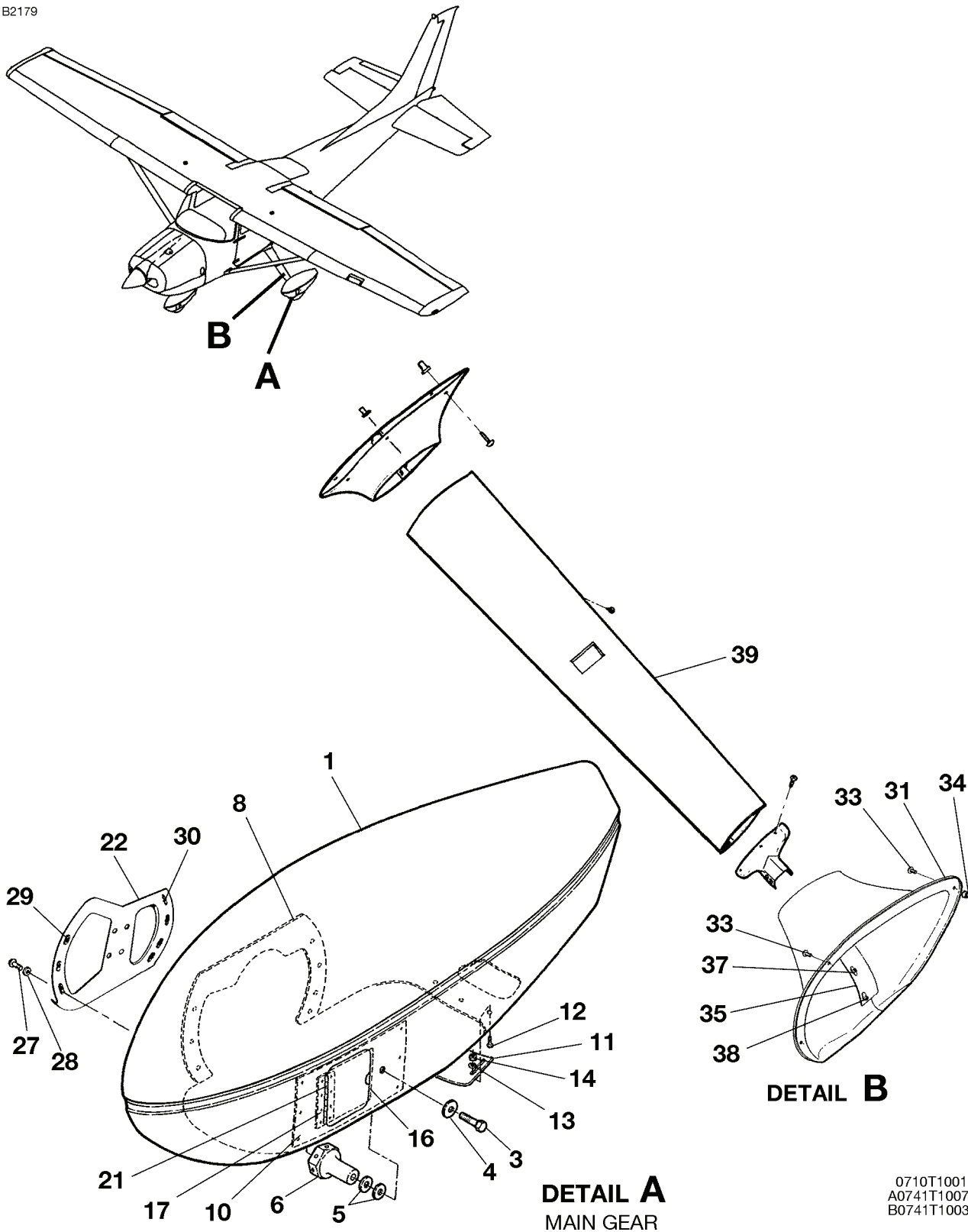
LANDING GEAR FAIRING INSTALLATION FIGURE 01 (SHEET 1)
