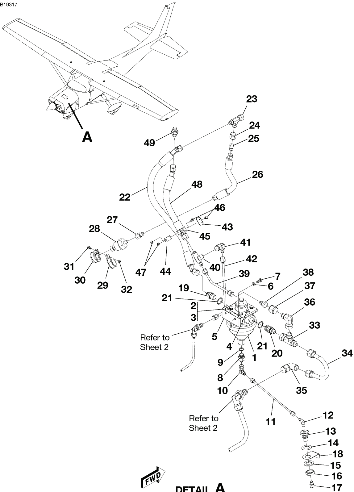
FUEL SYSTEM - J182T FIGURE 03 (SHEET 1)
