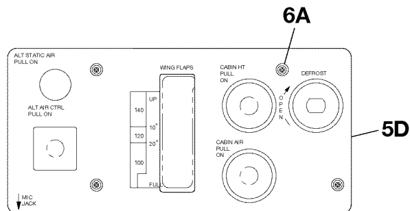
DETAIL C AIRPLANES J1820001 AND ON LED PANEL INSTALLATION FIGURE 01 (SHEET 1)
