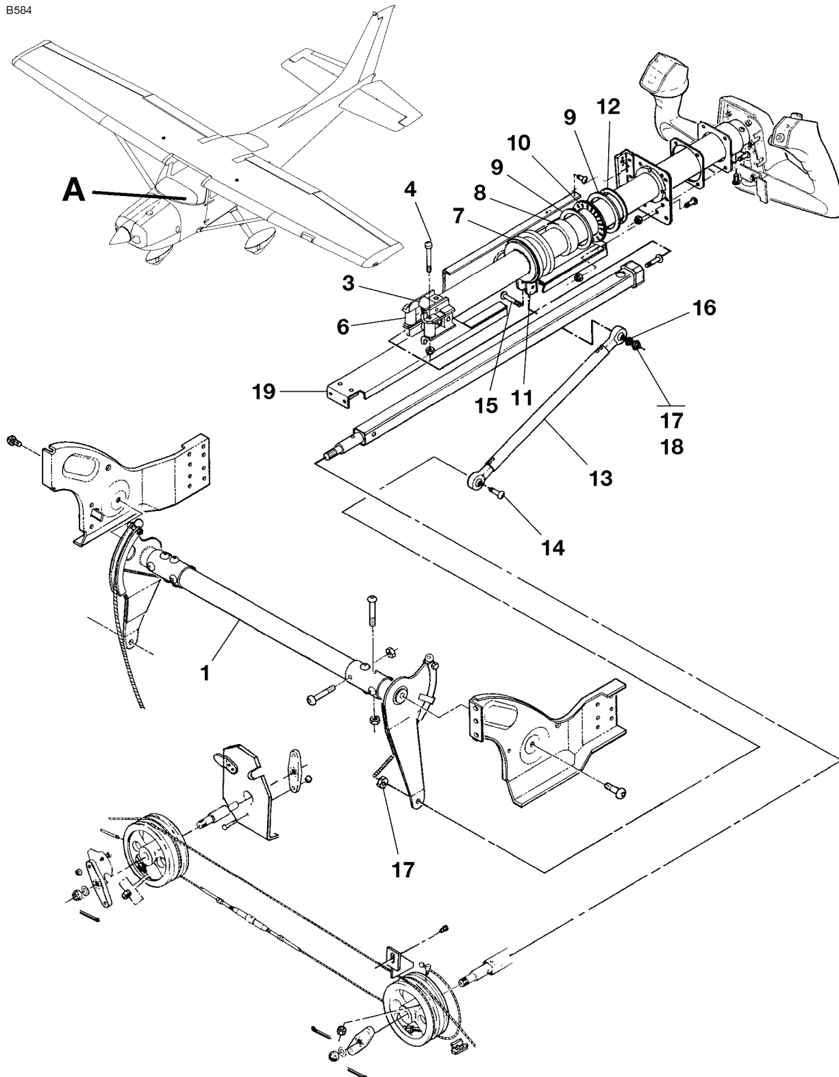
CONTROL COLUMN INSTALLATION FIGURE 01 (SHEET 1)
