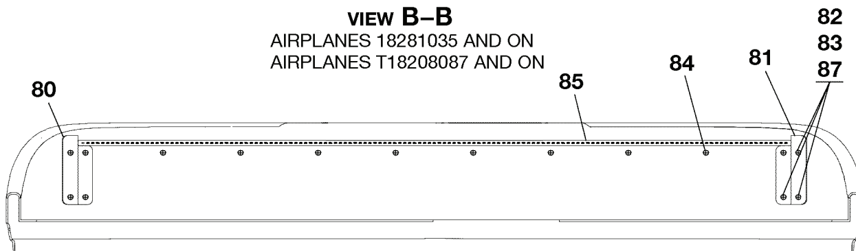
VIEW B-B AIRPLANES 18280945 THRU 18281034 AND AIRPLANES T18208001 THRU T18208086 INSTRUMENT PANEL LIGHT INSTALLATION FIGURE 01 (SHEET 2)
