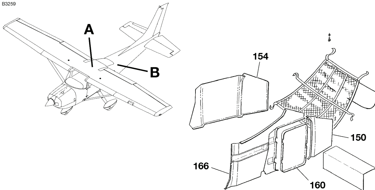
DETAIL B
