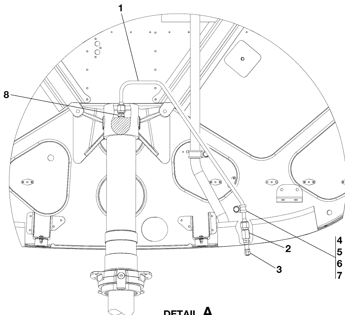
NOSE LANDING GEAR EXTENSION SERVICE INSTALLATION - J182T FIGURE 01 (SHEET 1)
