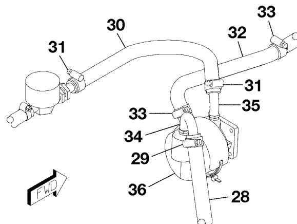
VACUUM SYSTEM - NAV III FIGURE 01A (SHEET 1)
