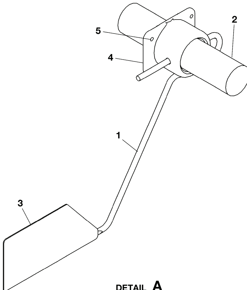
CONTROL LOCK FIGURE 01 (SHEET 1)
