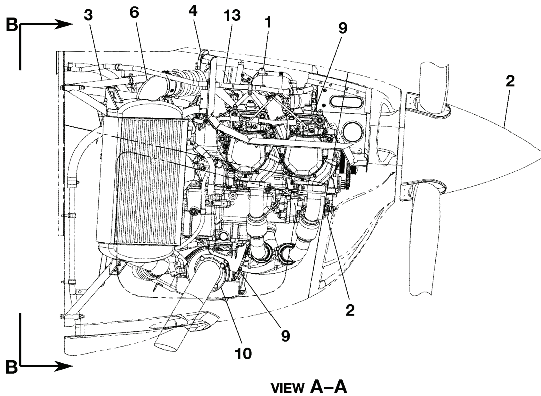
ENGINE COMPONENTS - J182T FIGURE 03 (SHEET 1)
