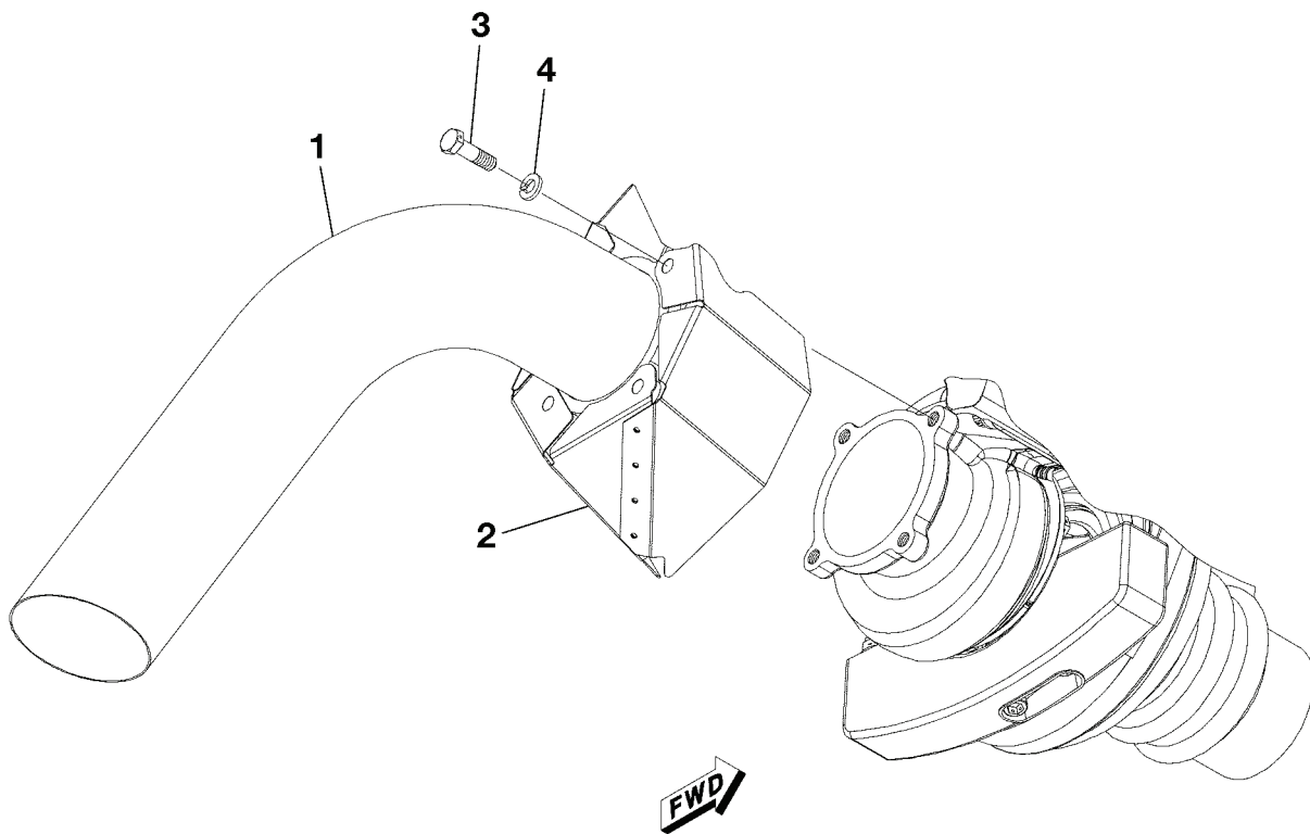
DETAIL A
