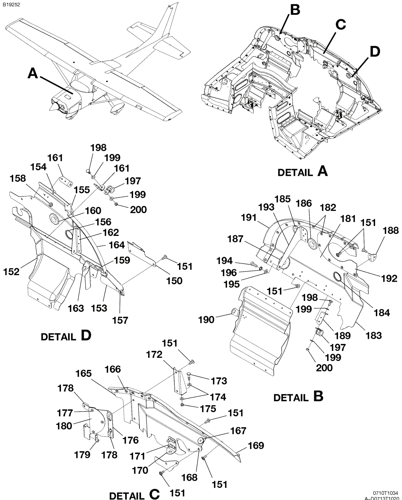
BAFFLE INSTALLATION - J182T FIGURE 03 (SHEET 3)
