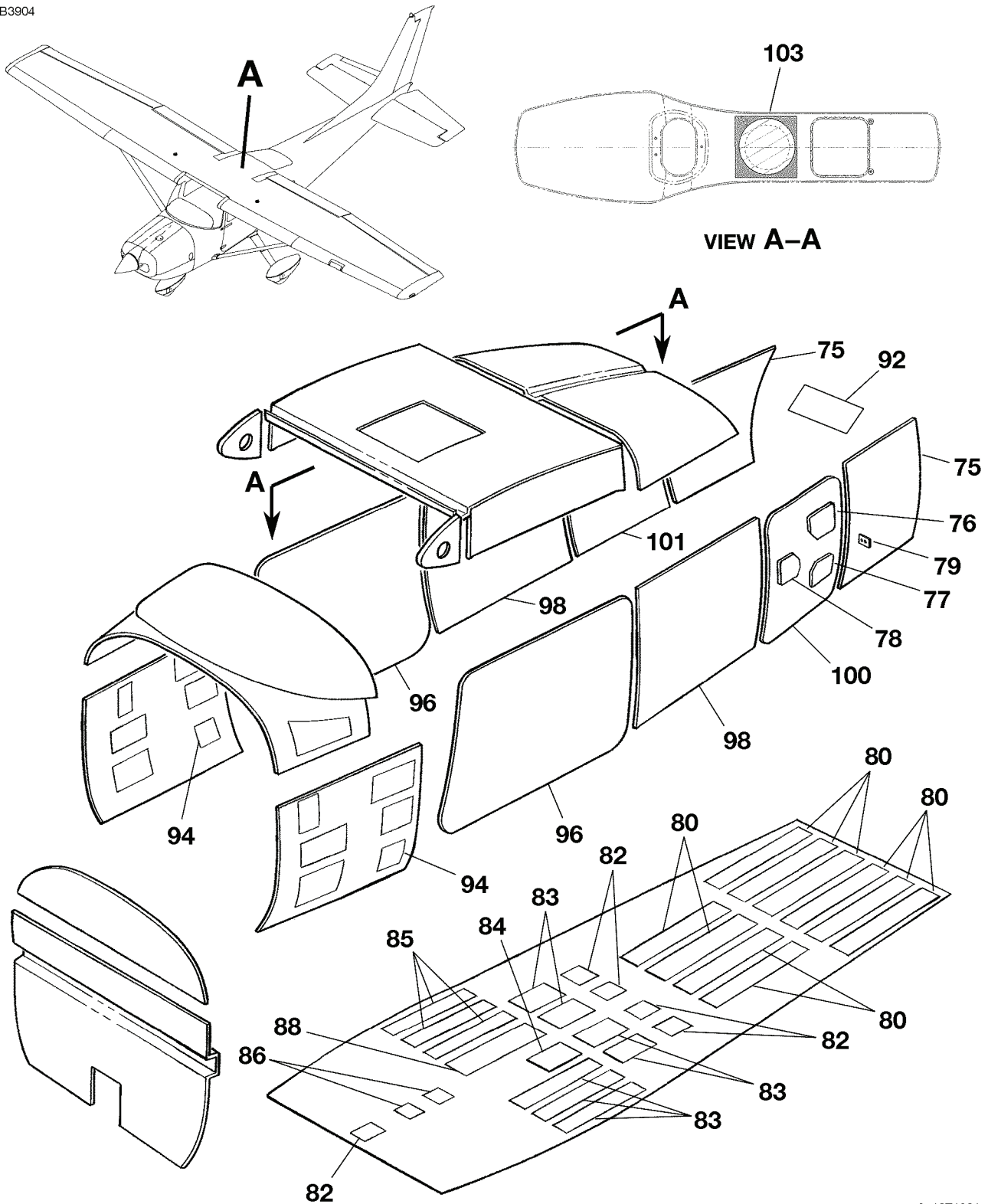
SOUNDPROOFING INSTALLATION FIGURE 01 (SHEET 2)
