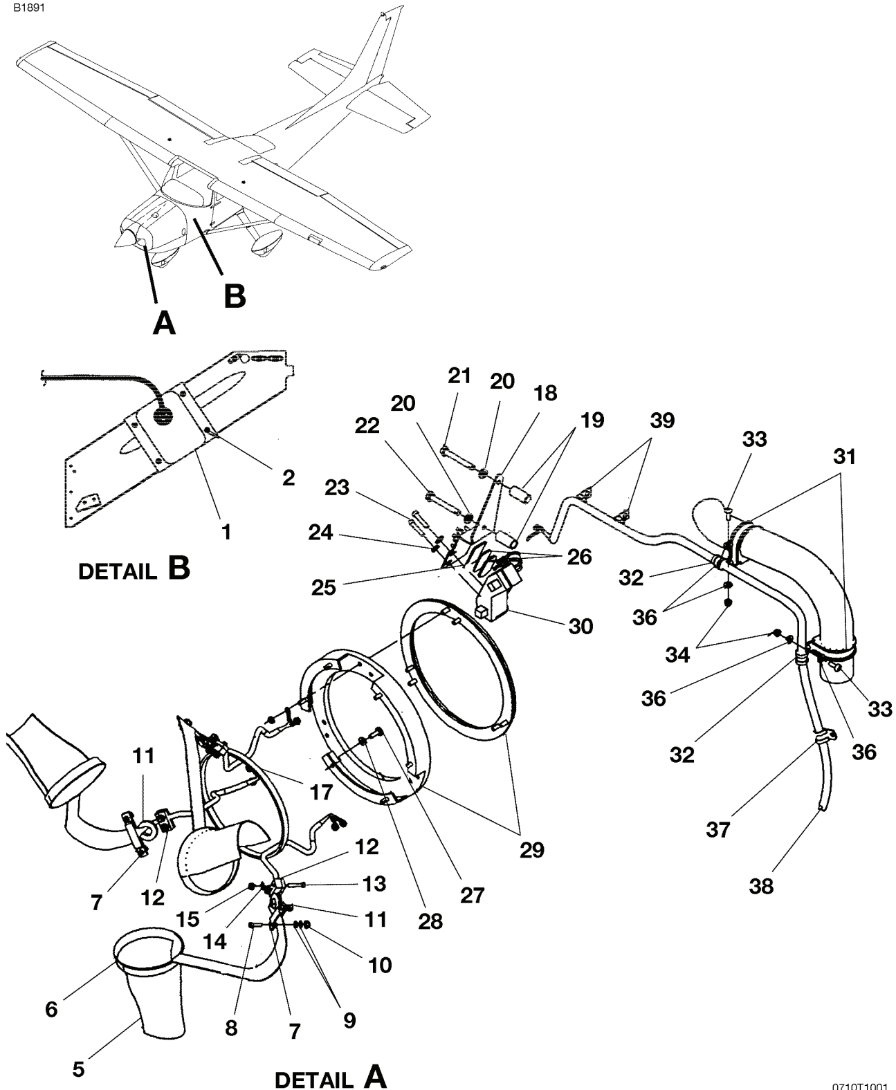
DE-ICE SYSTEM FIGURE 01 (SHEET 1)
