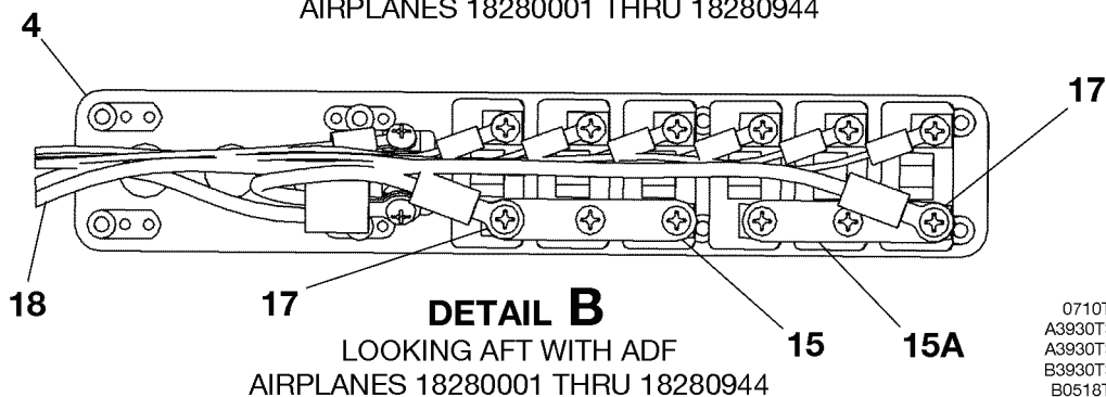
CIRCUIT BREAKER PANEL ASSEMBLY-AVIONICS - RH 182 FIGURE 02 (SHEET 1)
