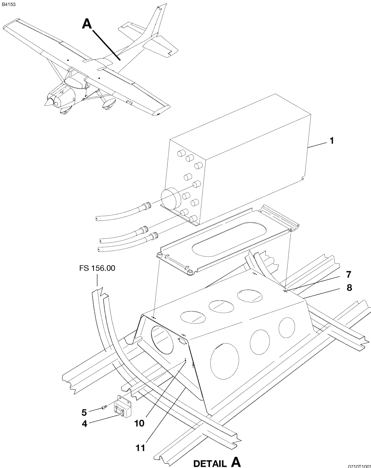
KTA-870 TRAFFIC AWARENESS SYSTEM (TAS) RECEIVER INSTALLATION FIGURE 02 (SHEET 1)
