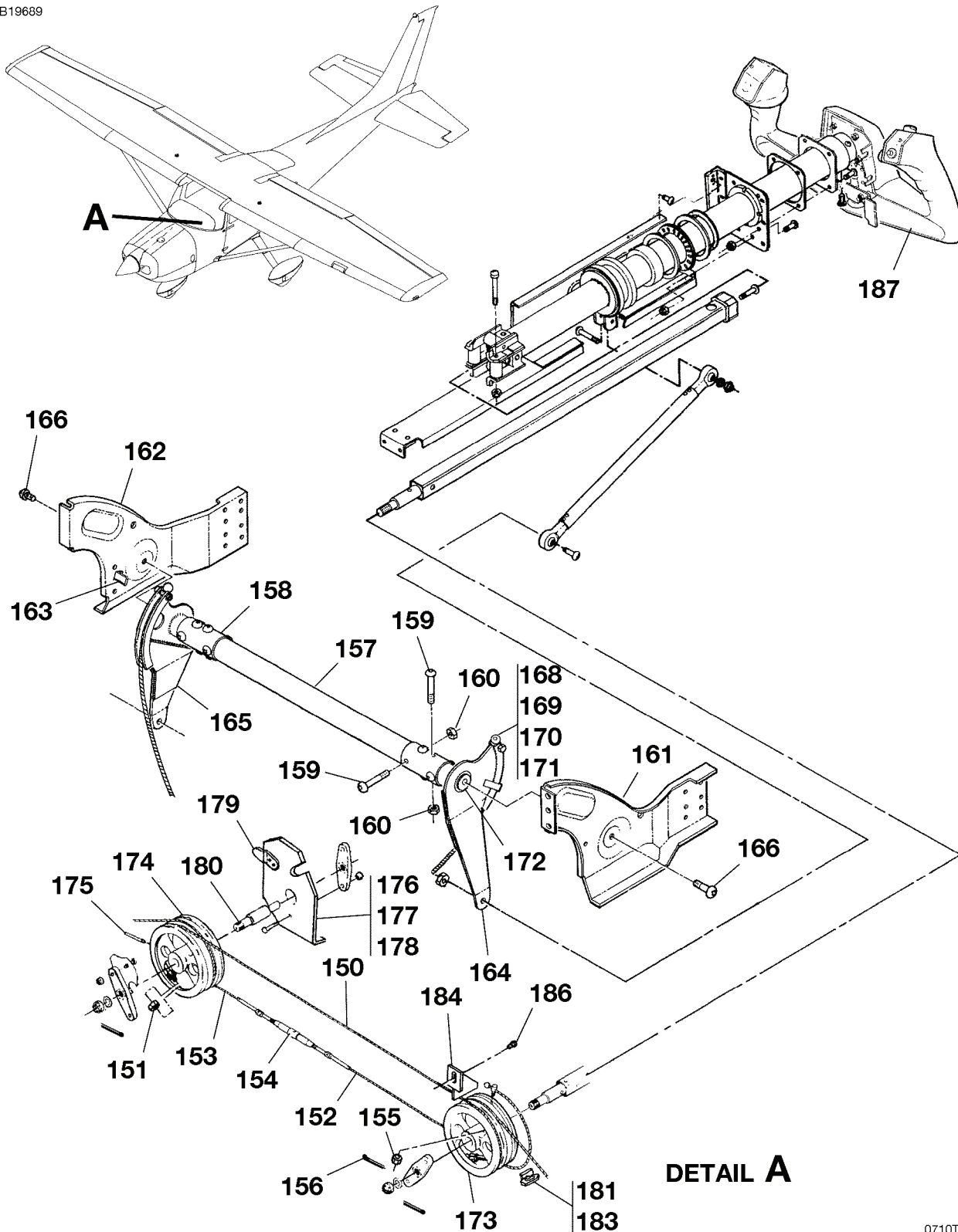
CONTROL COLUMN INSTALLATION FIGURE 01 (SHEET 3)
