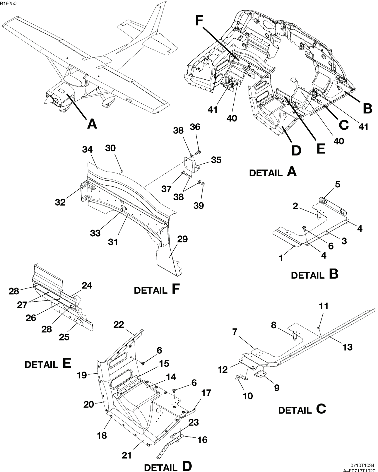
BAFFLE INSTALLATION - J182T FIGURE 03 (SHEET 1)
