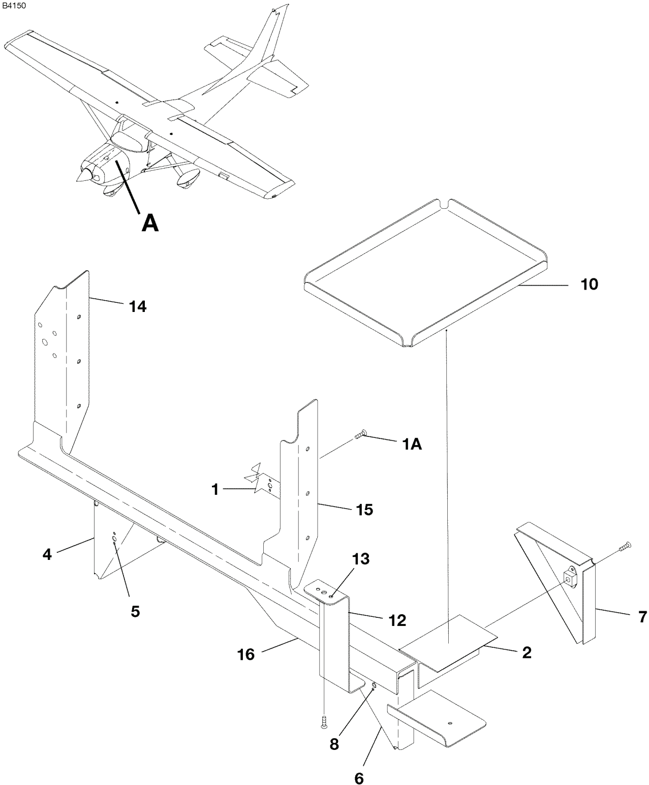
AVIONICS SUPPORT STRUCTURE - NAV III FIGURE 01 (SHEET 1)
