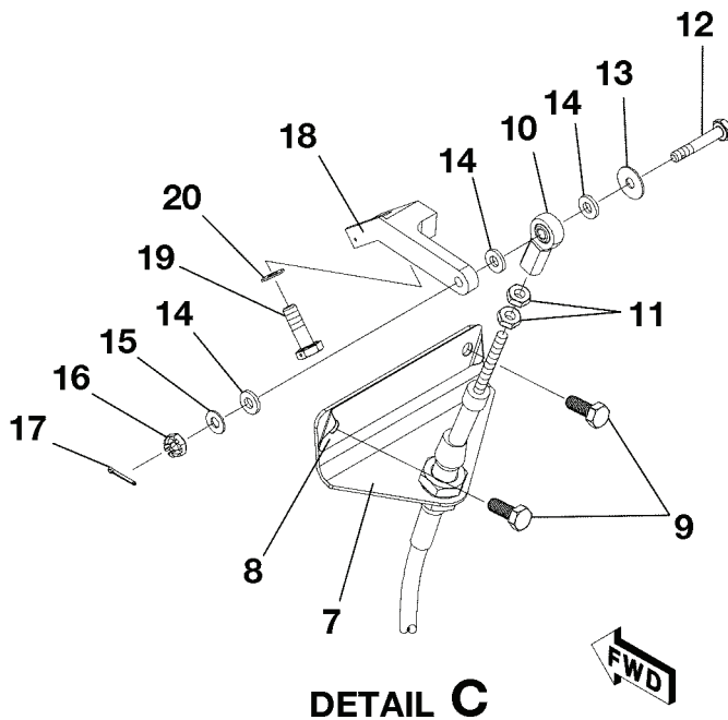
THROTTLE CONTROL INSTALLATION - J182T FIGURE 02 (SHEET 1)
