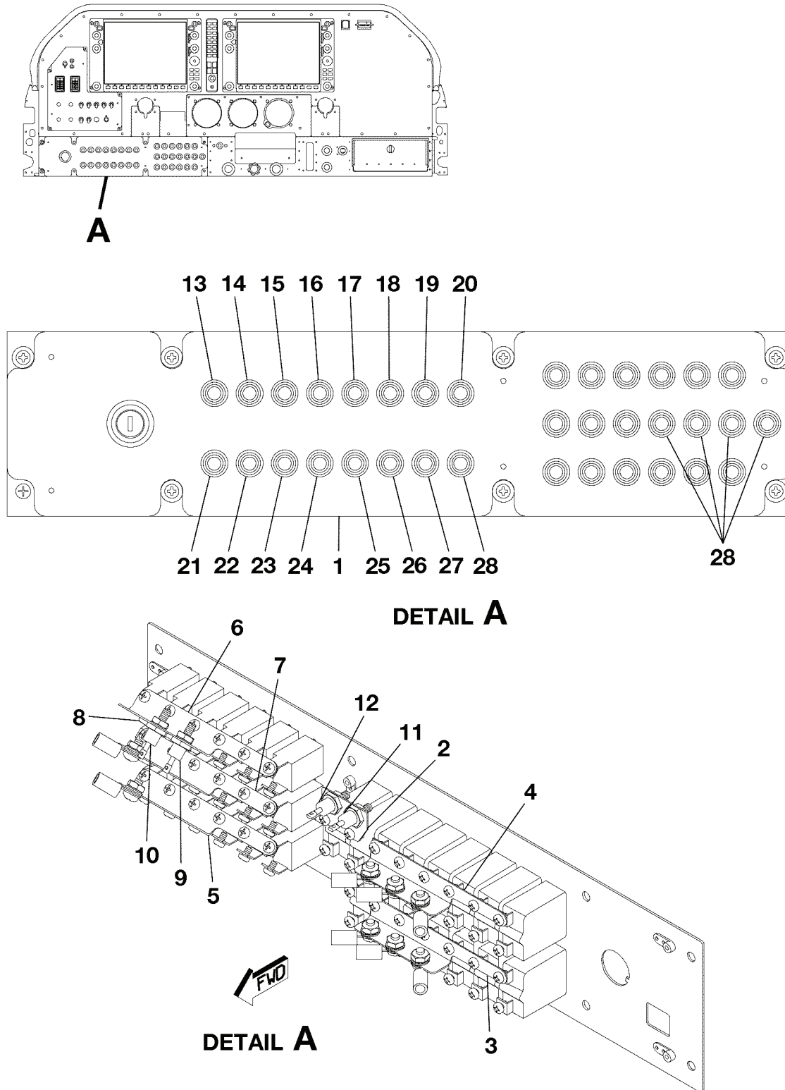
CIRCUIT BREAKER PANEL ASSEMBLY - NAV III FIGURE 01 (SHEET 1)
