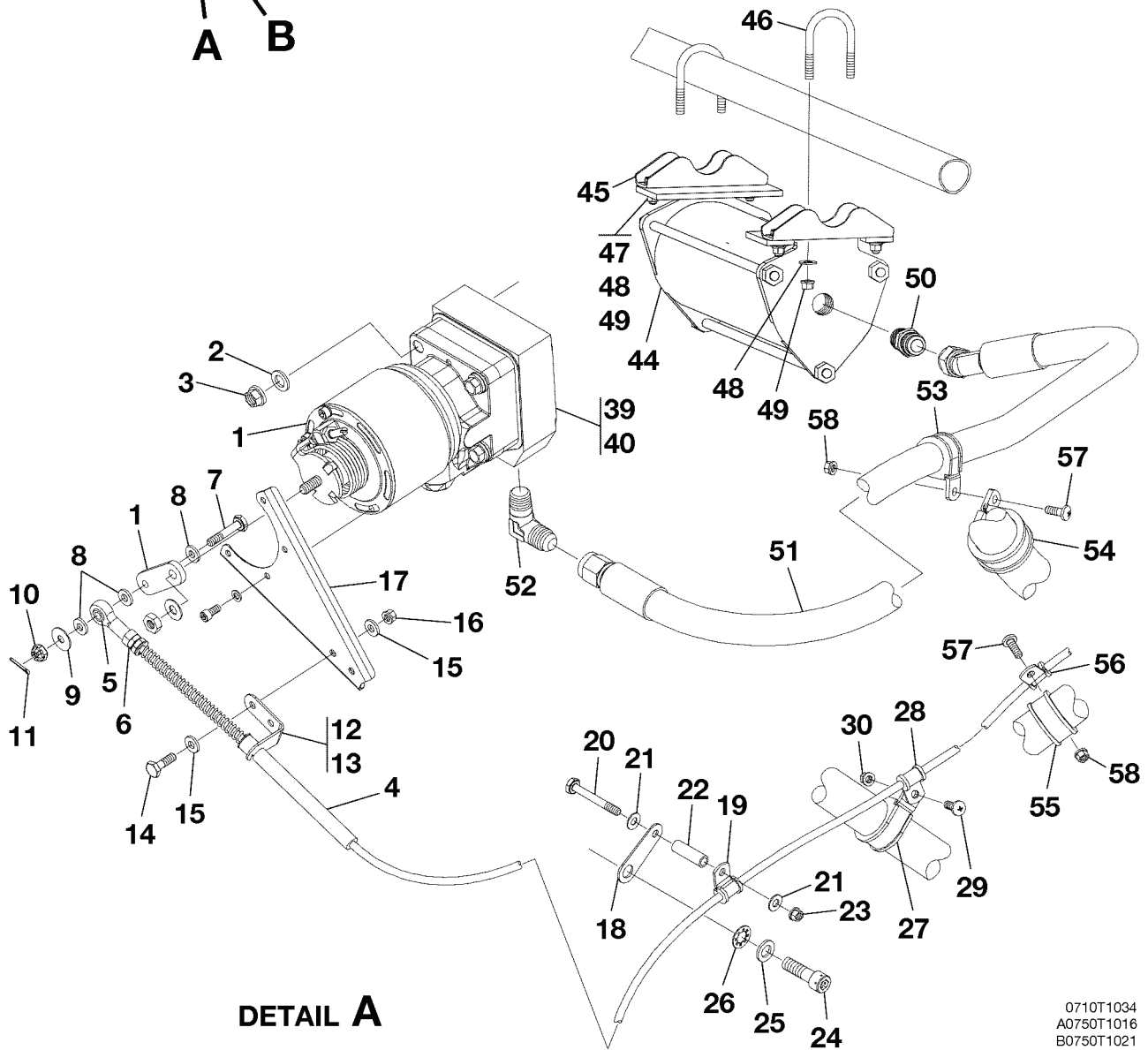
GOVERNOR INSTALLATION - PROPELLER J182T FIGURE 02 (SHEET 1)
