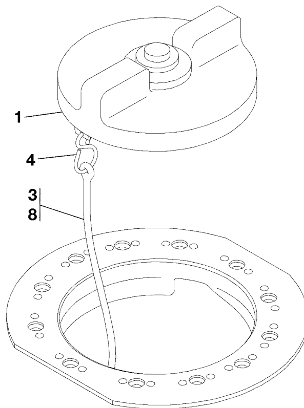
DETAIL A
