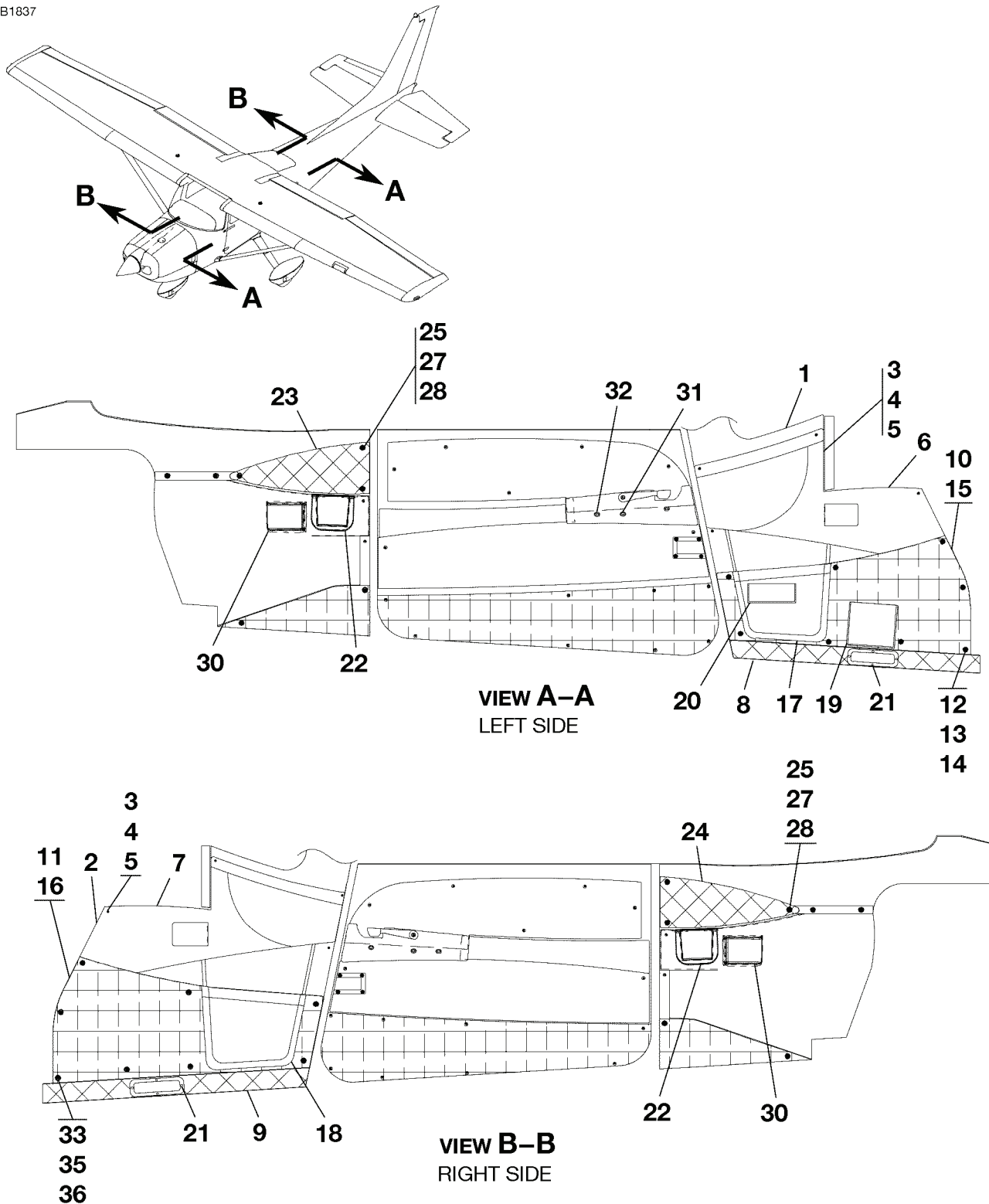
CABIN TRIM - SIDEWALLS FIGURE 01A (SHEET 1)
