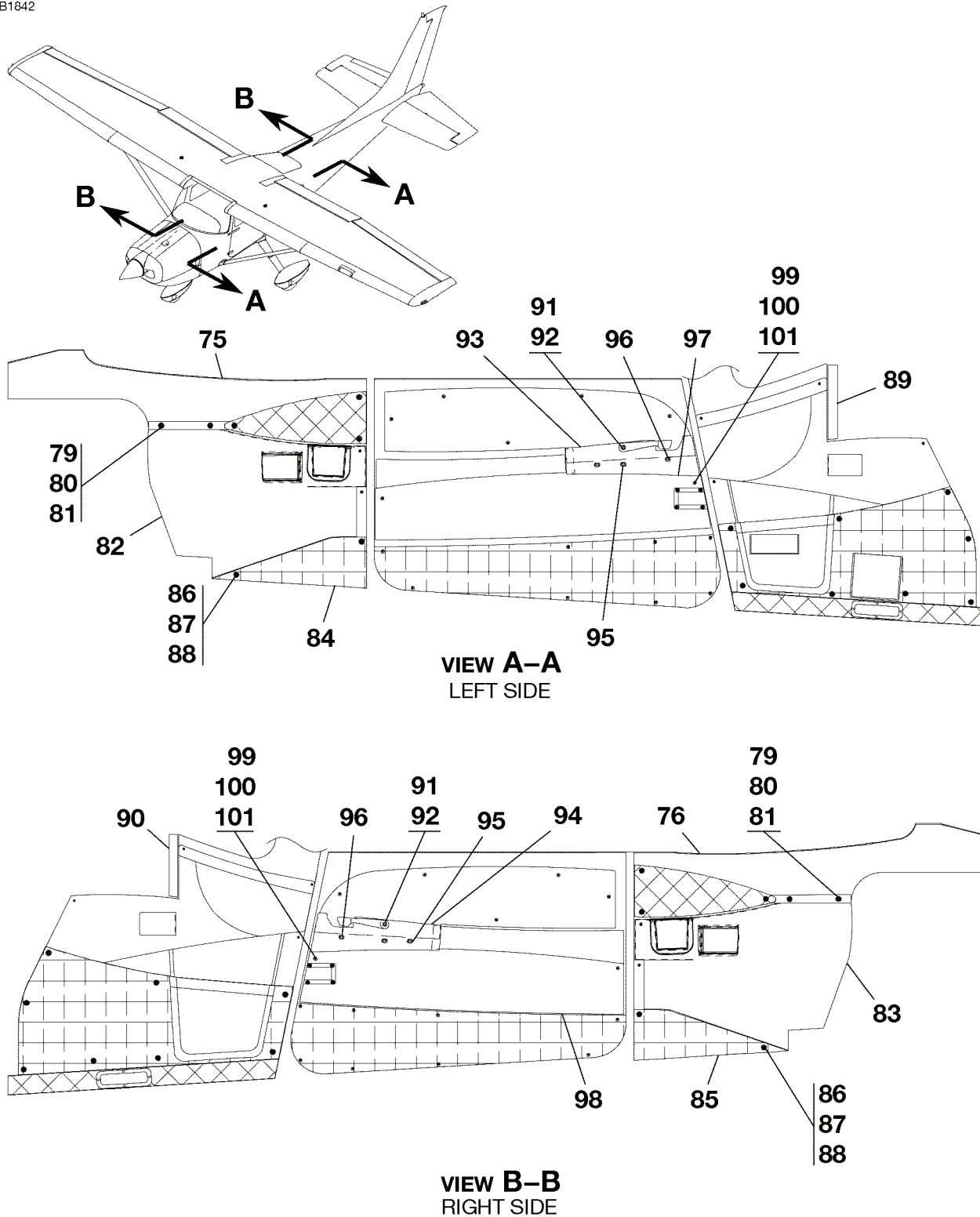
CABIN TRIM - SIDEWALLS FIGURE 01A (SHEET 2)
