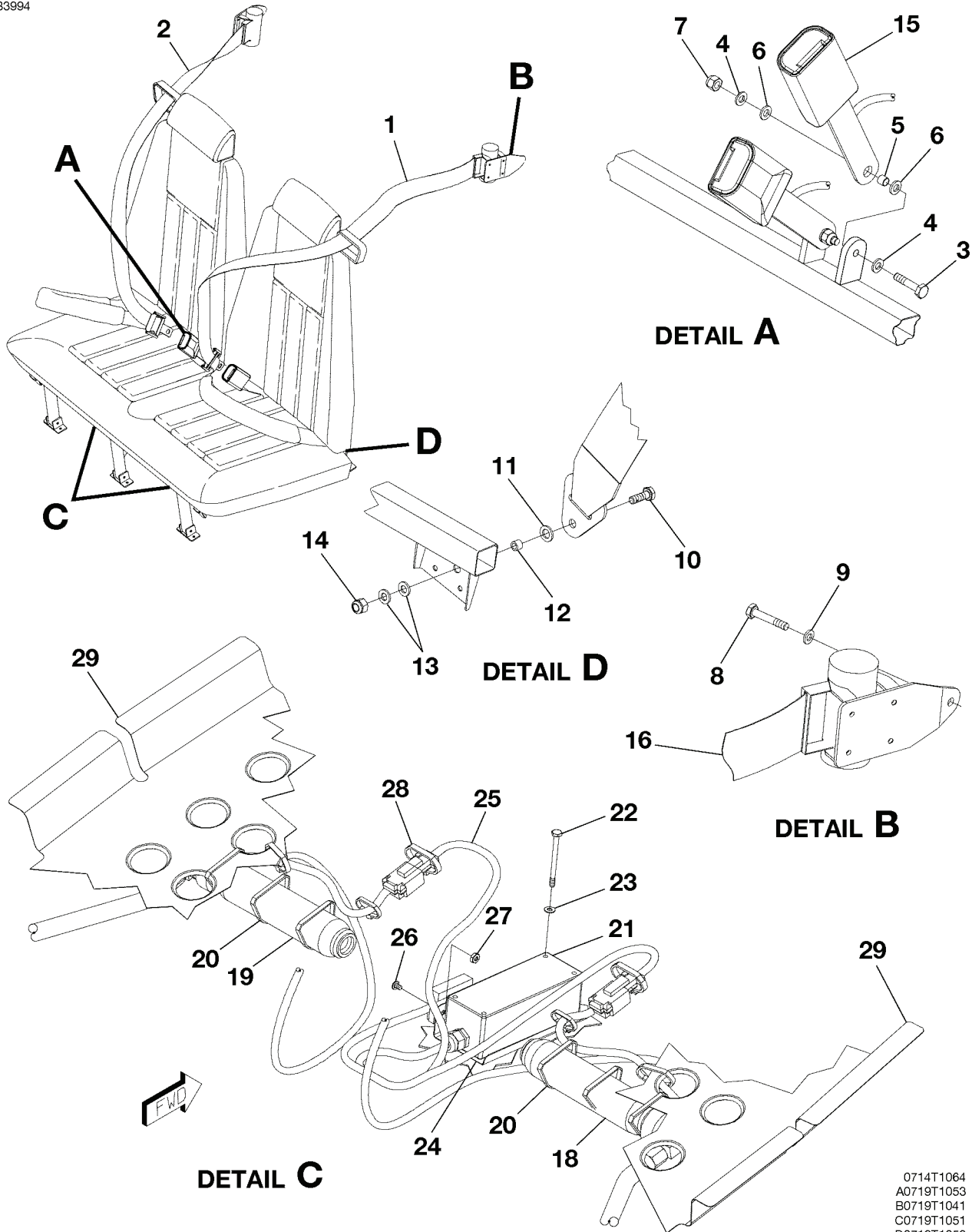
AMSAFE INFLATABLE RESTRAINT SYSTEM - AFT BENCH SEAT FIGURE 01A (SHEET 1)
