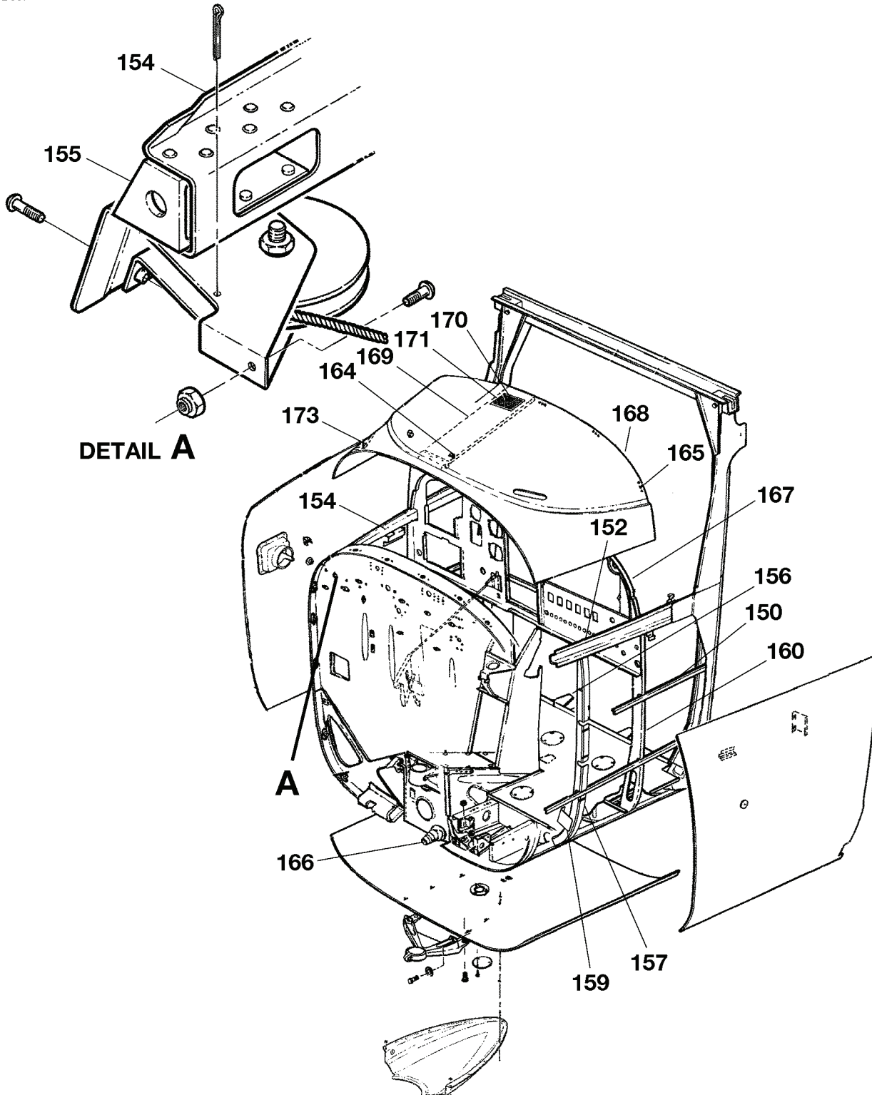
FORWARD FUSELAGE ASSEMBLY FIGURE 01 (SHEET 3)
