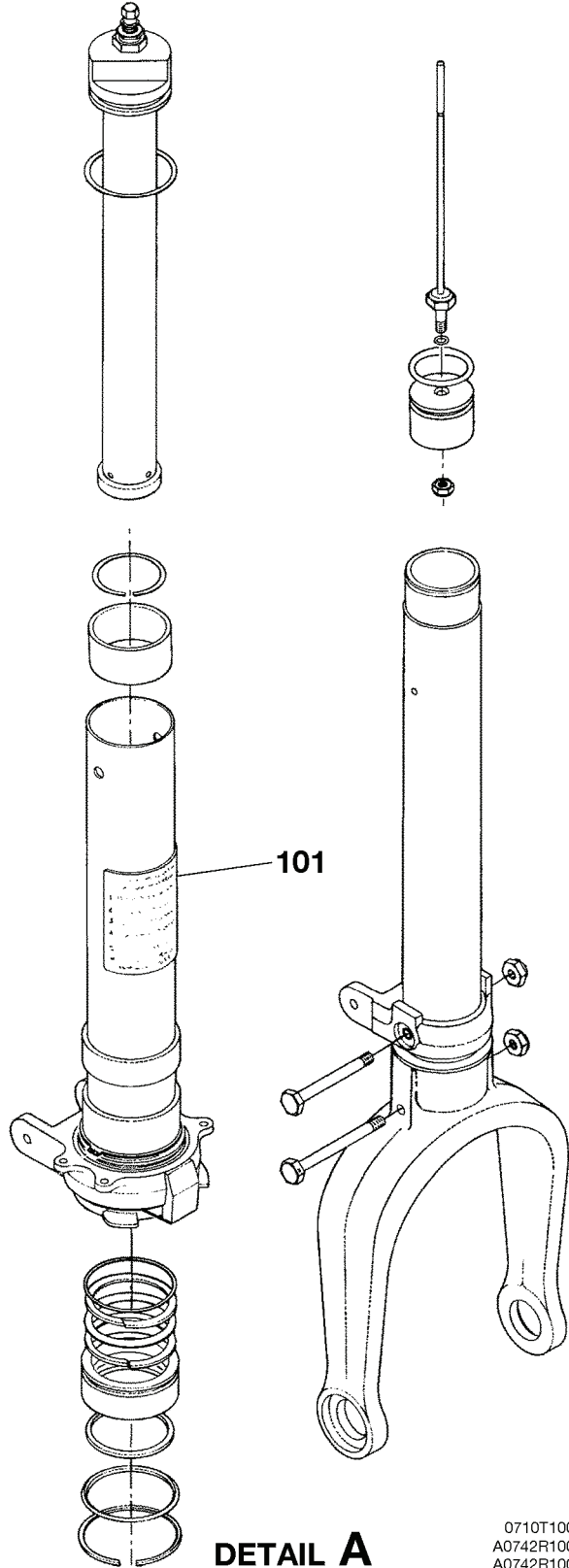
NOSE GEAR SHOCK STRUT ASSEMBLY FIGURE 01 (SHEET 2)
