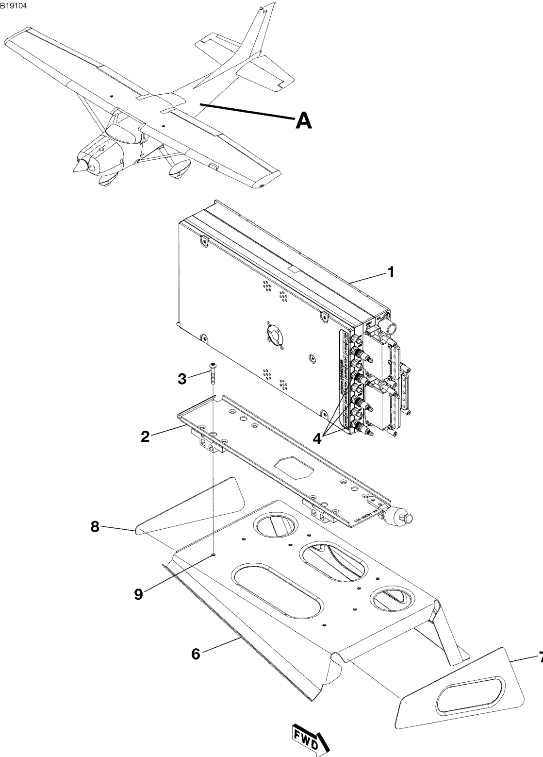
GTS 800 TRAFFIC AWARENESS SYSTEM (TAS) INSTALLATION FIGURE 02A (SHEET 1)
