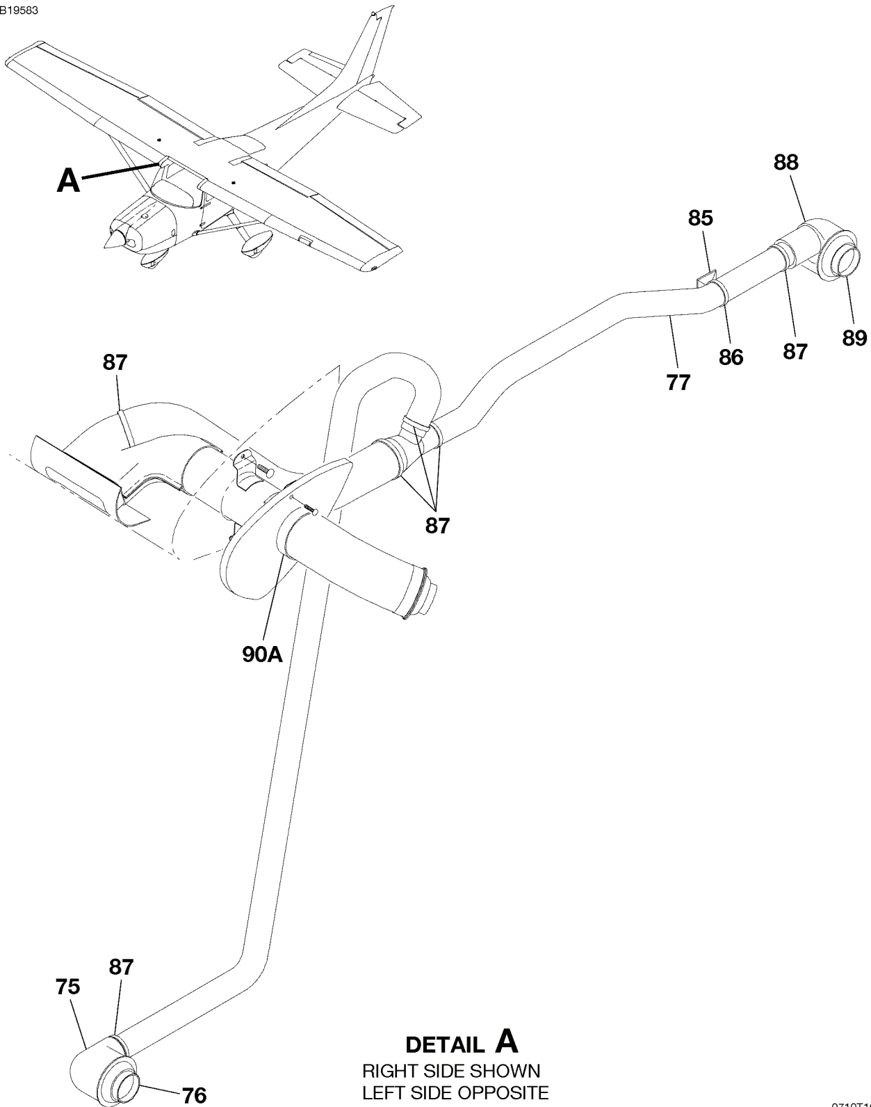
CABIN VENTILATION SYSTEM FIGURE 01 (SHEET 2)
