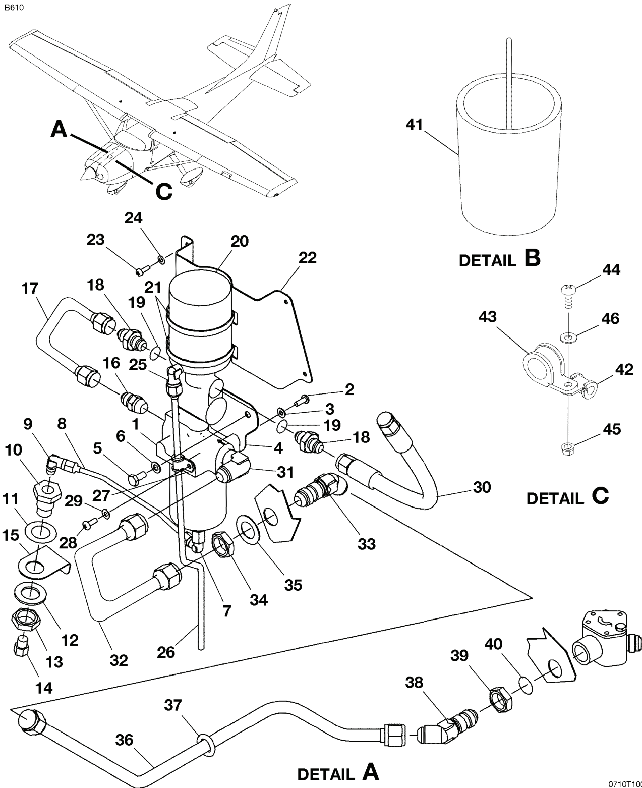
FUEL SYSTEM - 182 FIGURE 01 (SHEET 1)
