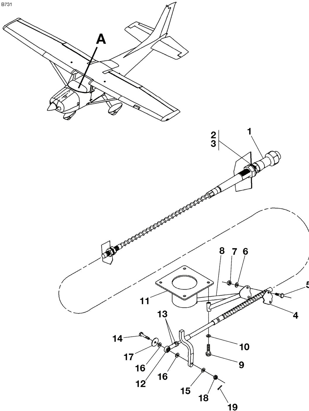
DETAIL A
