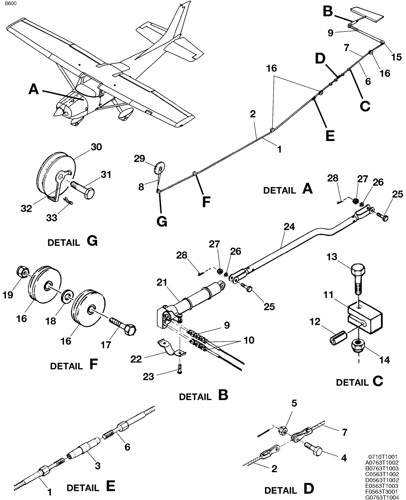
ELEVATOR TRIM CONTROL SYSTEM FIGURE 01 (SHEET 1)
