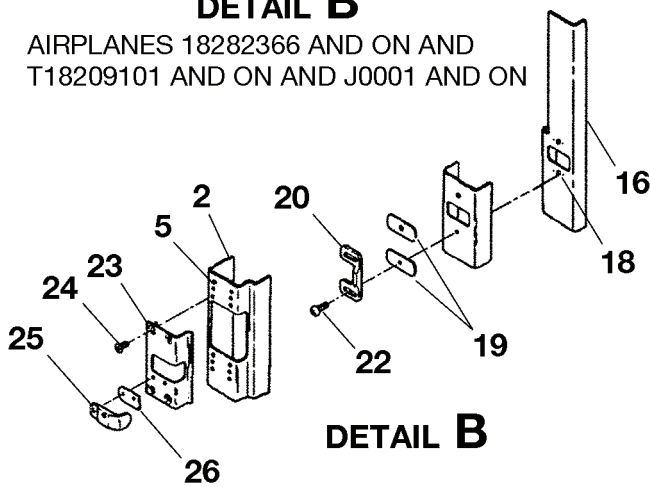
REAR DOORPOST BULKHEAD ASSEMBLY FIGURE 02 (SHEET 1)
