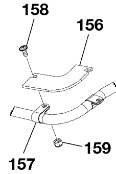
DETAIL B
