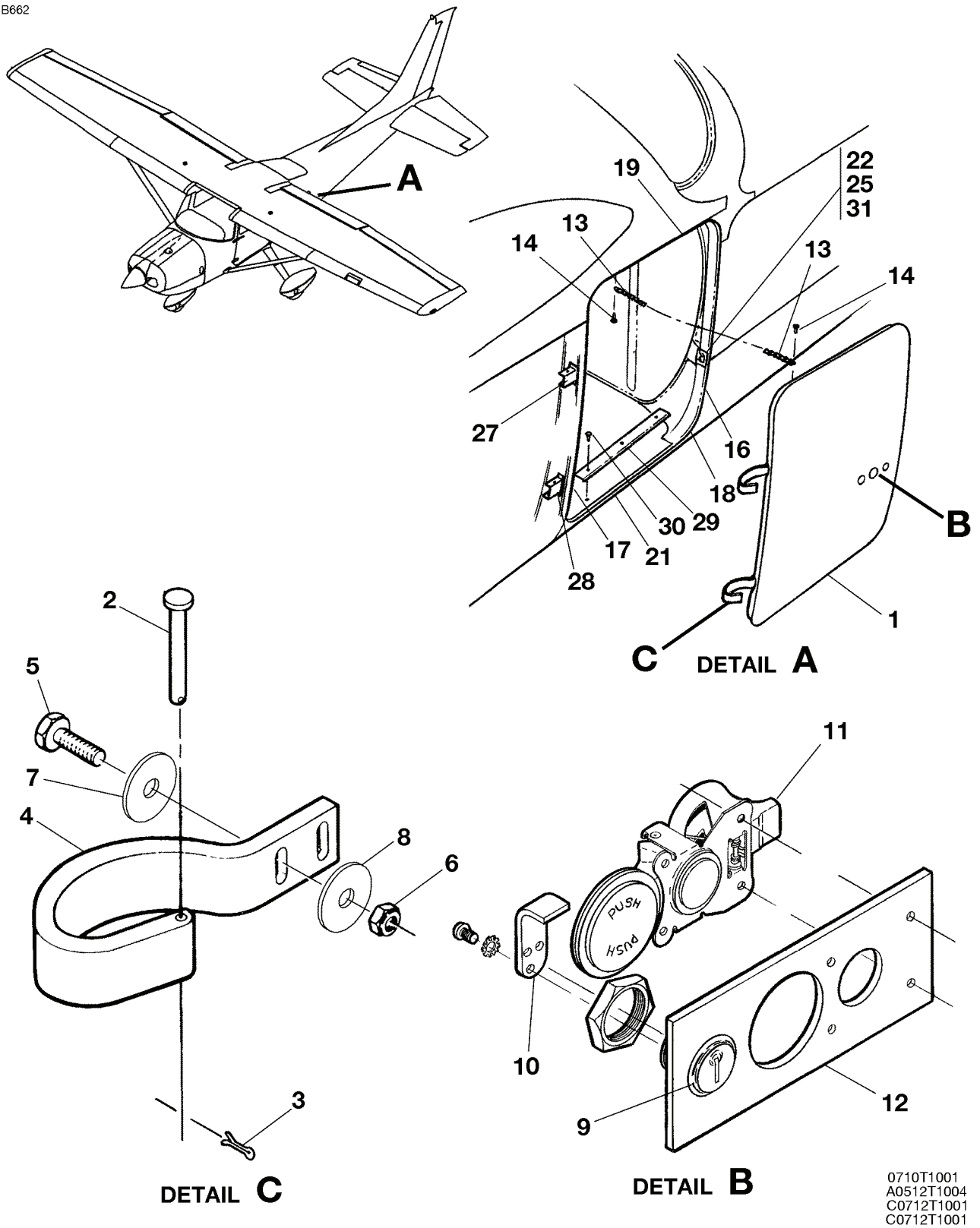
BAGGAGE DOOR INSTALLATION FIGURE 01 (SHEET 1)
