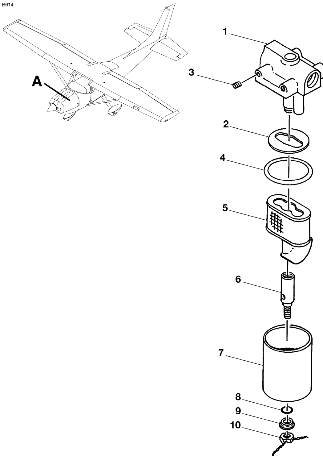
DETAIL A
