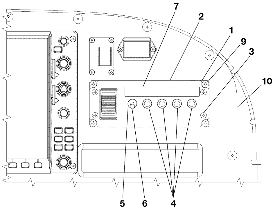
DETAIL B
