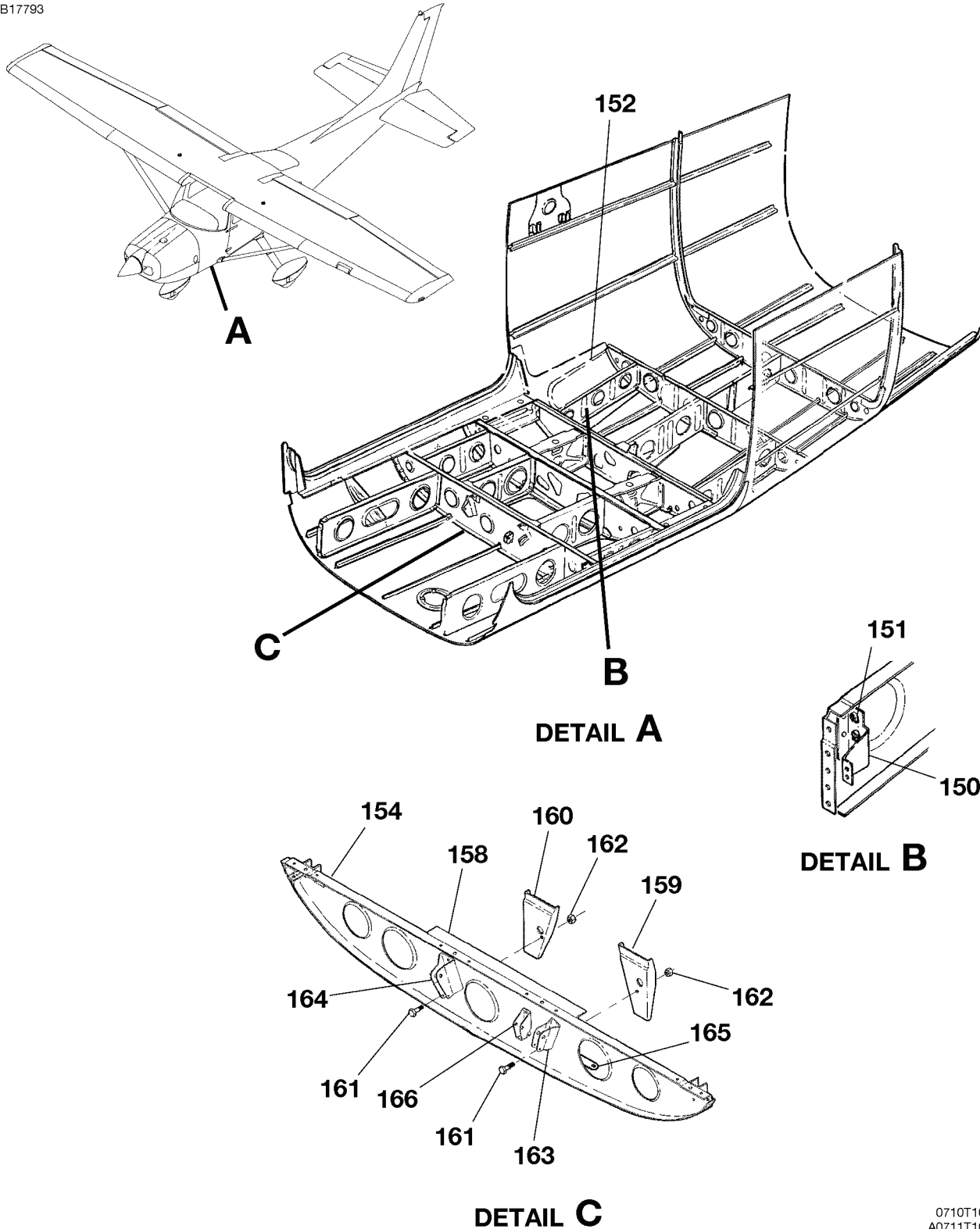
LOWER CABIN SECTION ASSEMBLY FIGURE 01 (SHEET 3)
