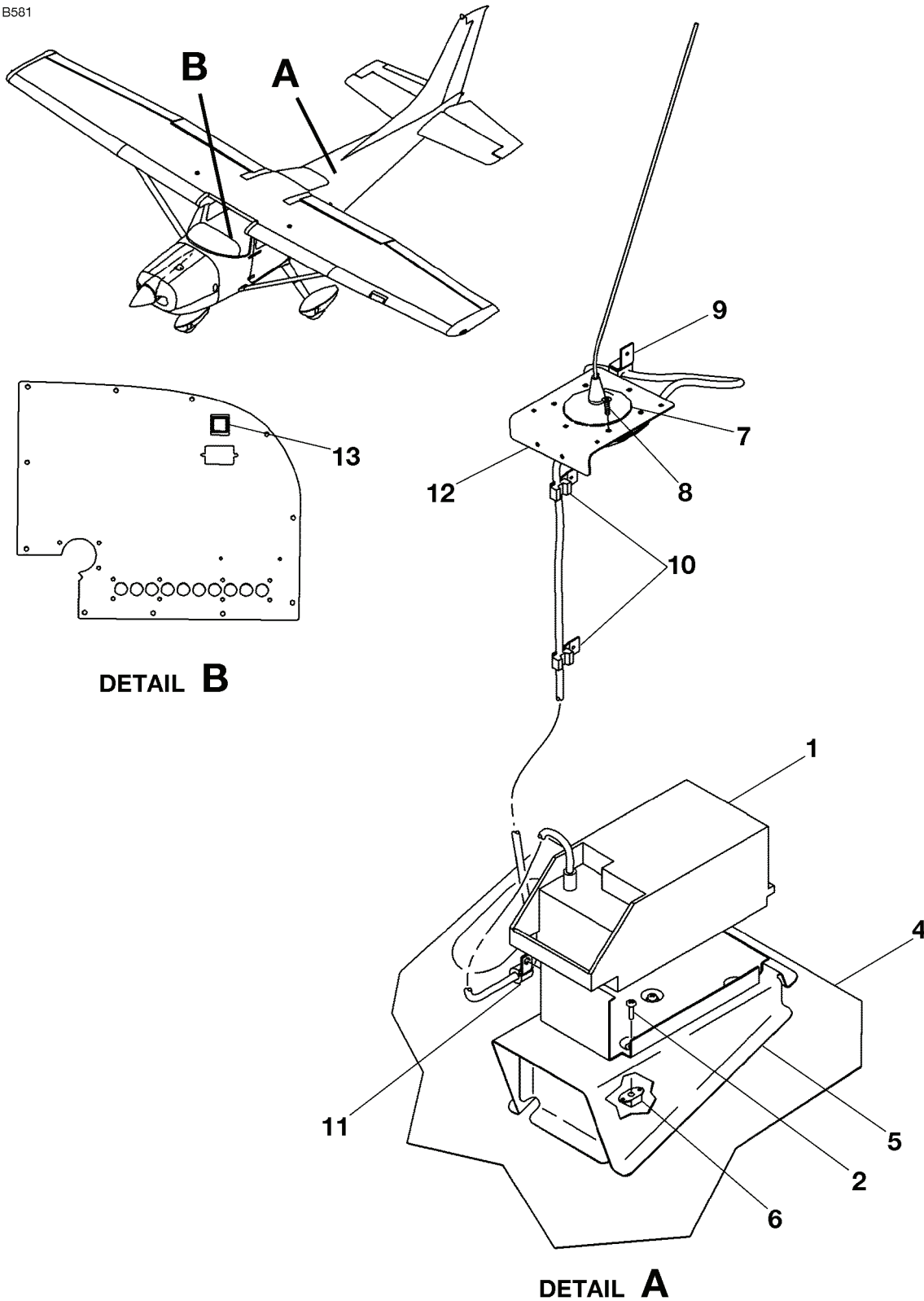
EMERGENCY LOCATOR TRANSMITTER INSTALLATION FIGURE 01 (SHEET 1)
