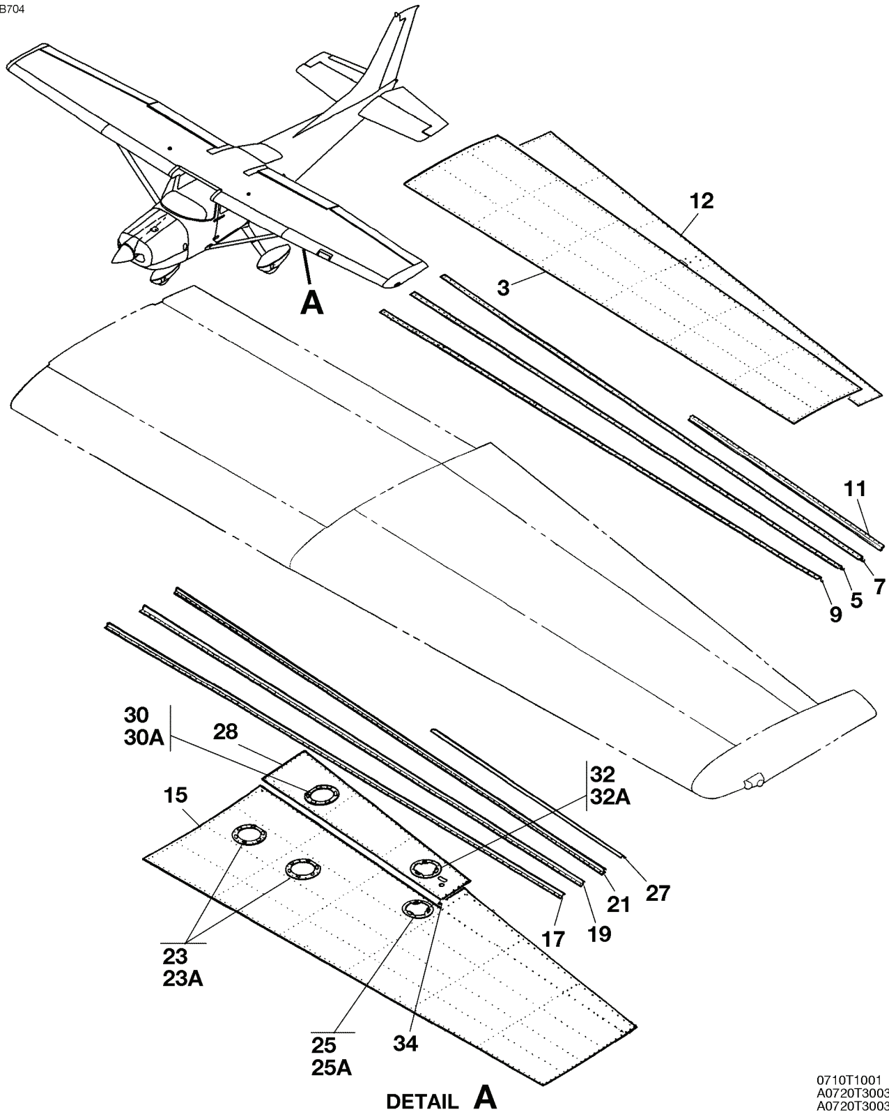
SKINS AND STRINGERS INSTALLATION - WING FIGURE 01 (SHEET 1)
