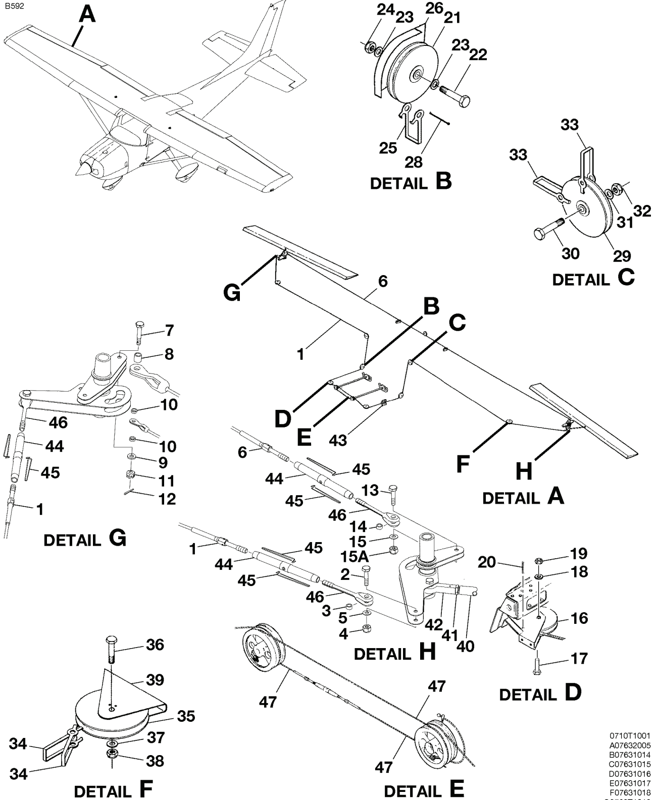
AILERON CONTROL SYSTEM INSTALLATION FIGURE 03 (SHEET 1)
