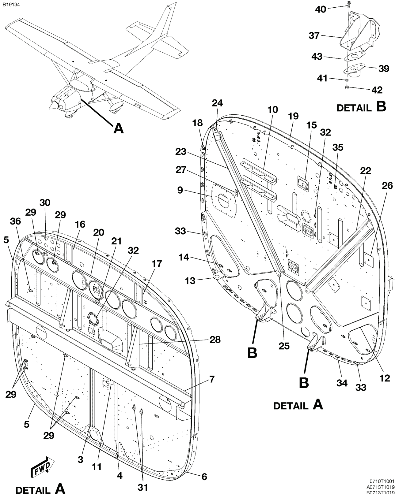
FIREWALL ASSEMBLY - J182T FIGURE 01A (SHEET 1)
