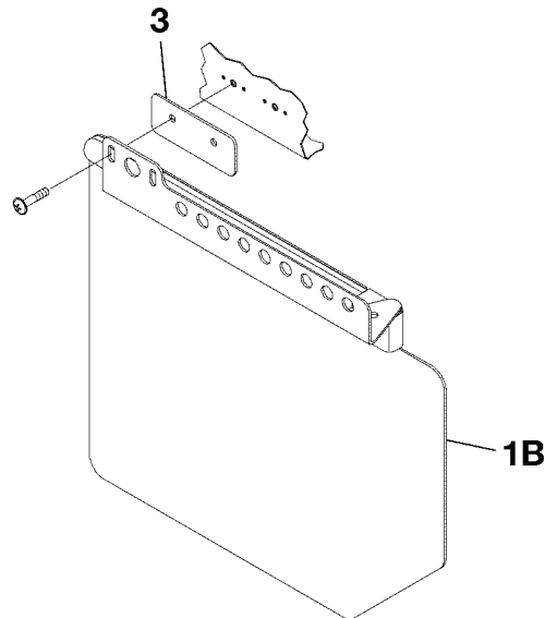
DETAIL A
