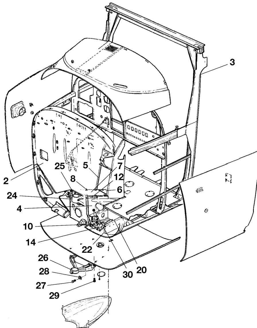
FORWARD FUSELAGE ASSEMBLY FIGURE 01 (SHEET 1)
