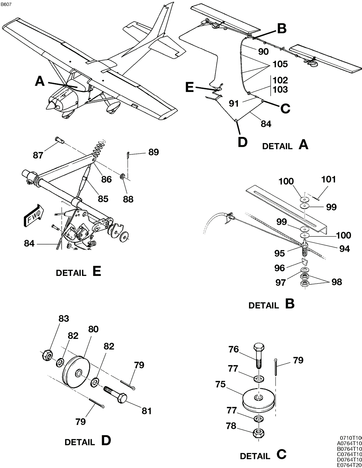
FLAP POSITION INDICATOR INSTALLATION FIGURE 02 (SHEET 2)
