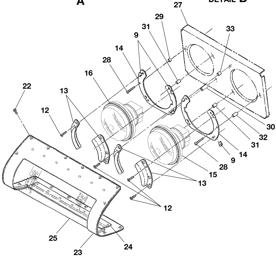
DETAIL A
