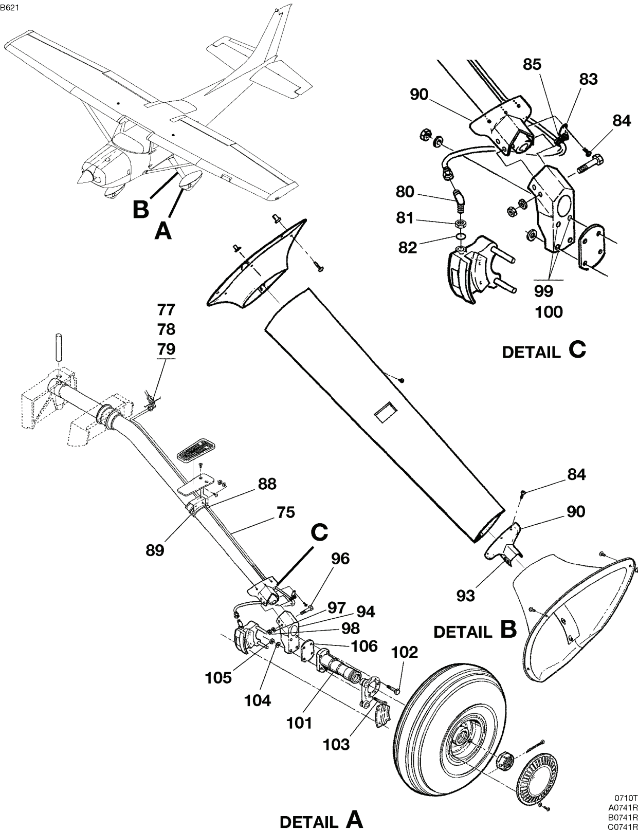
MAIN LANDING GEAR INSTALLATION FIGURE 01 (SHEET 2)
