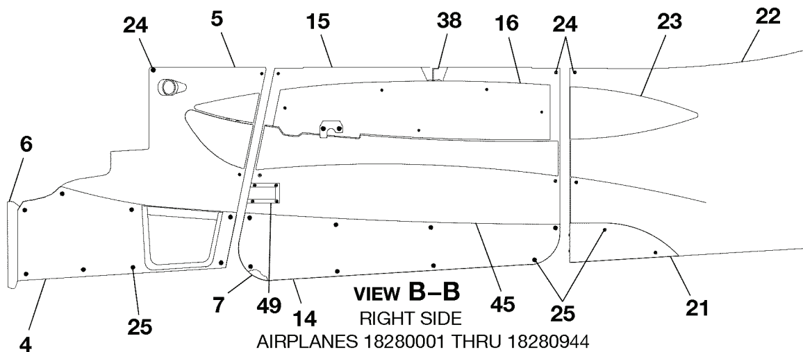
CABIN TRIM FIGURE 01 (SHEET 1)
