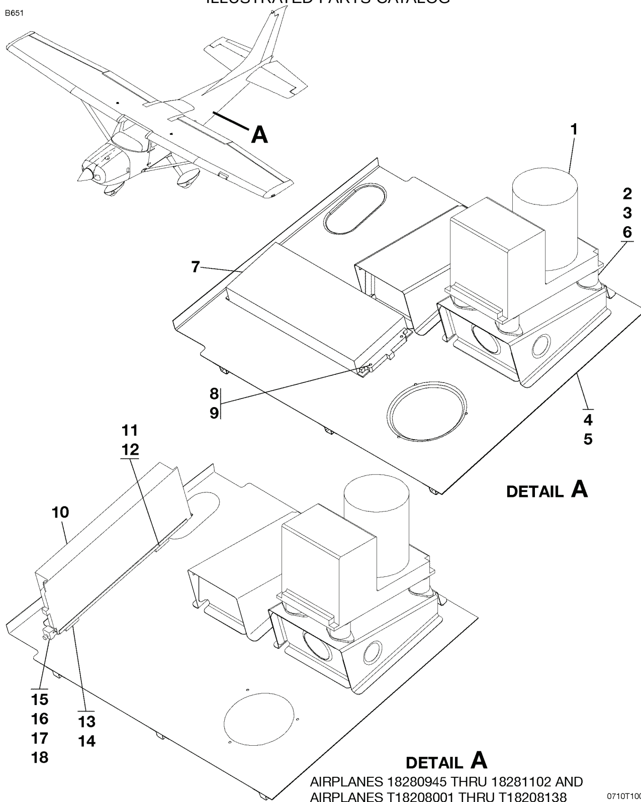
HORIZONTAL SITUATION INDICATOR (HSI) INSTALLATION - NAV CONVERTER & DIRECTIONAL GYRO FIGURE 02 (SHEET 1)
