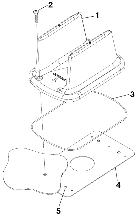
DETAIL A
