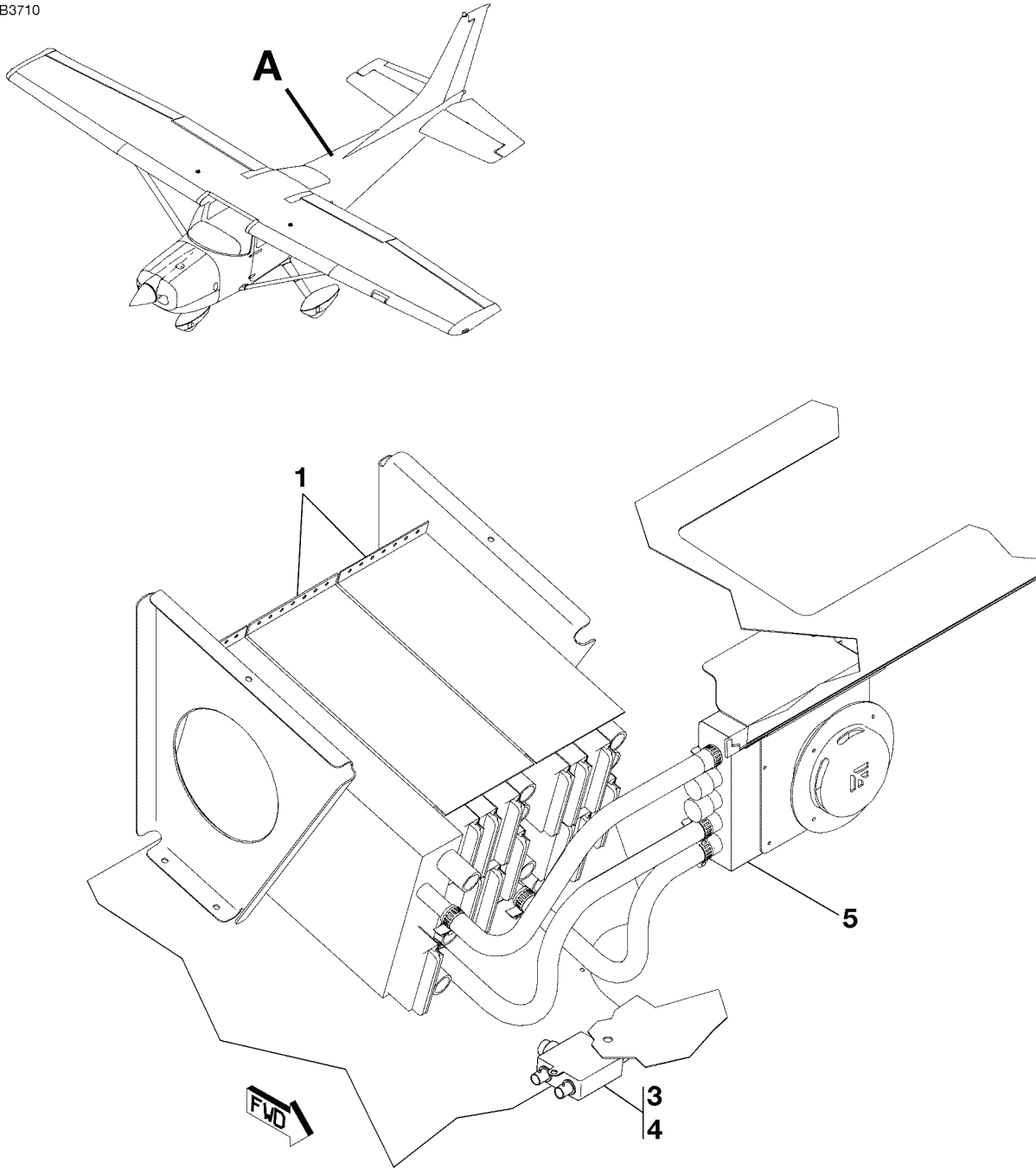
DETAIL A
