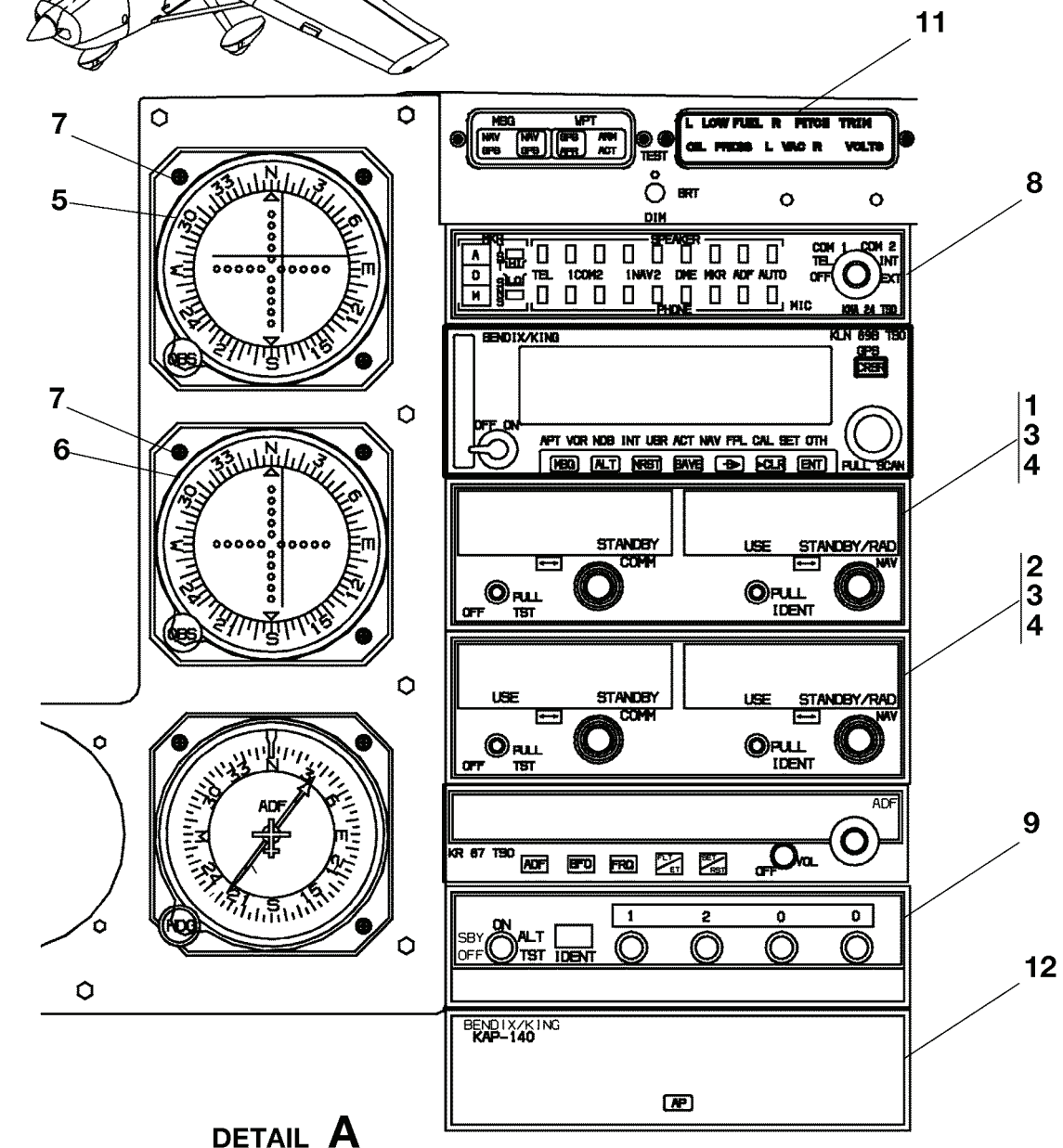
VHF NAVIGATION SYSTEM - BASIC FIGURE 01 (SHEET 1)
