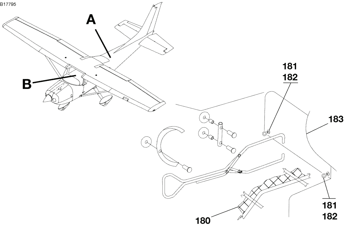
DETAIL A
