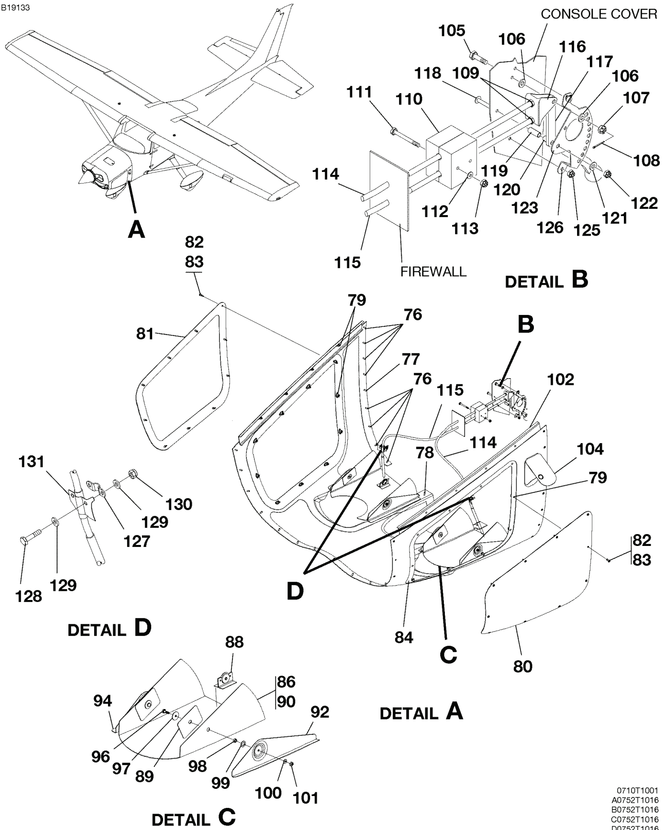
ENGINE COWL ASSEMBLY - J182T FIGURE 01A (SHEET 2)
