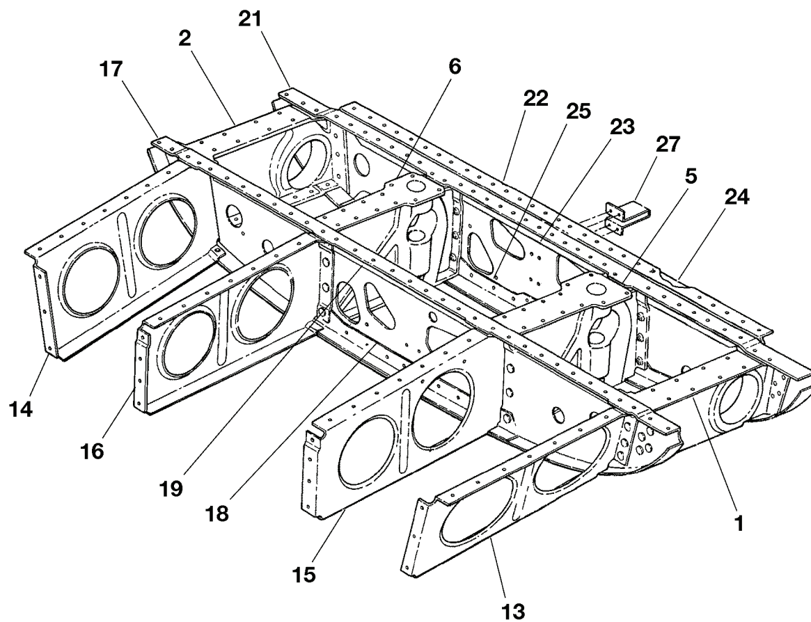
DETAIL A
