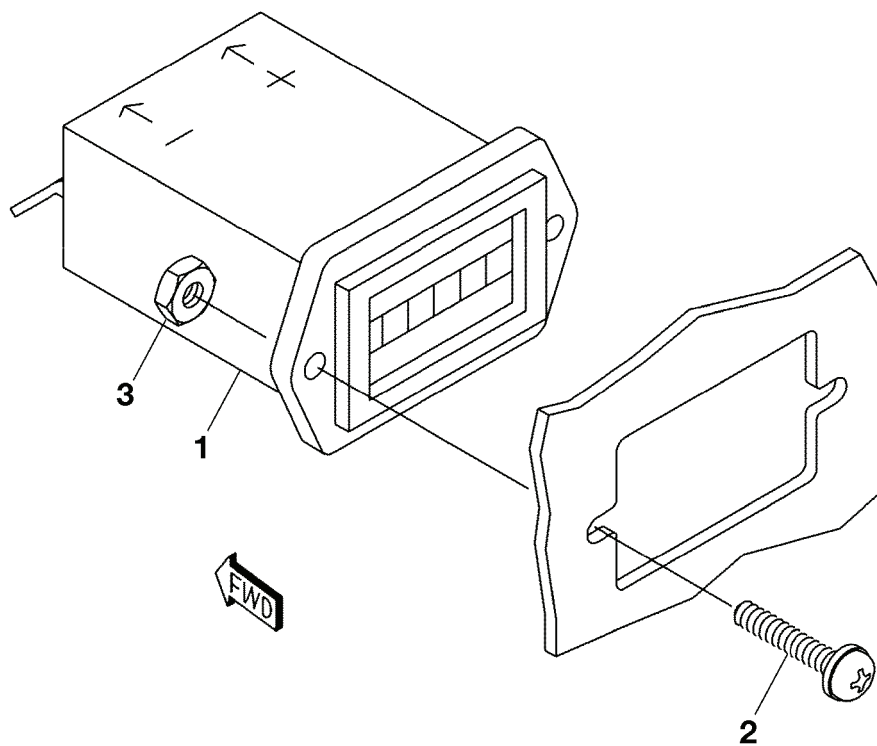
DETAIL A
