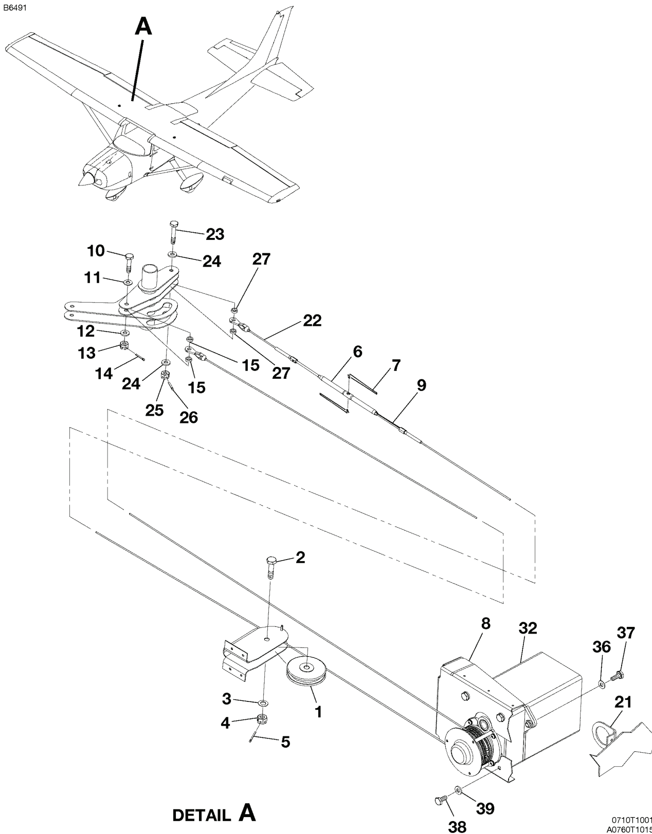
ROLL SERVO INSTALLATION - NAV III FIGURE 04 (SHEET 1)
