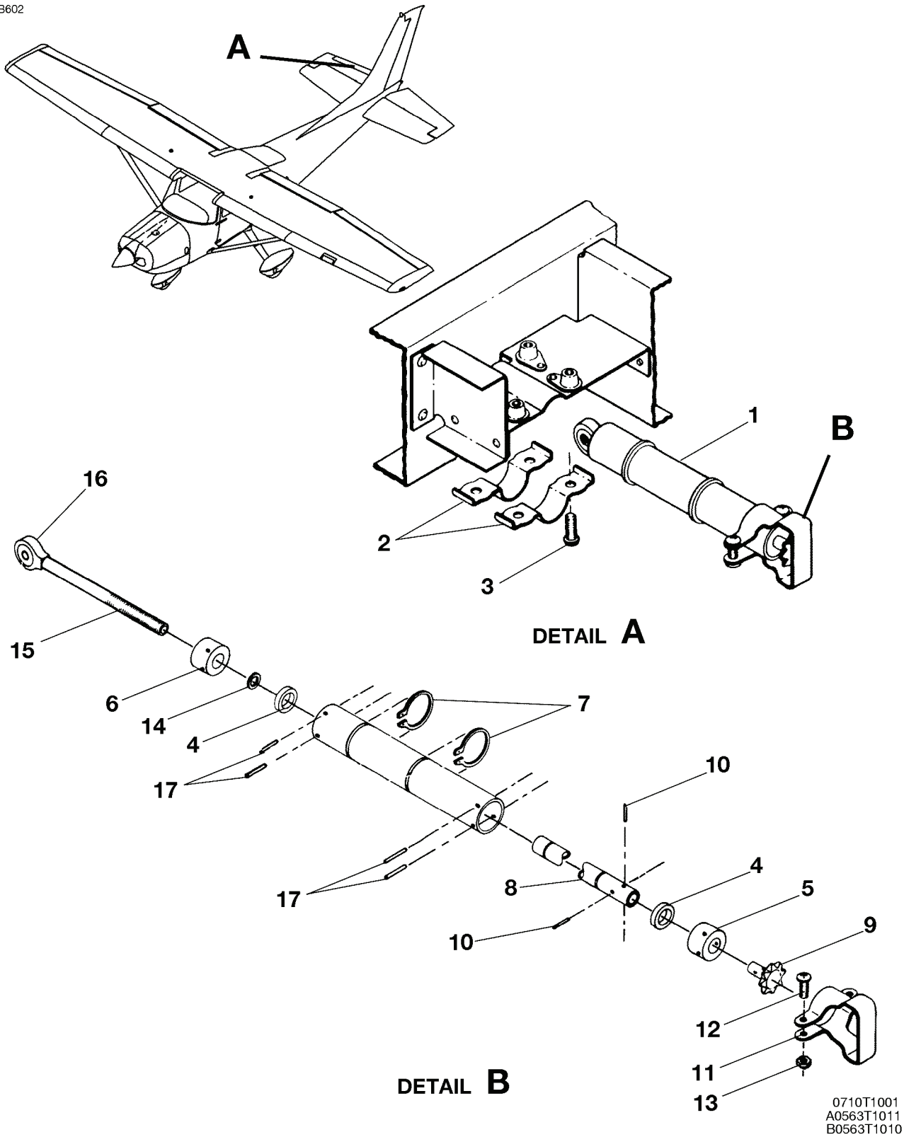
ELEVATOR TRIM TAB ACTUATOR ASSEMBLY FIGURE 02 (SHEET 1)
