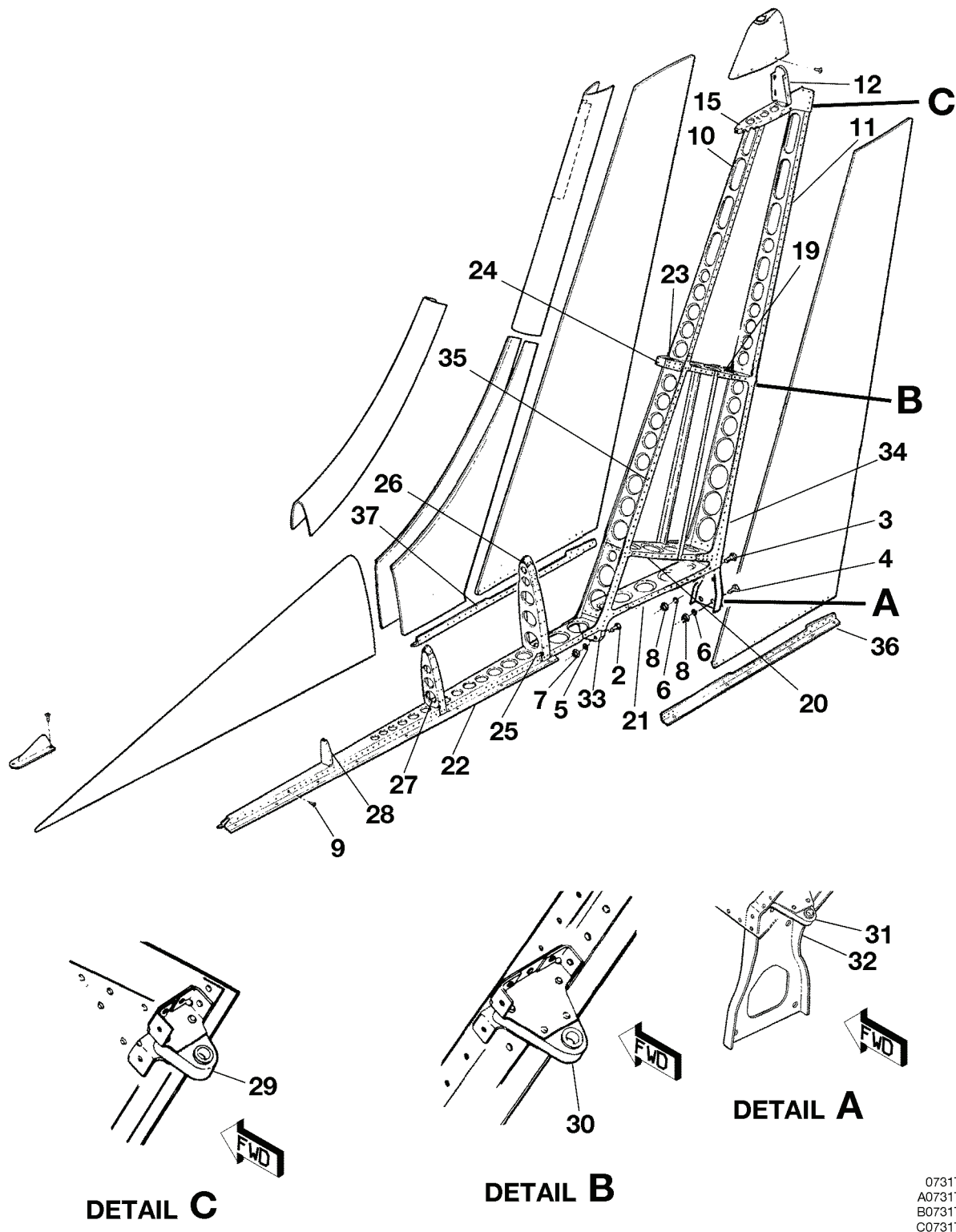
FIN AND DORSAL INSTALLATION FIGURE 01 (SHEET 1)
