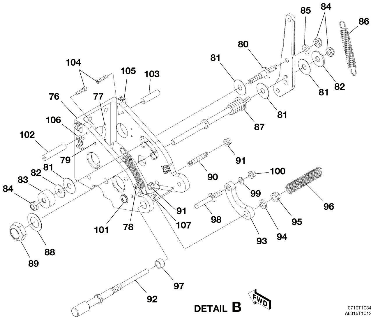
THROTTLE QUADRANT INSTALLATION - J182T FIGURE 01 (SHEET 2)
