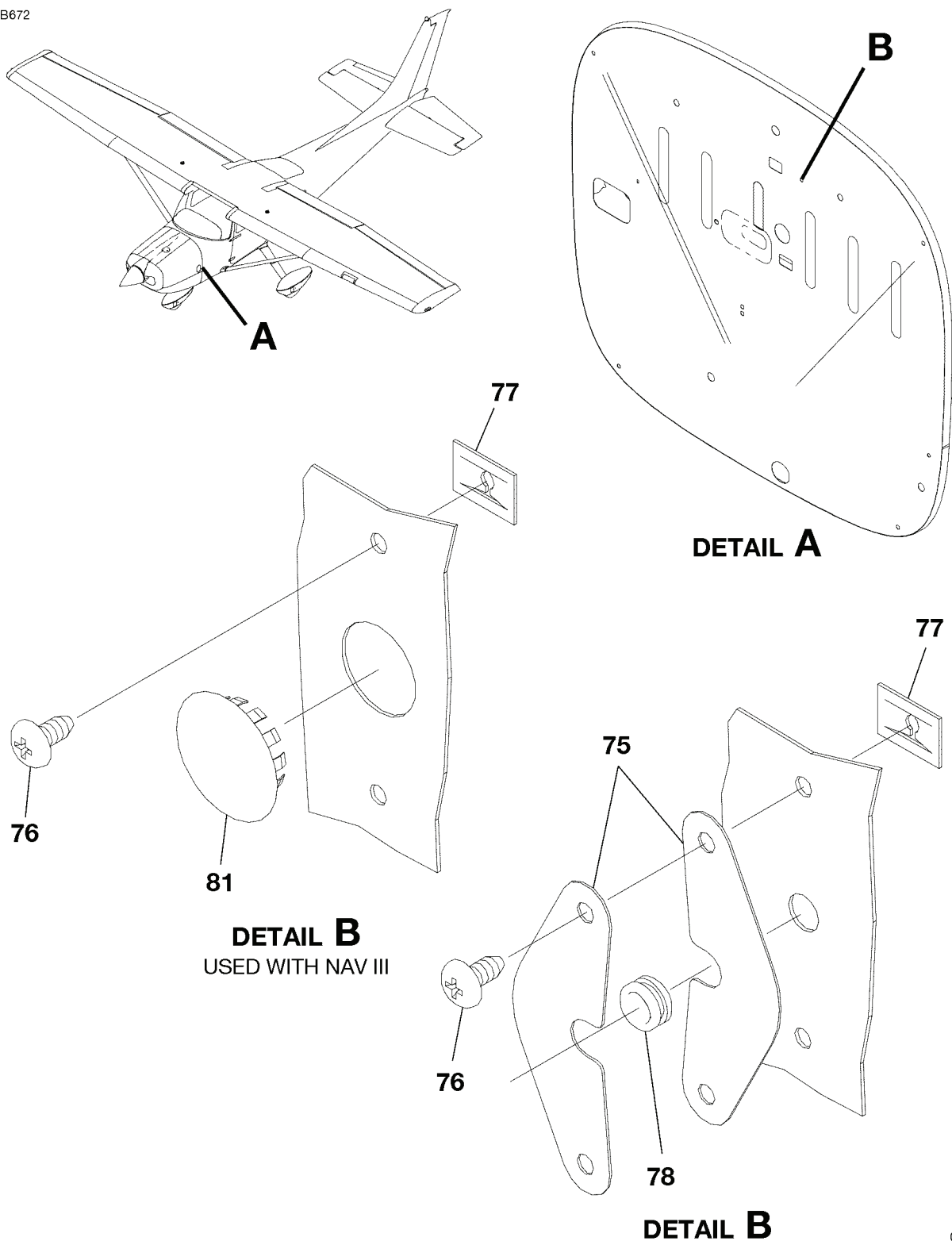
FIREWALL ASSEMBLY FIGURE 01 (SHEET 2)
