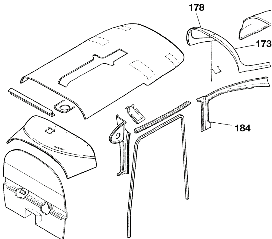
DETAIL A
