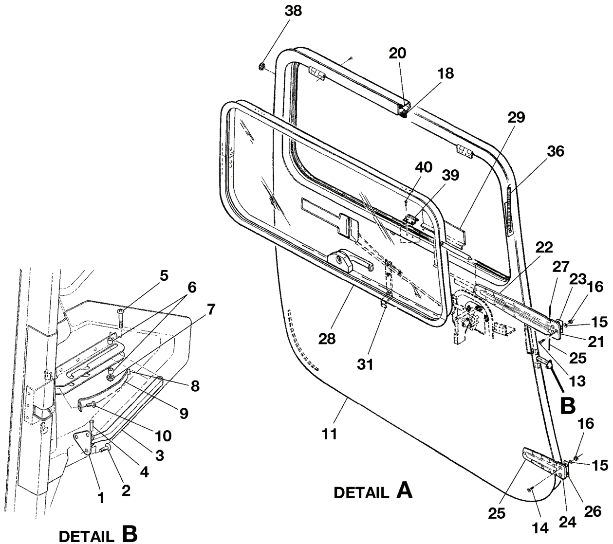
CABIN DOOR INSTALLATION - RH FIGURE 02 (SHEET 1)
