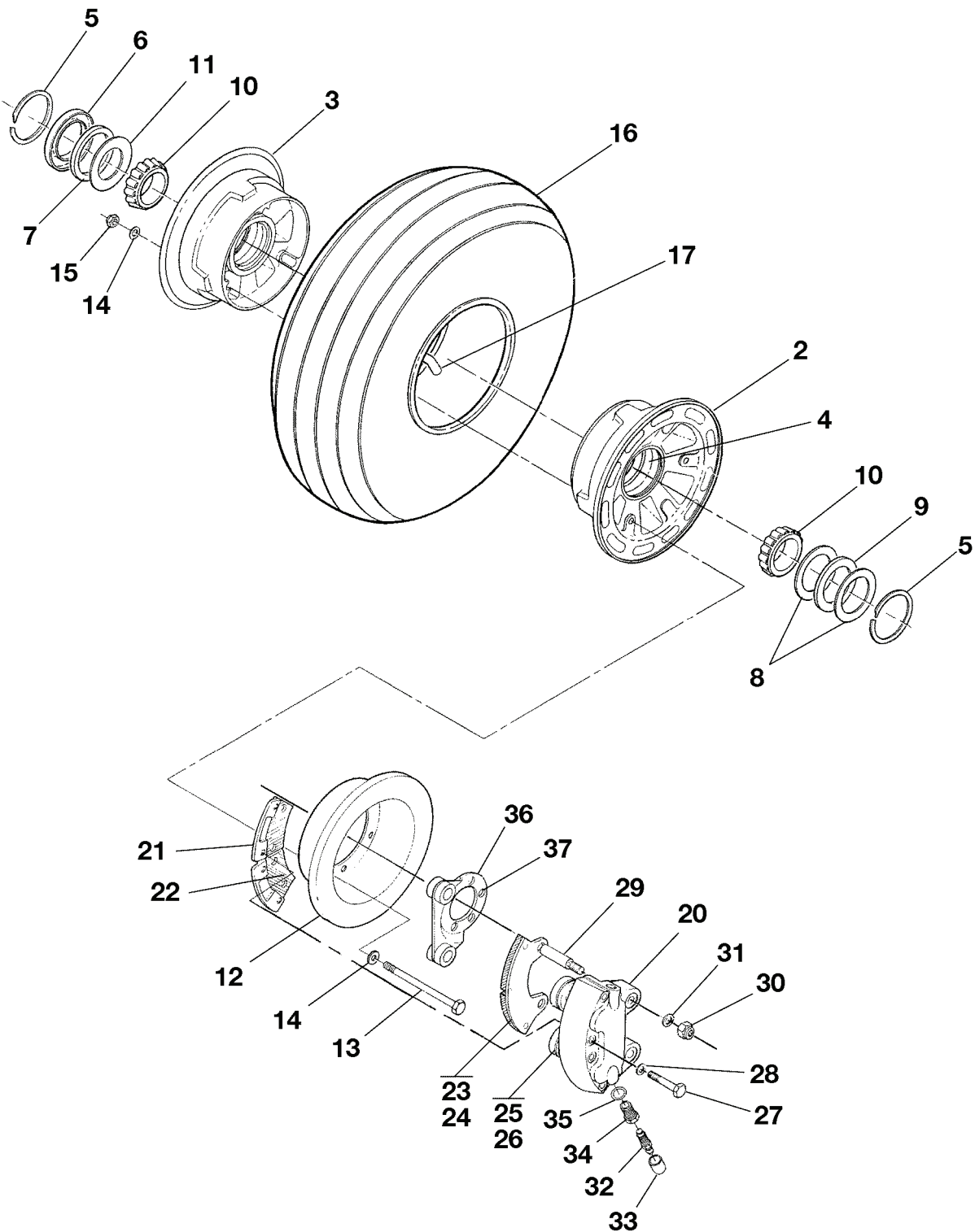
WHEEL AND BRAKE ASSEMBLY - MAIN LANDING GEAR FIGURE 01 (SHEET 1)
