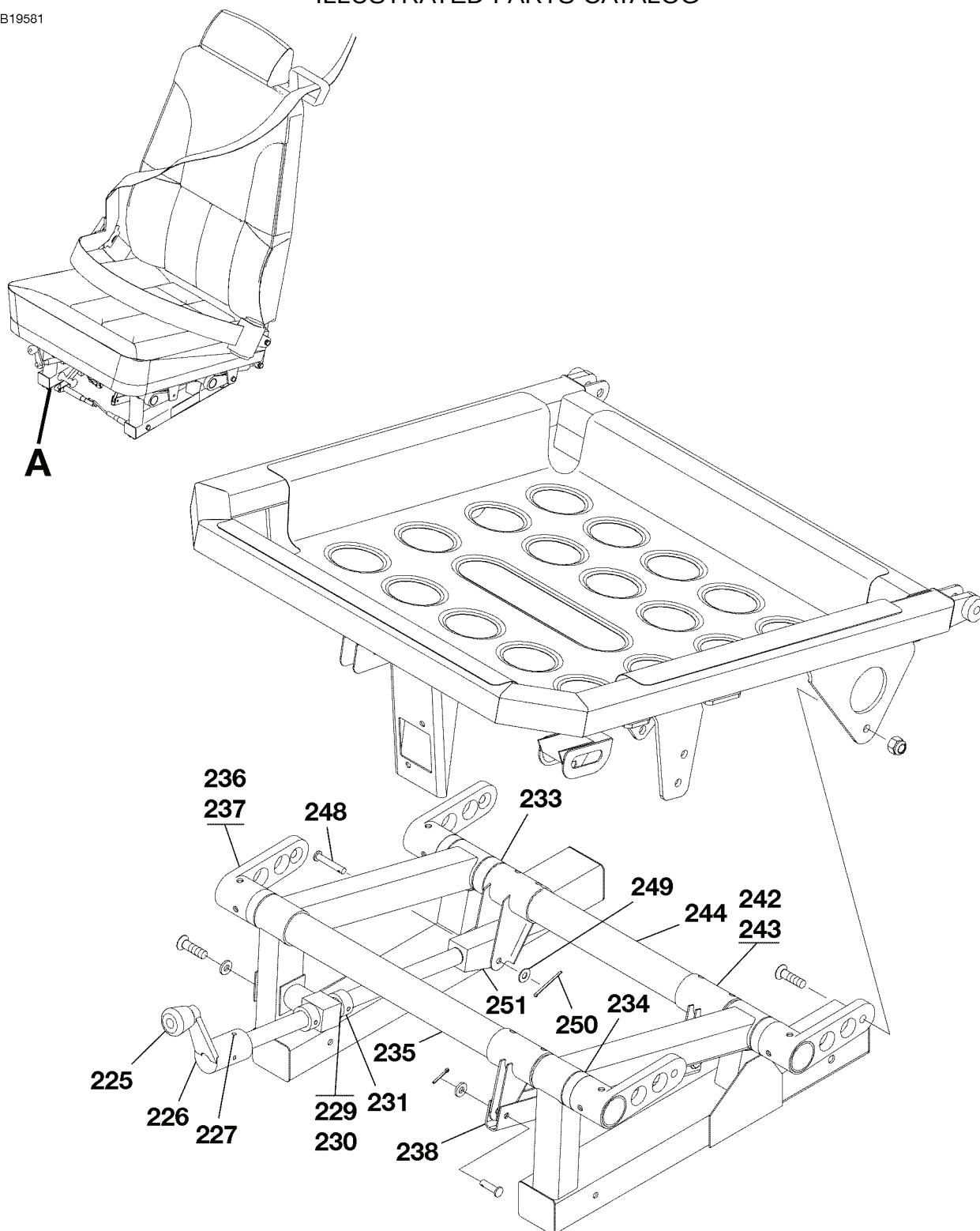
SEAT ASSEMBLY-PILOT AND COPILOT FIGURE 02A (SHEET 4)
