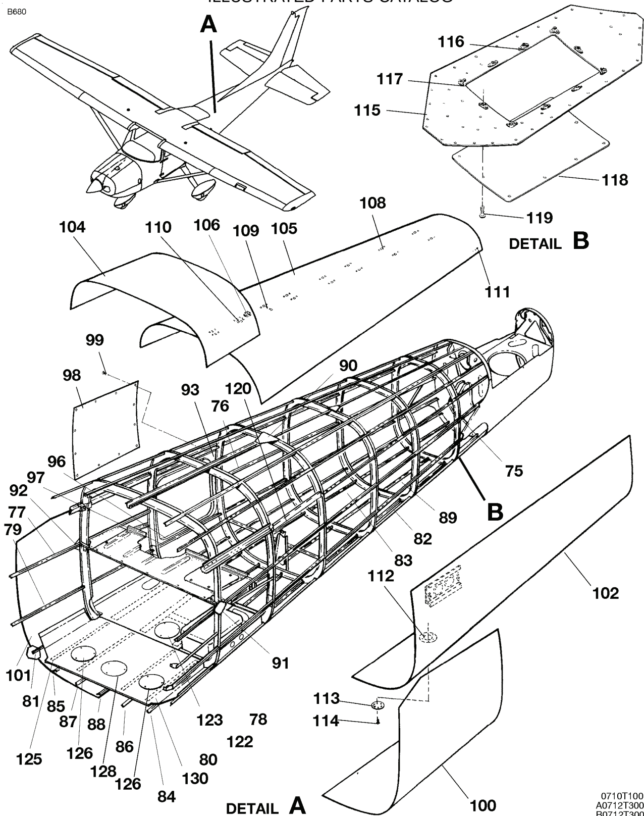
TAILCONE ASSEMBLY FIGURE 01 (SHEET 2)
