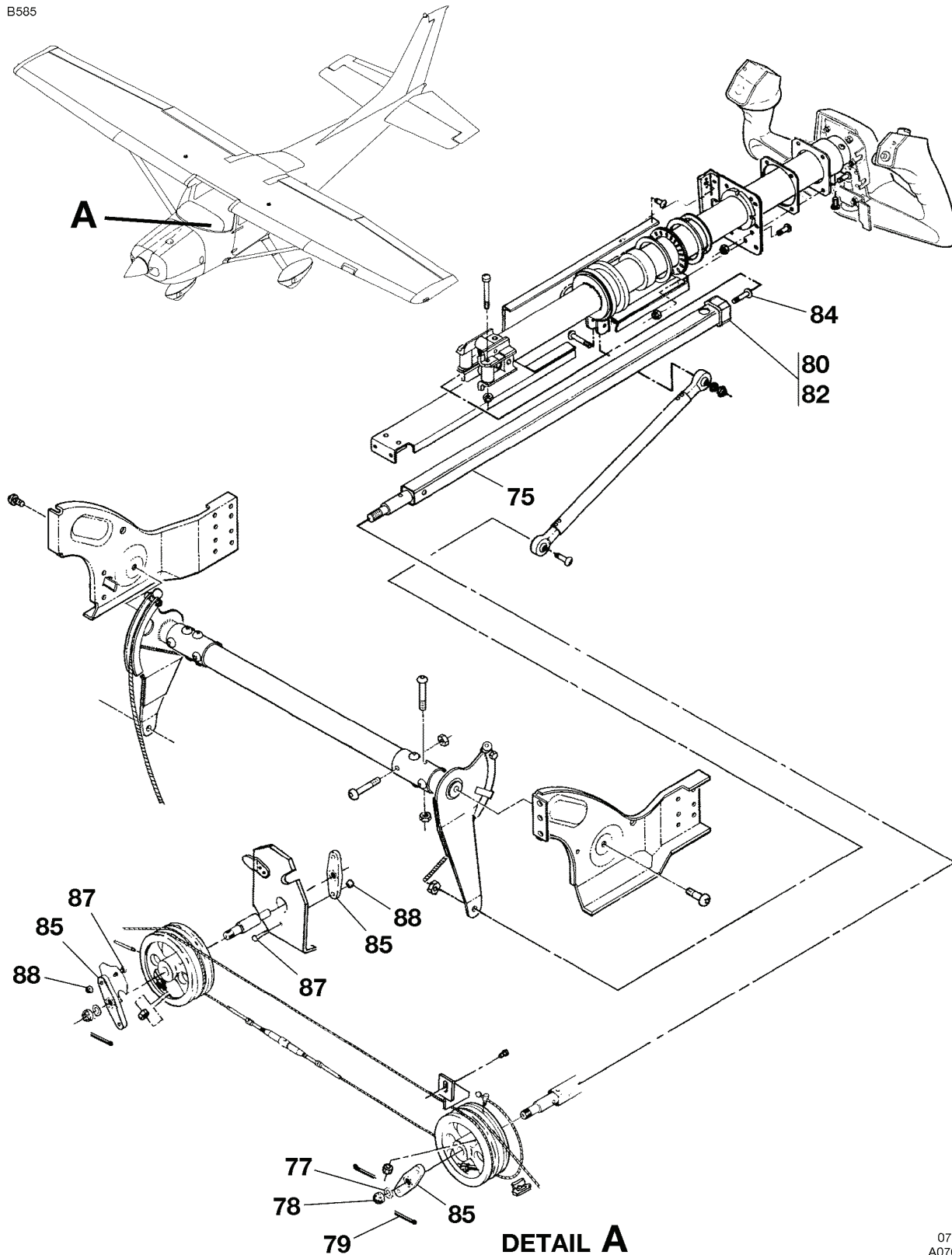
CONTROL COLUMN INSTALLATION FIGURE 01 (SHEET 2)
