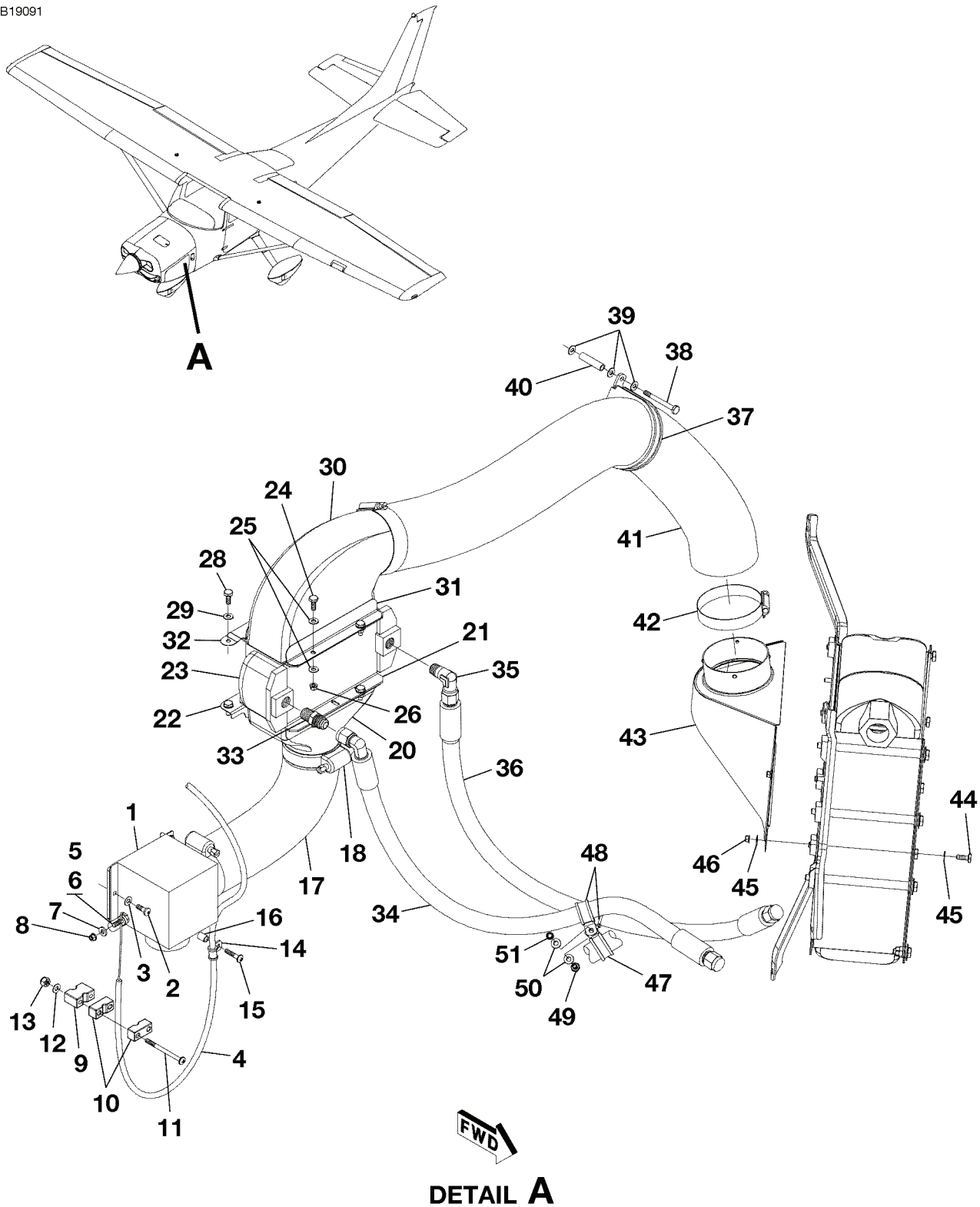
CABIN HEATING AND DEFROSTING INSTALLATION - J182T FIGURE 02 (SHEET 1)
