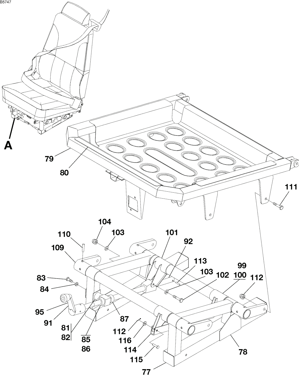
SEAT ASSEMBLY-PILOT AND COPILOT FIGURE 02 (SHEET 2)
