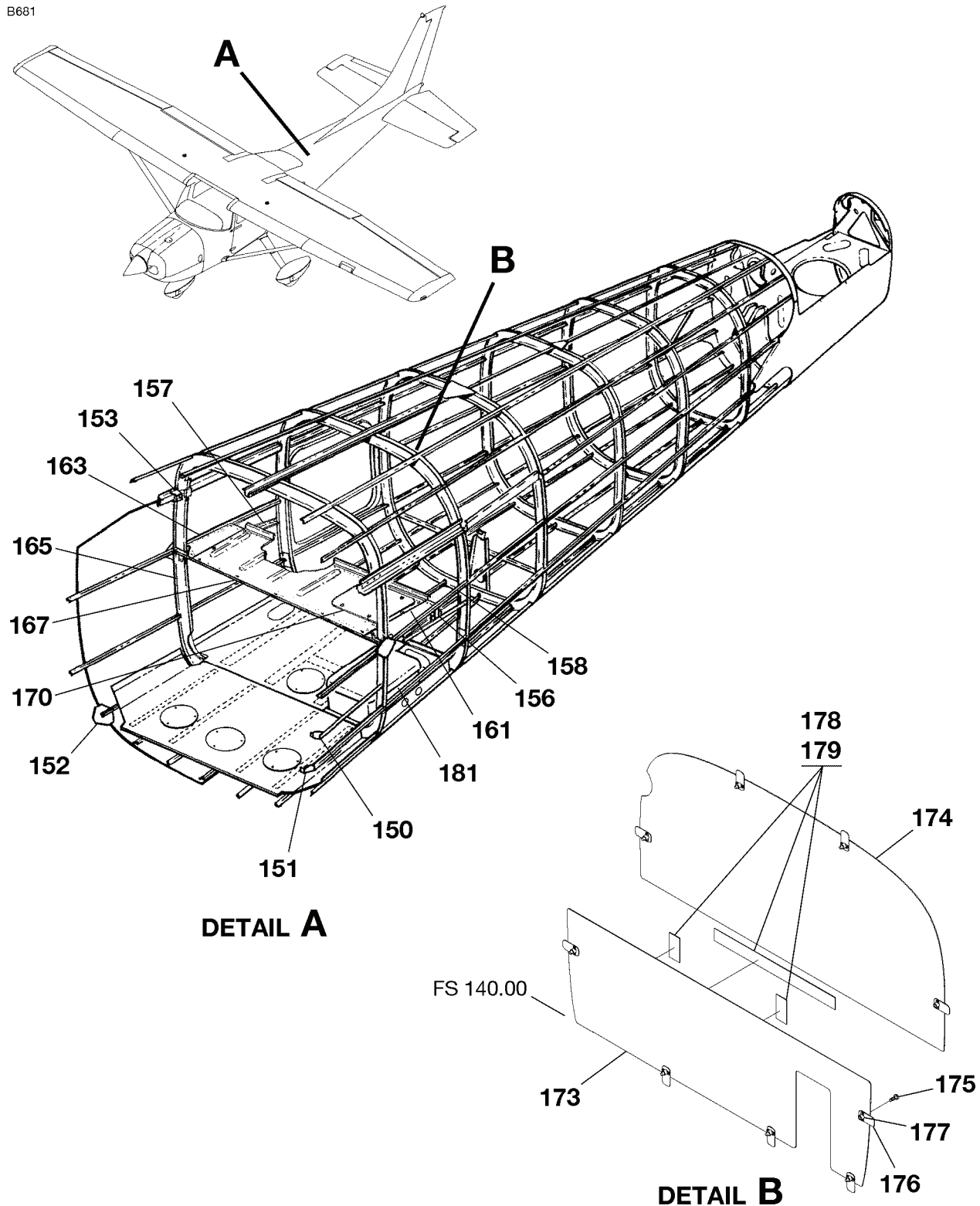
TAILCONE ASSEMBLY FIGURE 01 (SHEET 3)
