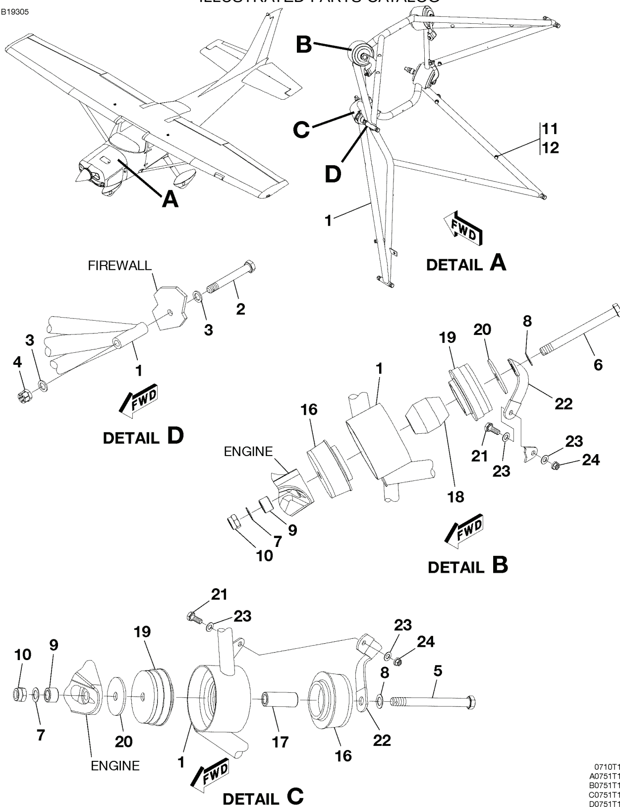
ENGINE MOUNT INSTALLATION - J182T FIGURE 02 (SHEET 1)
