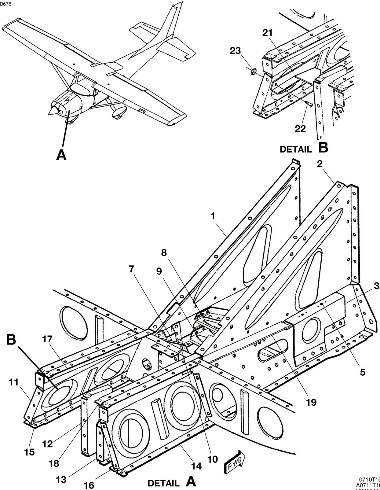
FRONT SECTION TUNNEL COMPONENTS FIGURE 04 (SHEET 1)
