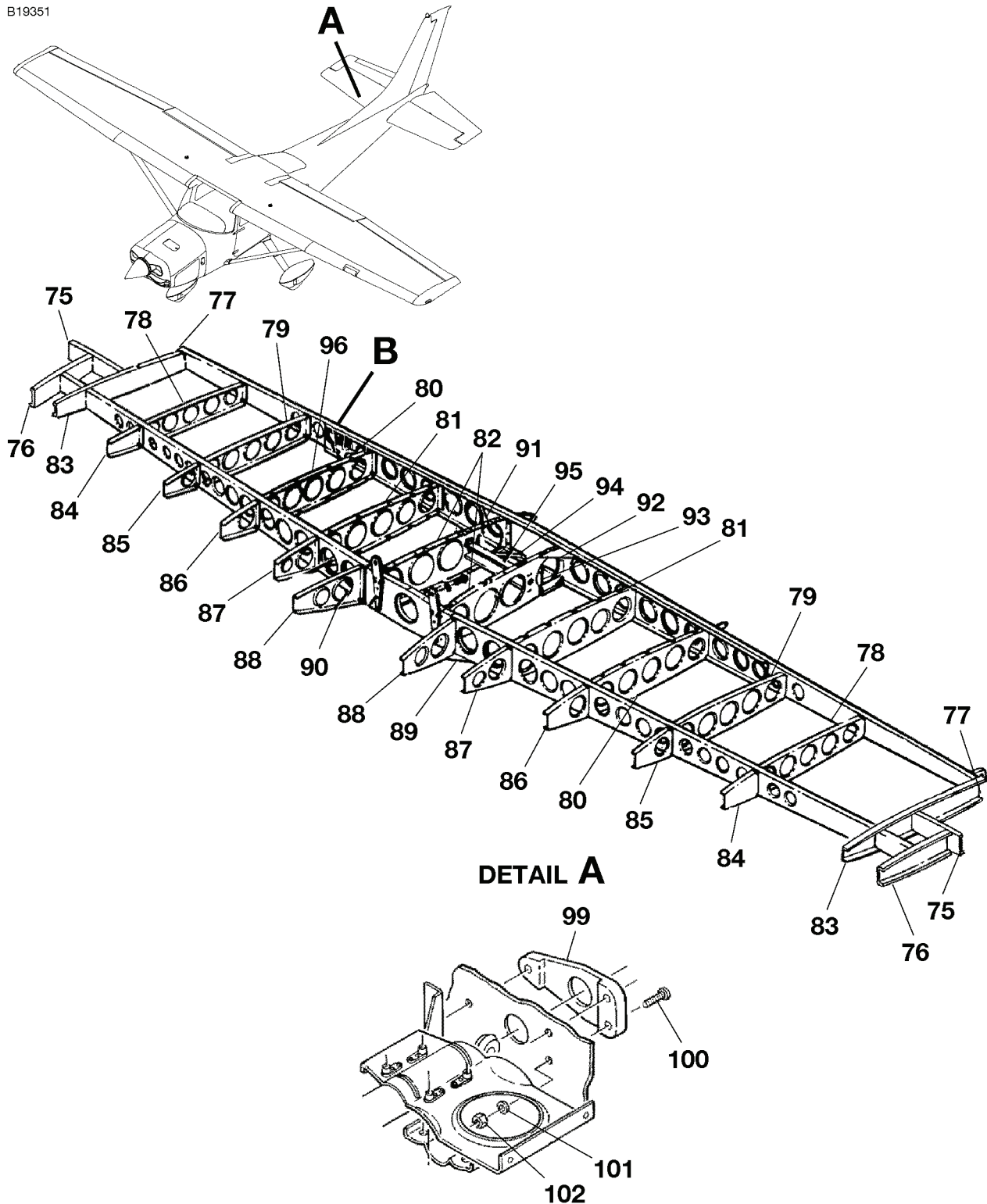
STABILIZER INSTALLATION FIGURE 01 (SHEET 2)
