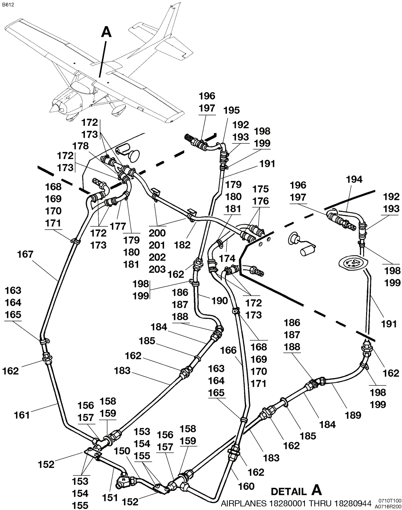
FUEL SYSTEM - 182 FIGURE 01 (SHEET 3)
