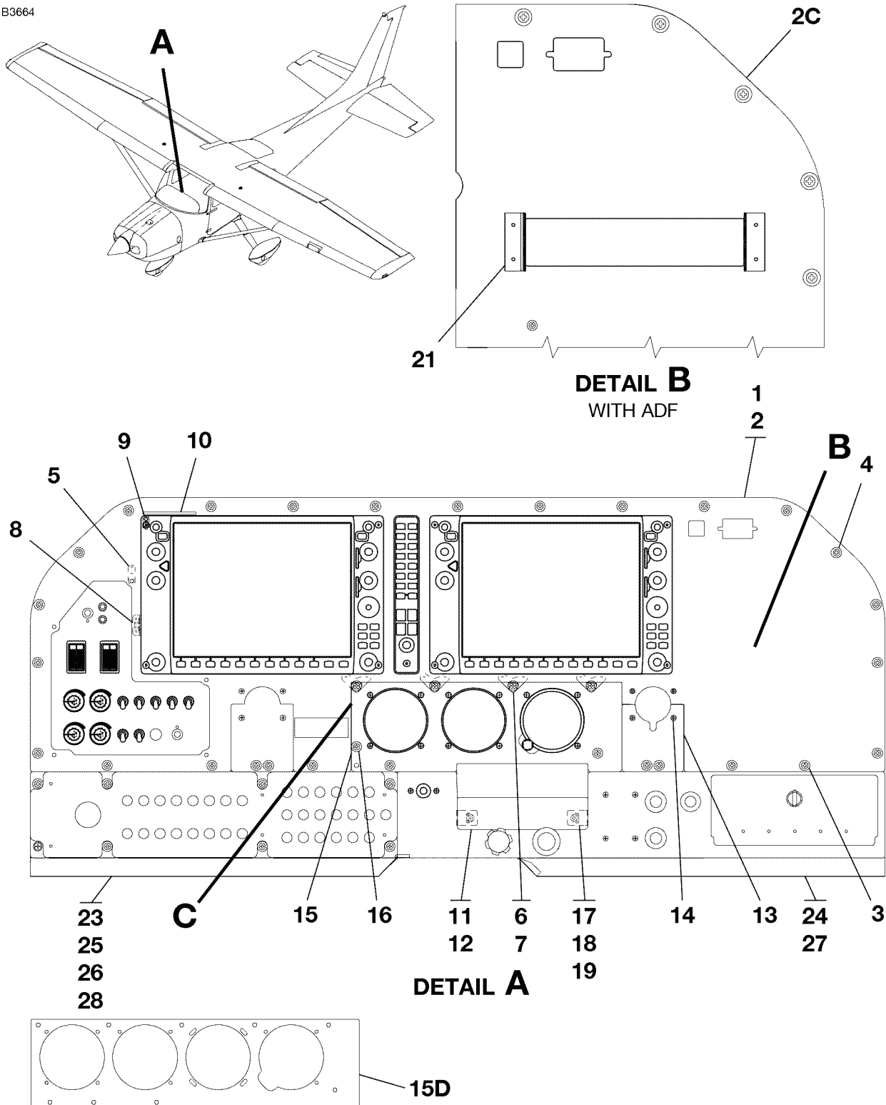
INSTRUMENT PANEL INSTALLATION - NAV III FIGURE 02 (SHEET 1)
