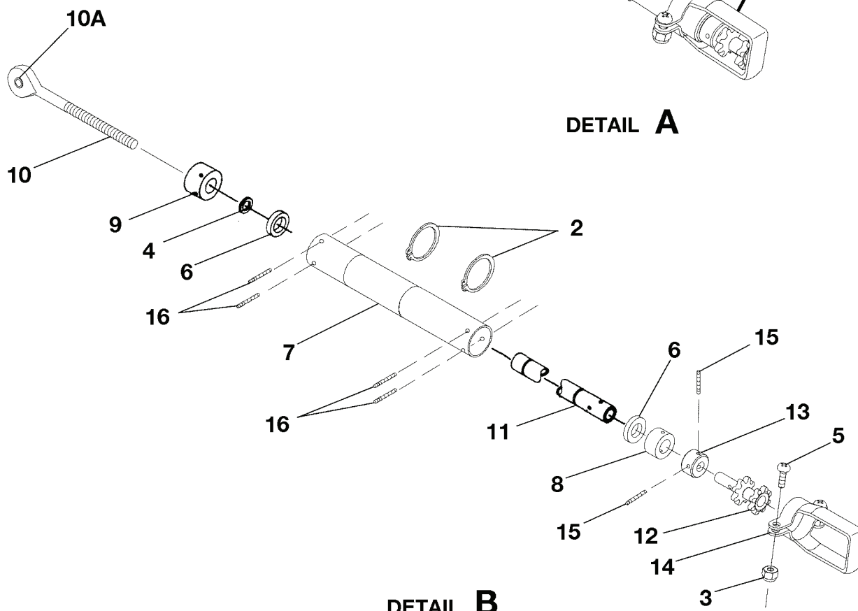
ELEVATOR TAB ACTUATOR ASSEMBLY - DUAL AXIS AUTO PILOT FIGURE 03 (SHEET 1)
