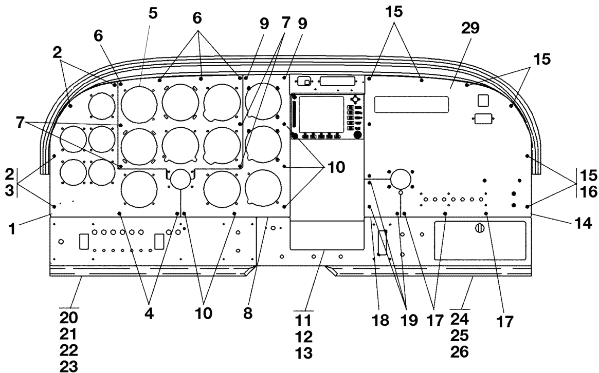
DETAIL A
