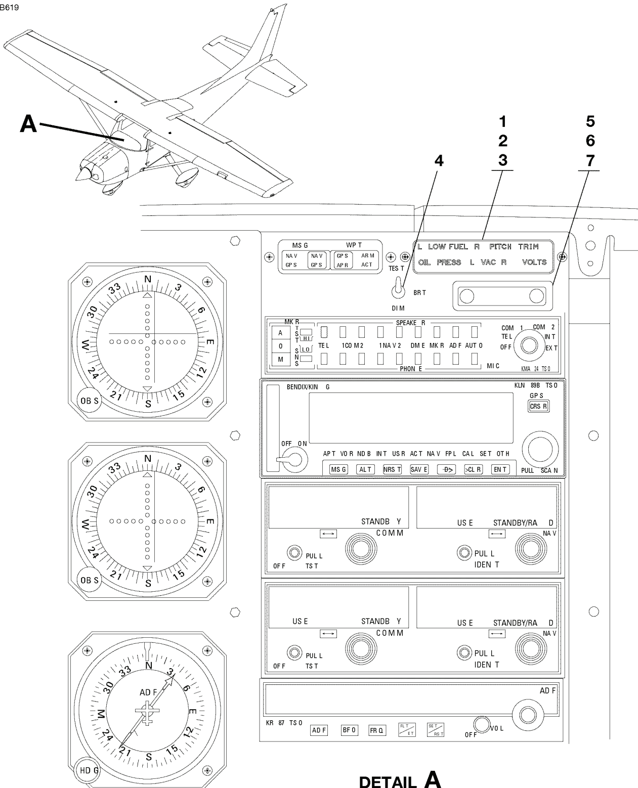
ANNUNCIATOR PANEL INSTALLATION - 182 FIGURE 01 (SHEET 1)
