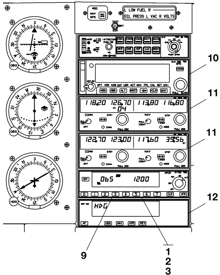
DETAIL A
