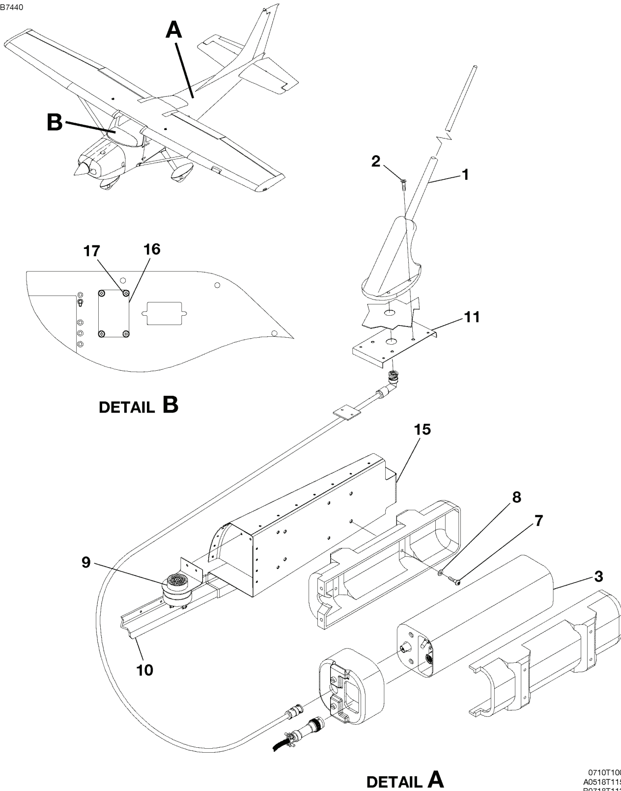
C406-N EMERGENCY LOCATOR TRANSMITTER FIGURE 04 (SHEET 1)
