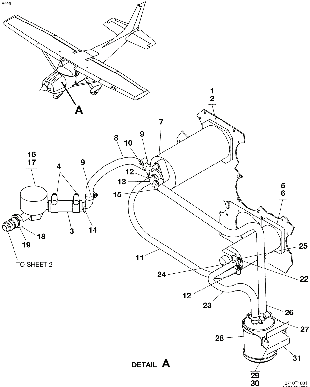
VACUUM SYSTEM - HORIZONTAL SITUATION INDICATOR (HSI) FIGURE 02 (SHEET 1)
