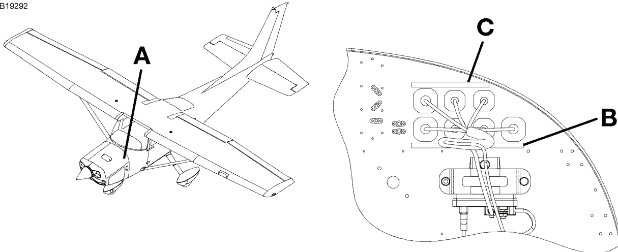
DETAIL A
