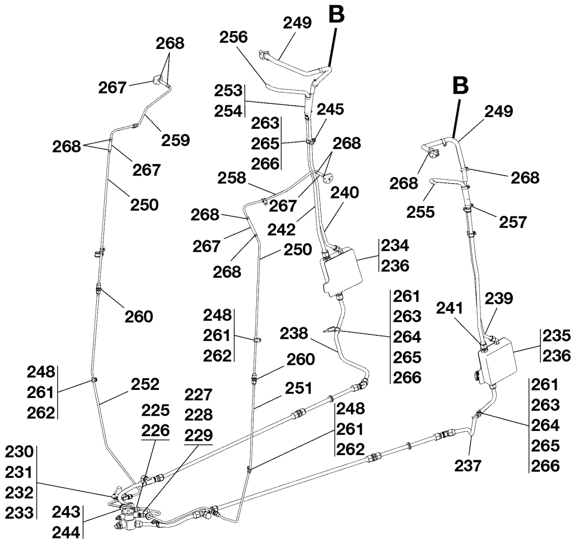
FUEL SYSTEM - 182/T182 FIGURE 02 (SHEET 4)
