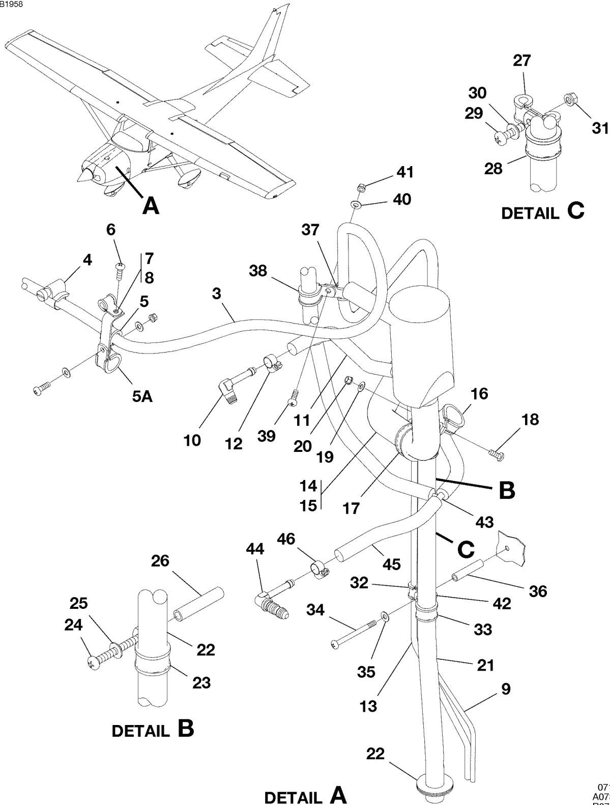
ENGINE DRAIN LINES INSTALLATION - T182 FIGURE 02 (SHEET 1)
