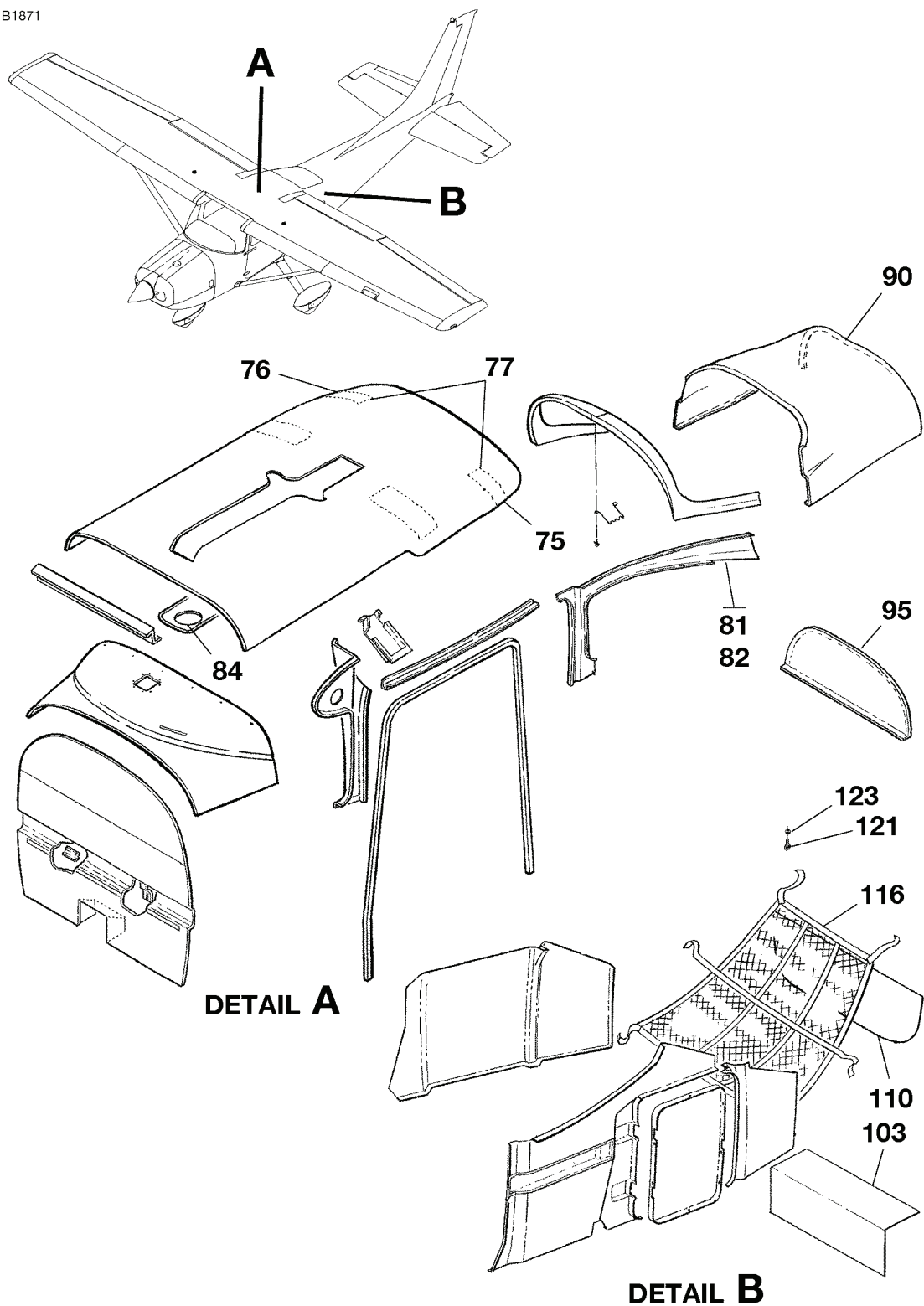
HEADLINER ASSEMBLIES FIGURE 02 (SHEET 2)
