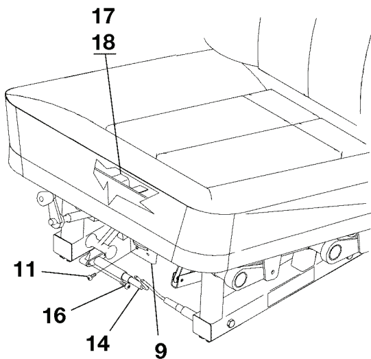
SEAT ASSEMBLY-PILOT AND COPILOT FIGURE 02 (SHEET 1)
