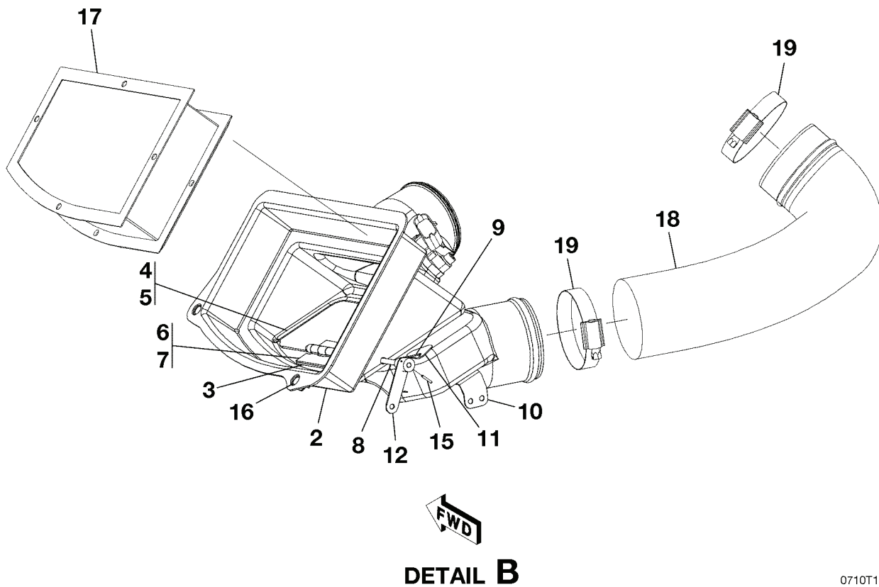
INDUCTION AIR INSTALLATION - J182T FIGURE 03 (SHEET 1)
