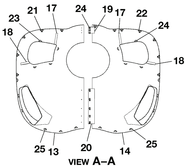
ENGINE COWL ASSEMBLY - J182T FIGURE 01A (SHEET 1)
