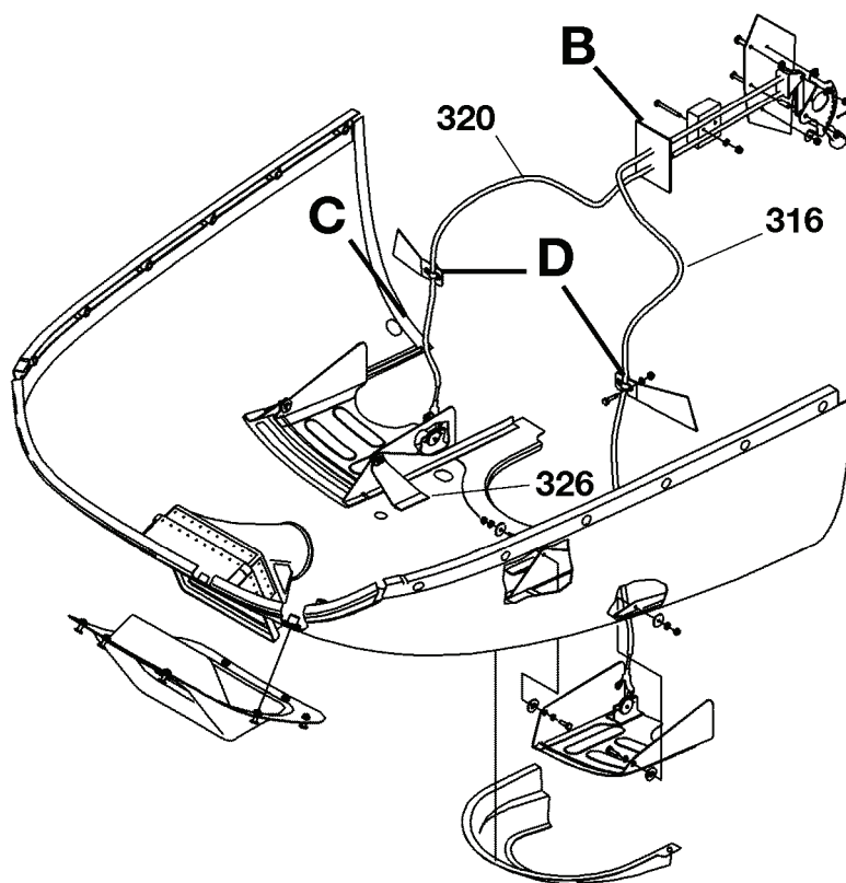
DETAIL A
