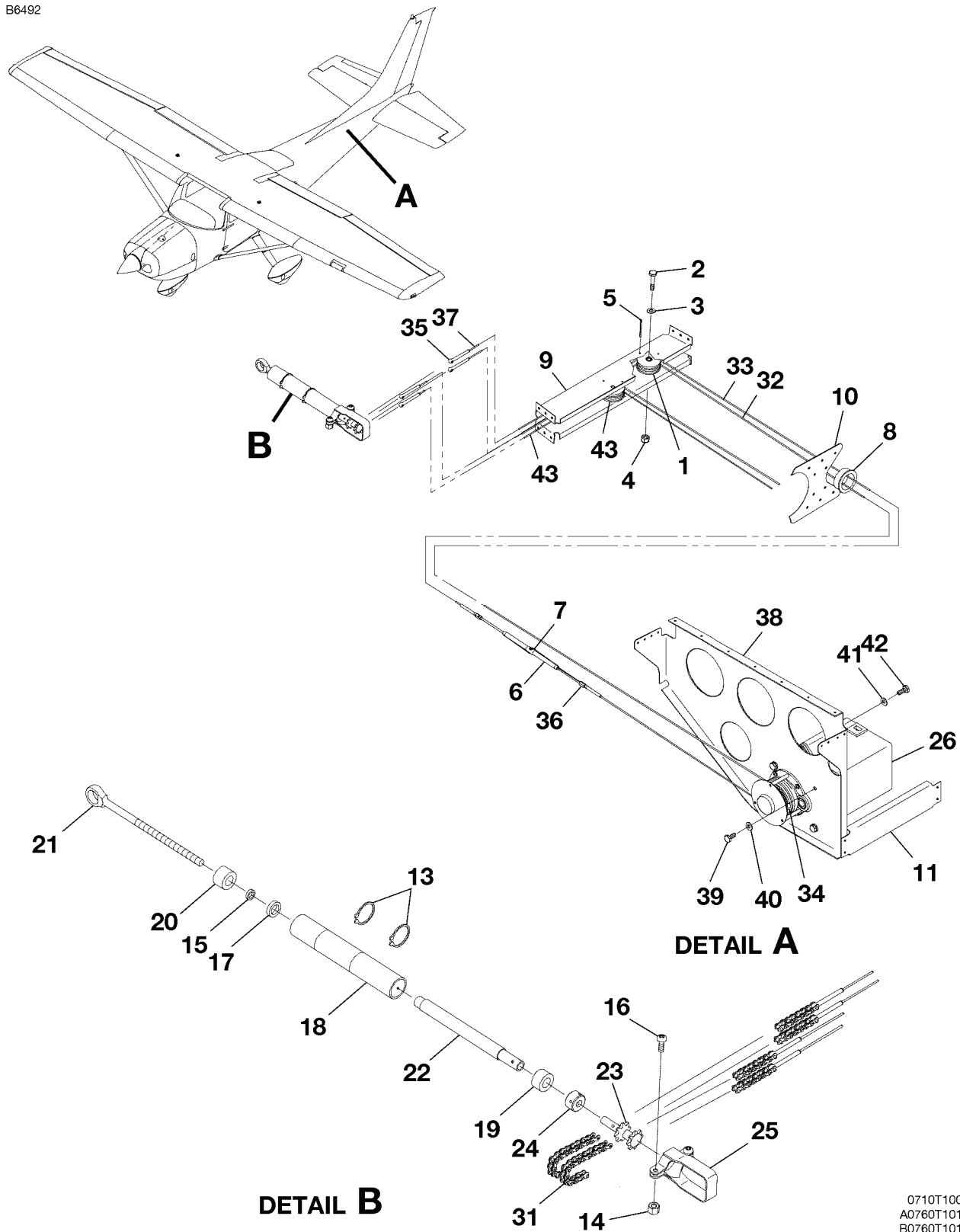
PITCH TRIM SERVO - NAV III FIGURE 05 (SHEET 1)
