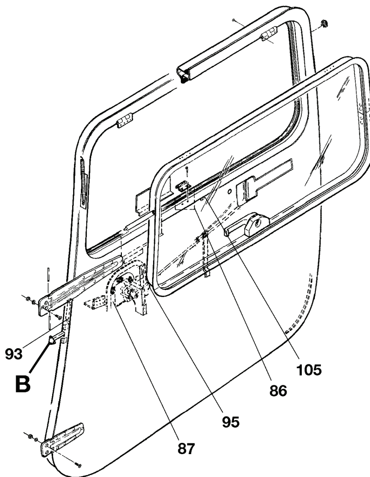
DETAIL A
