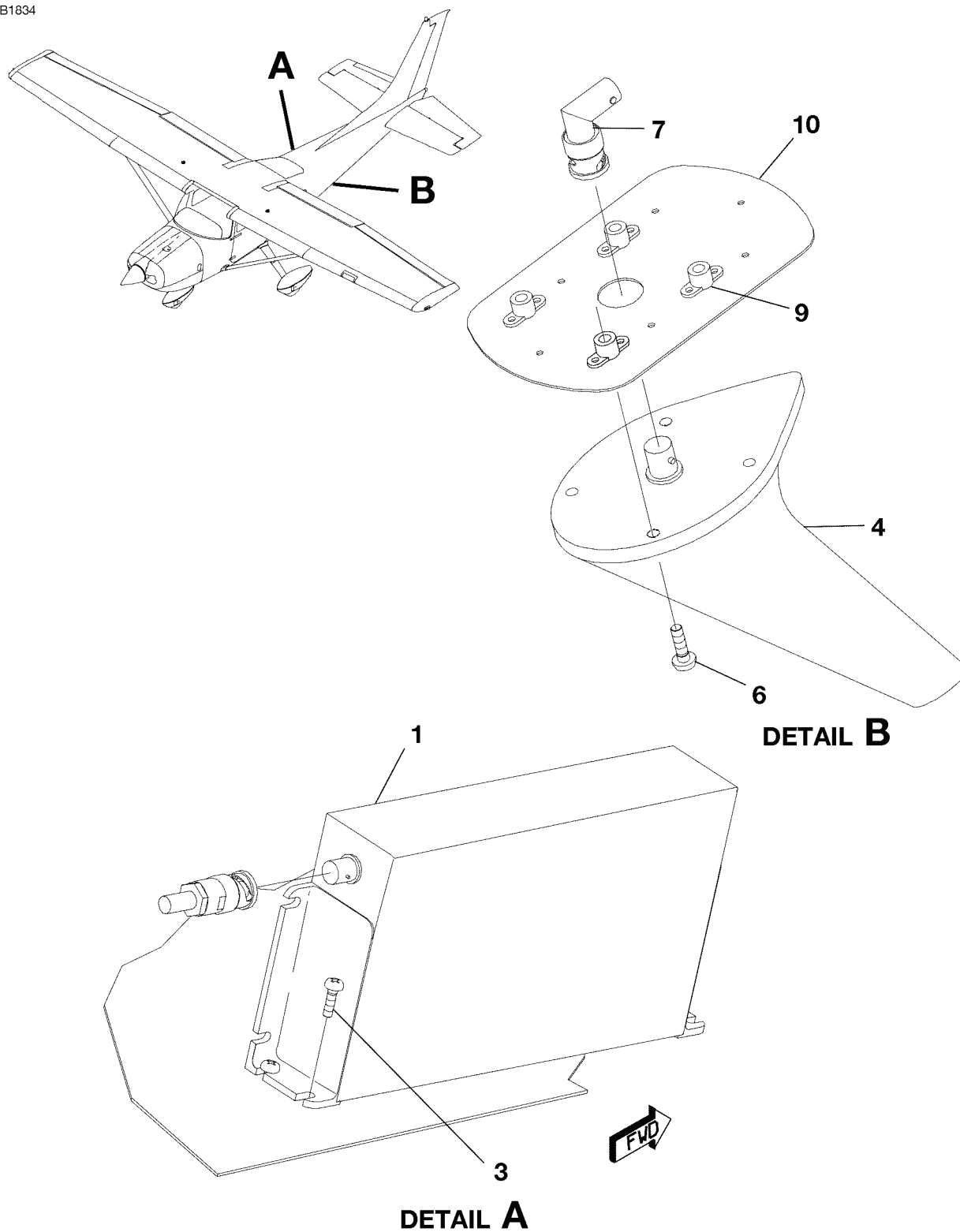
FIS RECEIVER AND ANTENNA INSTALLATION FIGURE 04 (SHEET 1)
