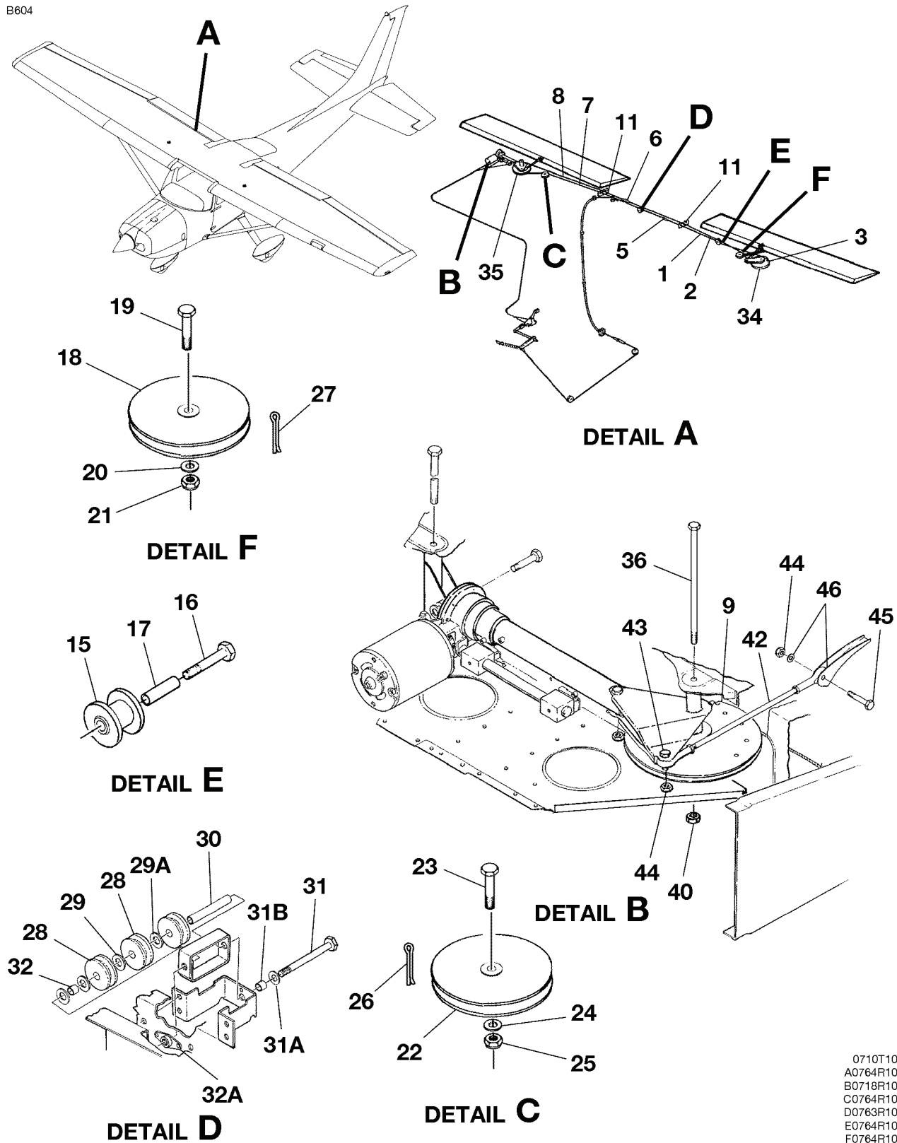
FLAP CONTROL SYSTEM - ELECTRIC FIGURE 01 (SHEET 1)
