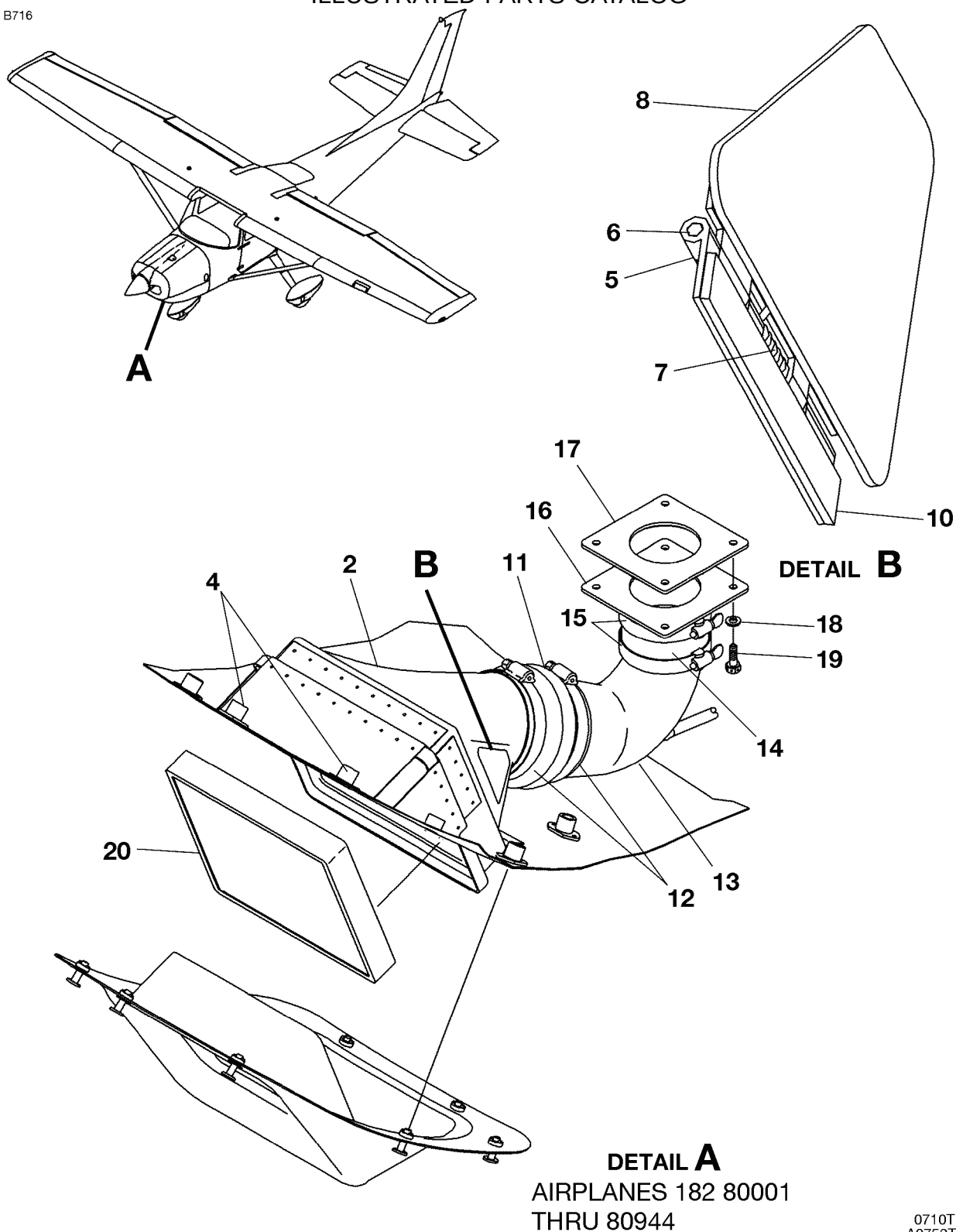
INDUCTION AIR INSTALLATION - 182 FIGURE 01 (SHEET 1)
