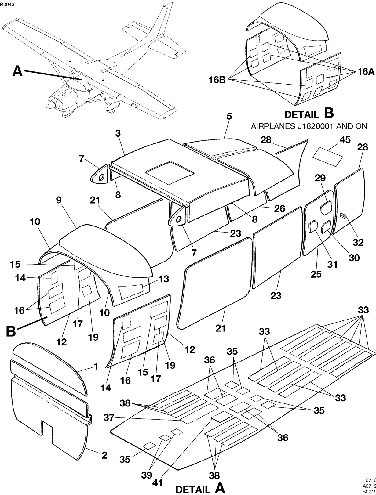
SOUNDPROOFING INSTALLATION - NAV III FIGURE 02 (SHEET 1)
