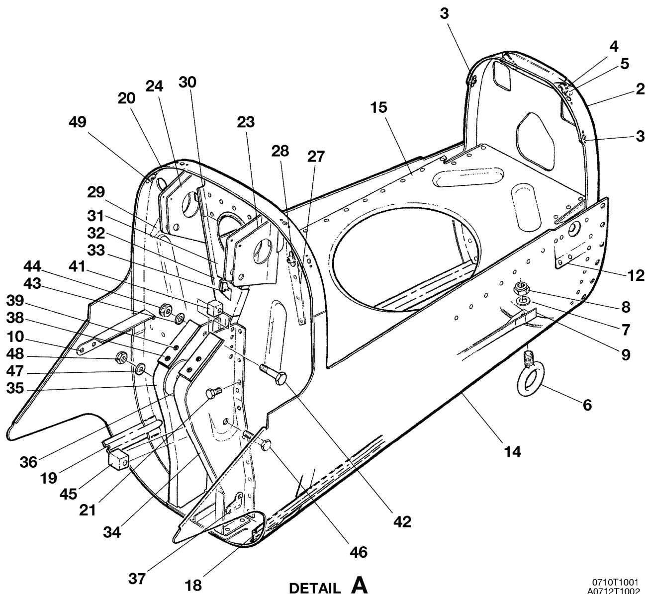
AFT TAILCONE ASSEMBLY - FS209.00 TO FS230.187 FIGURE 01 (SHEET 1)
