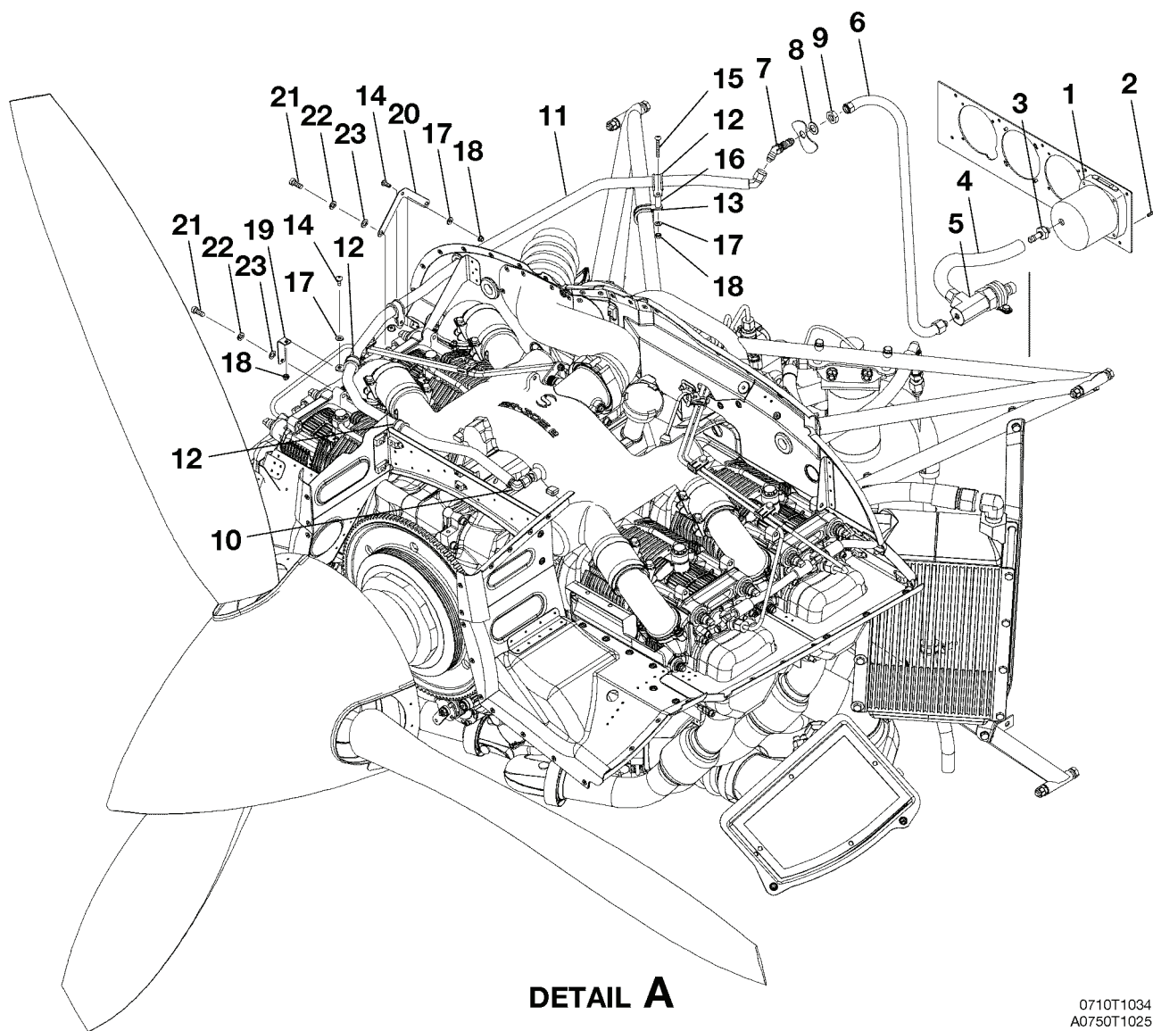
INDICATOR-MANIFOLD PRESSURE - J182T FIGURE 01A (SHEET 1)
