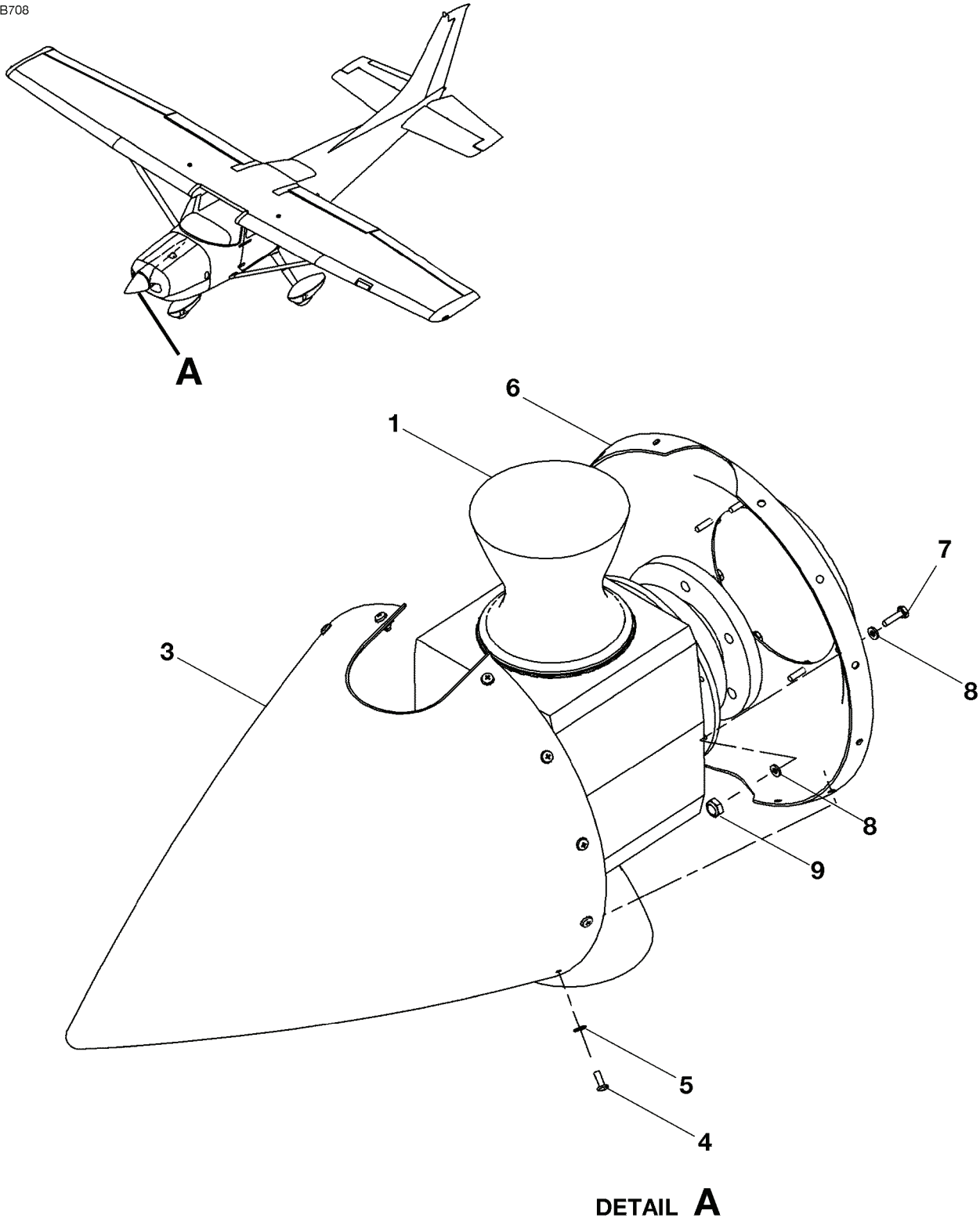
PROPELLER AND SPINNER INSTALLATION FIGURE 01 (SHEET 1)
