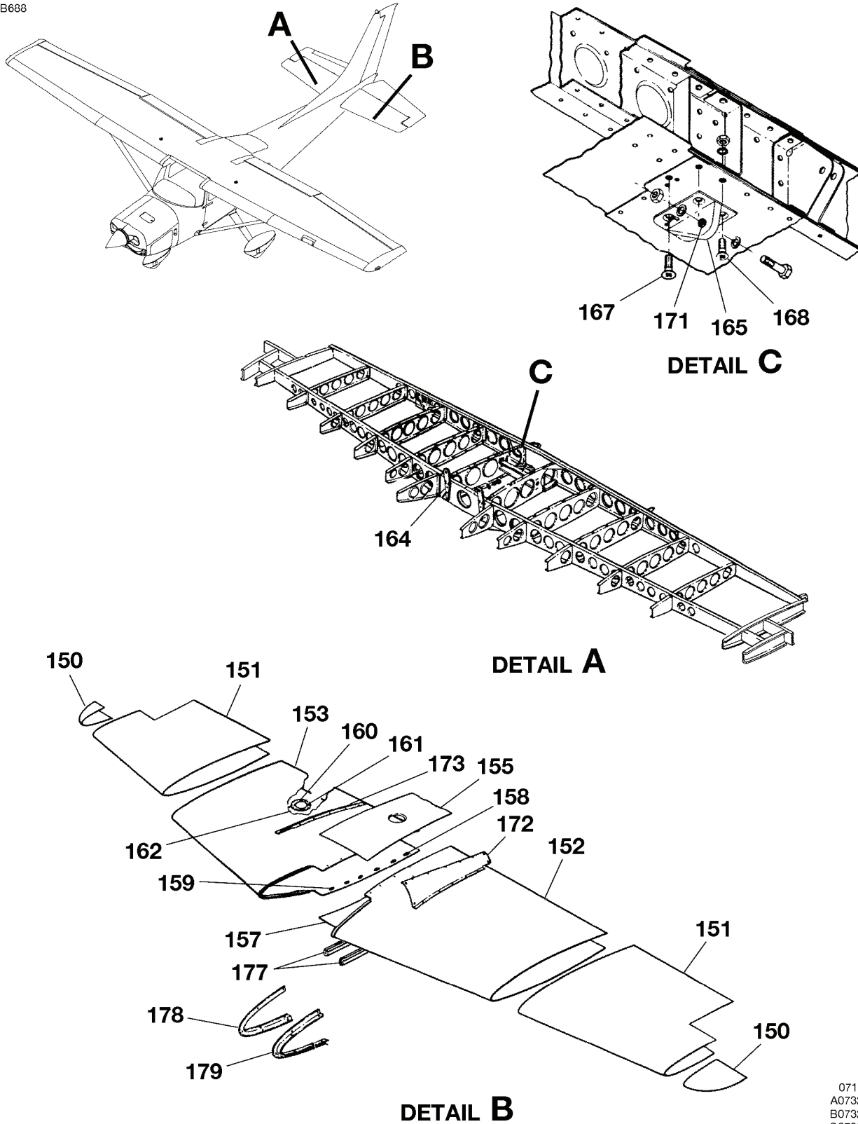
STABILIZER INSTALLATION FIGURE 01 (SHEET 3)
