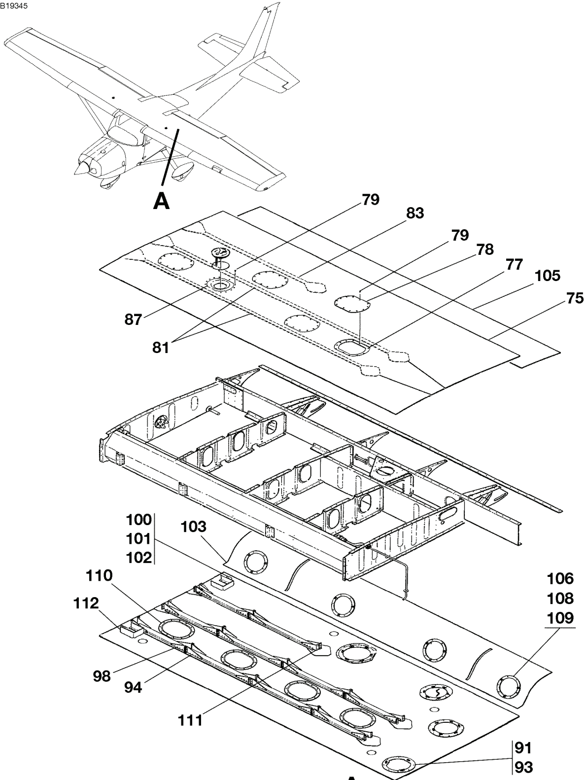
FUEL BAY STRUCTURE ASSEMBLY FIGURE 02 (SHEET 2)
