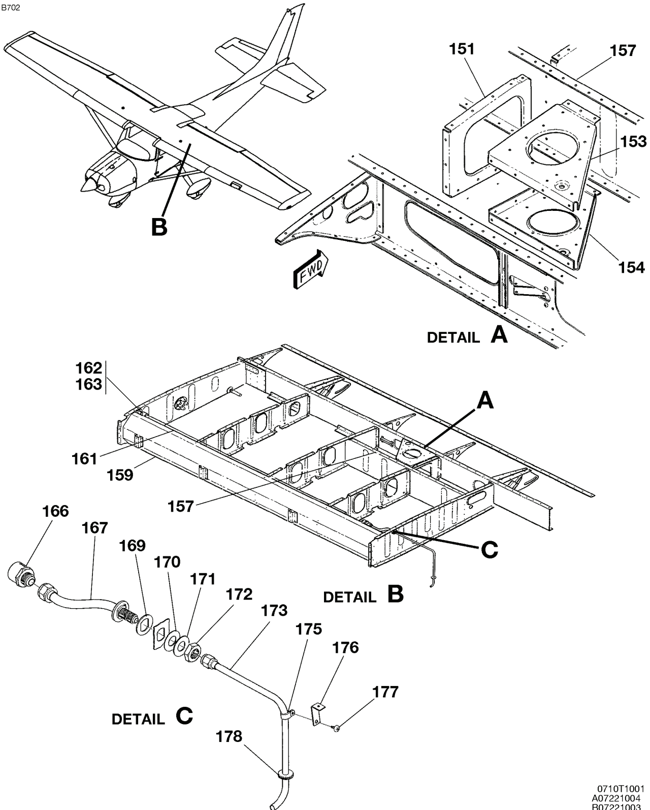
FUEL BAY STRUCTURE ASSEMBLY FIGURE 01 (SHEET 3)
