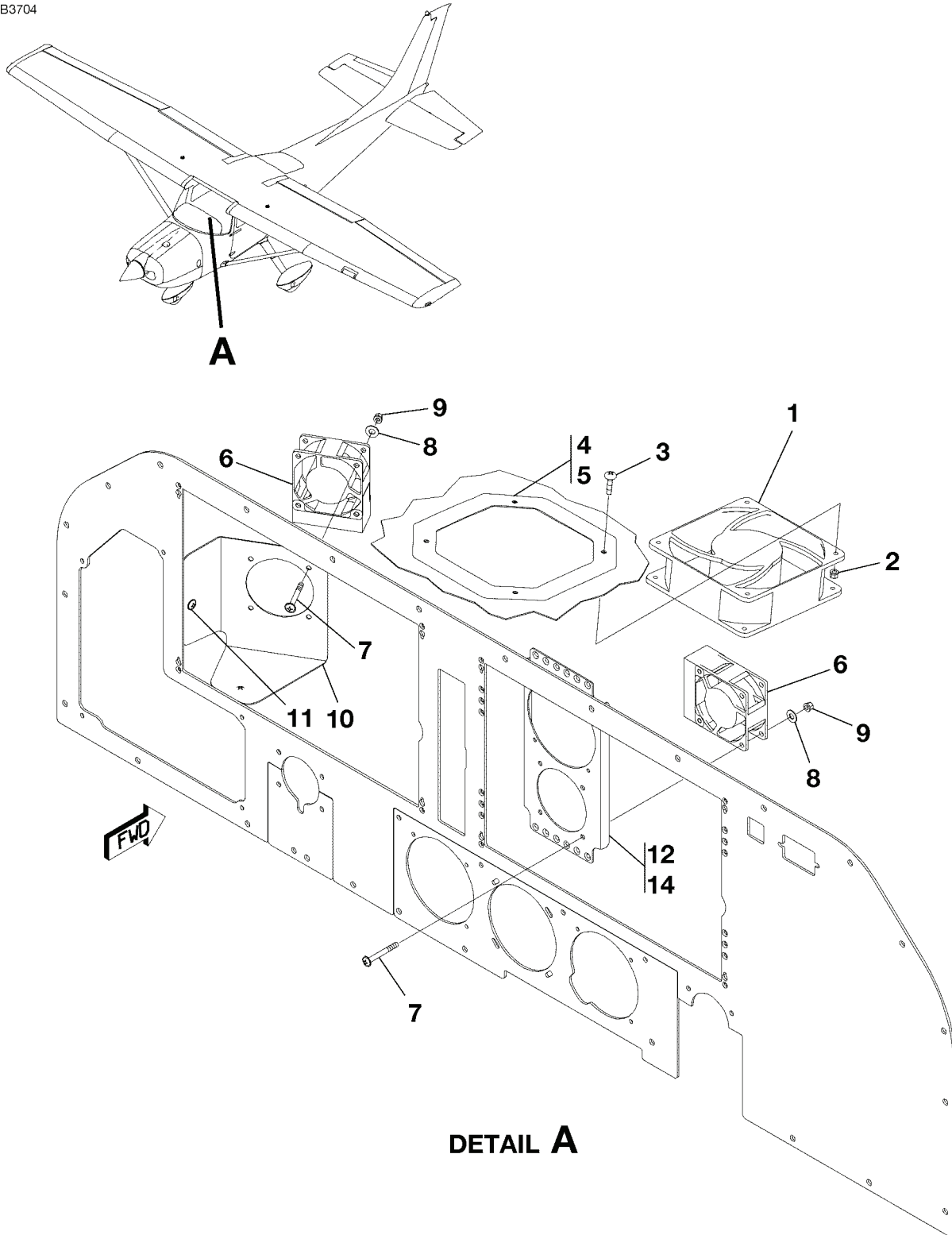
AVIONICS COOLING FAN INSTALLATION - GARMIN FIGURE 02 (SHEET 1)
