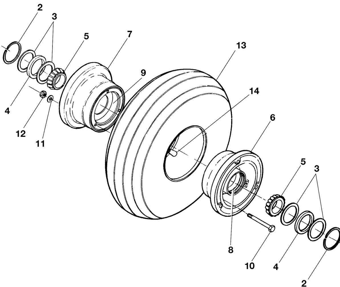
DETAIL A
