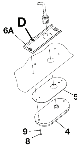
DETAIL C
