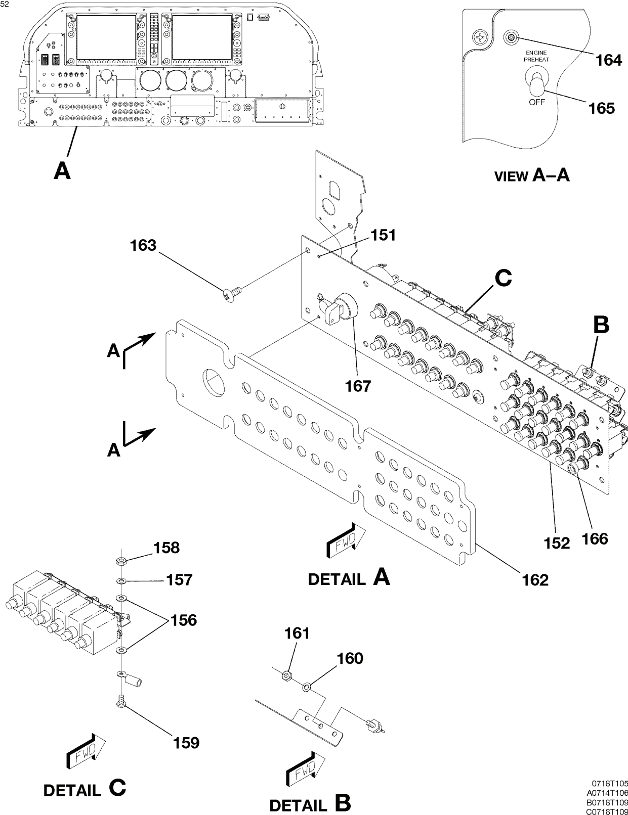
CIRCUIT BREAKER PANEL ASSEMBLY - NAV III FIGURE 01 (SHEET 3)
