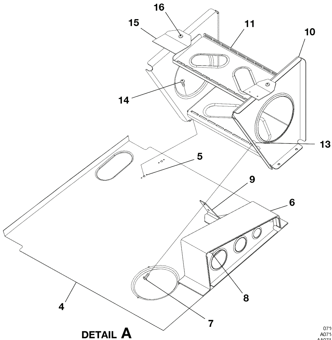
DETAIL A ATTITUDE HEADING AND REFERENCE SYSTEM - NAV III FIGURE 01 (SHEET 1)
