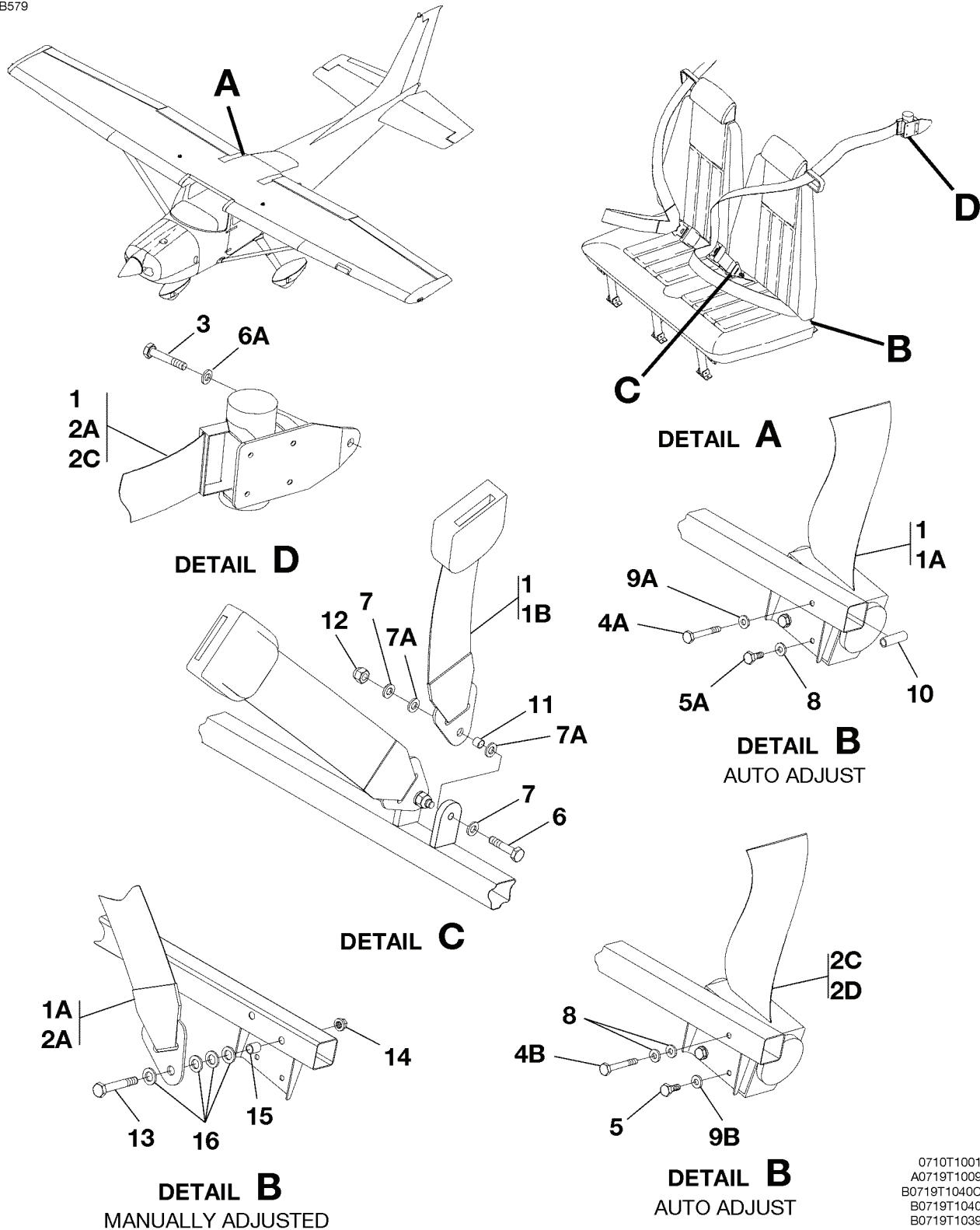
RESTRAINT SYSTEM-AFT BENCH SEAT FIGURE 01 (SHEET 1)
