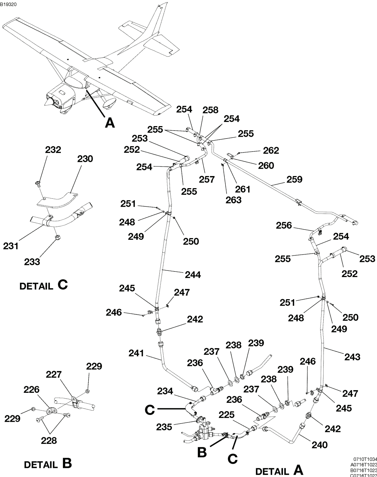
FUEL SYSTEM - J182T FIGURE 03 (SHEET 4)
