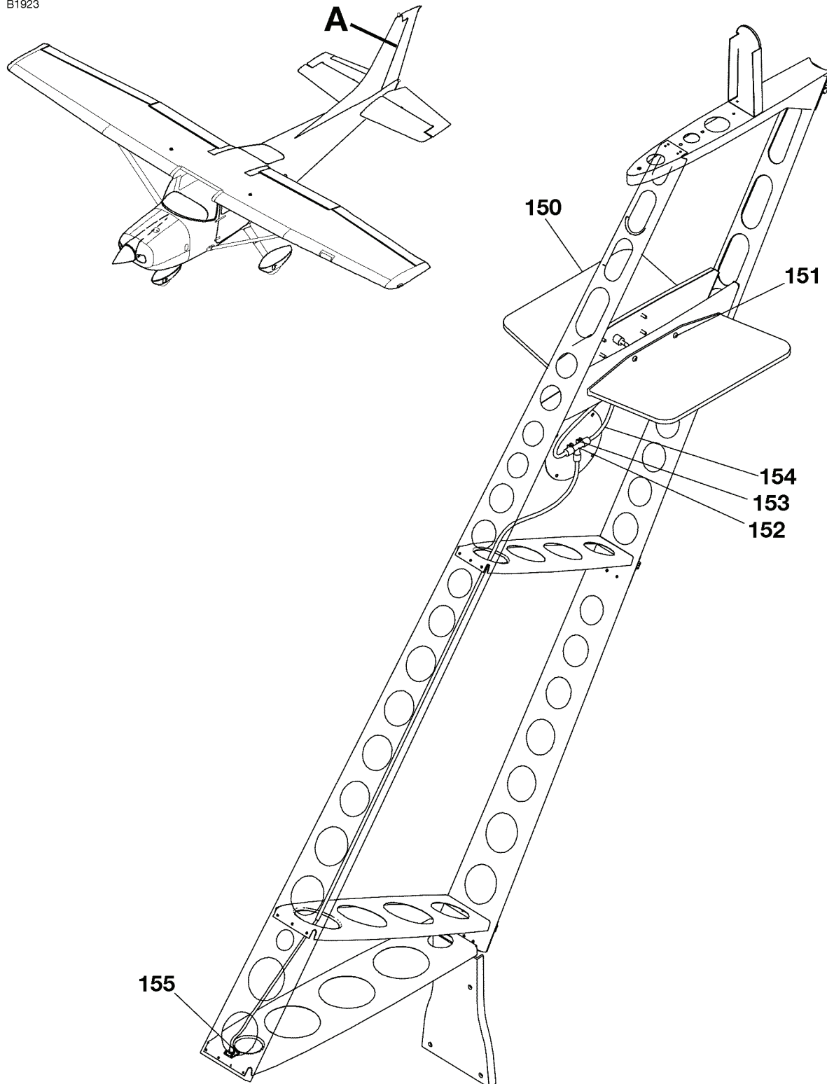
VHF NAVIGATION SYSTEM - BASIC FIGURE 01 (SHEET 3)
