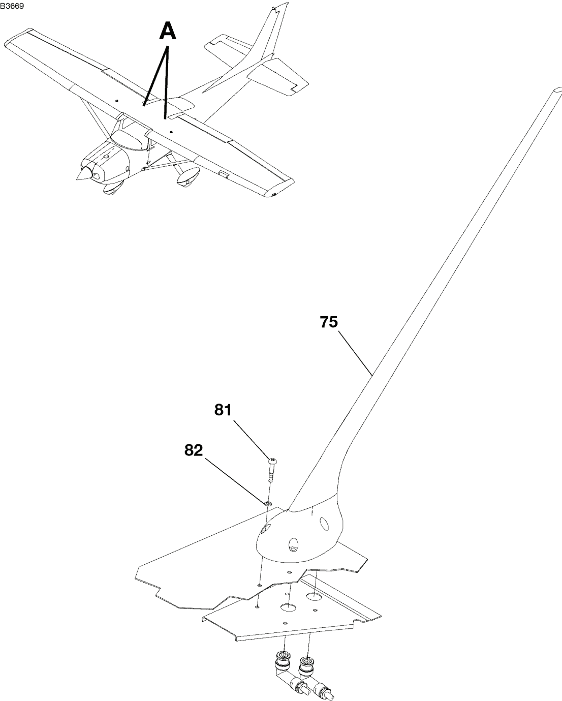
DETAIL A
