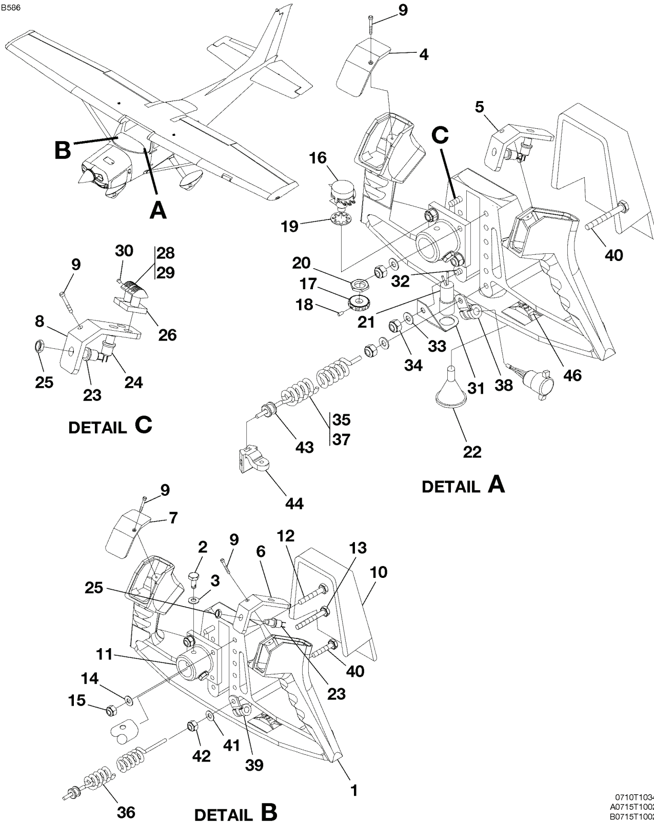
CONTROL WHEEL AND SWITCHES INSTALLATION FIGURE 02 (SHEET 1)
