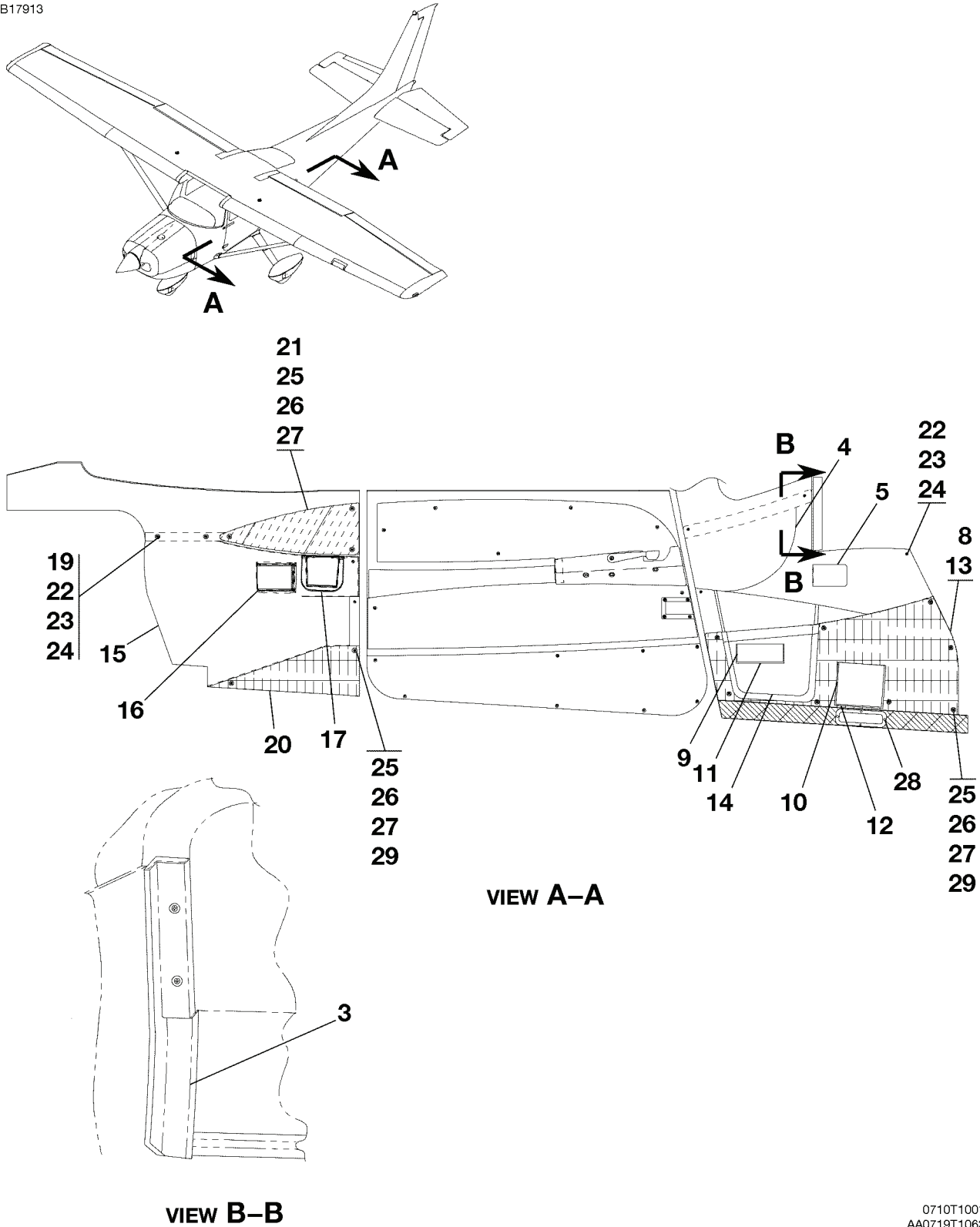
CABIN TRIM - SIDEWALLS FIGURE 01B (SHEET 1)
